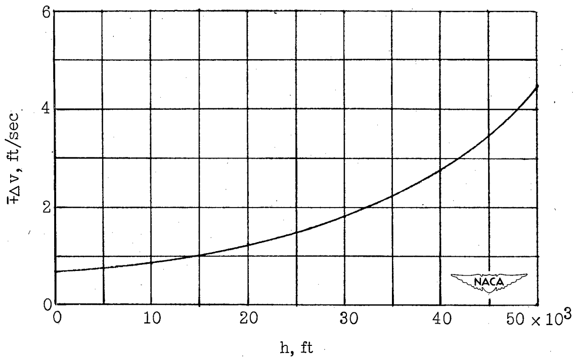
Figure 12.- Error in vertical velocity due to error of \pm 0.01 inch of water per second in time rate of change of static pressure.
