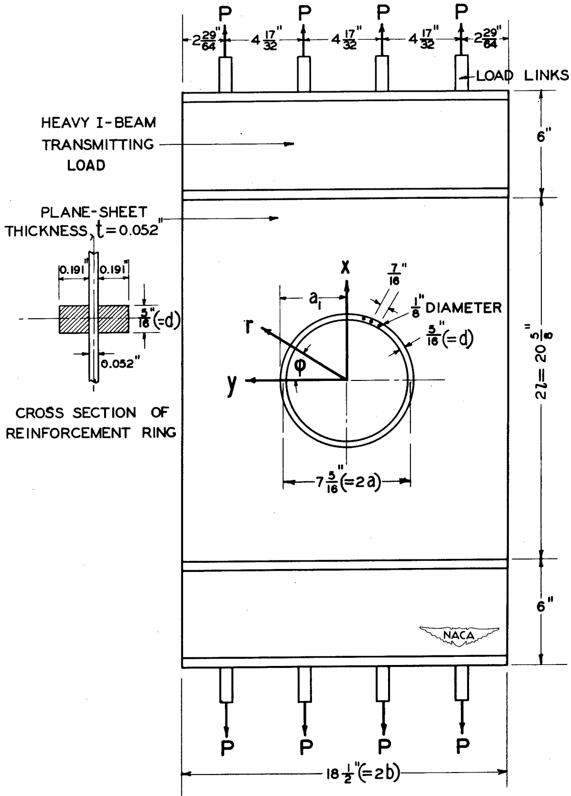
Figure 3.- Experimental setup.
