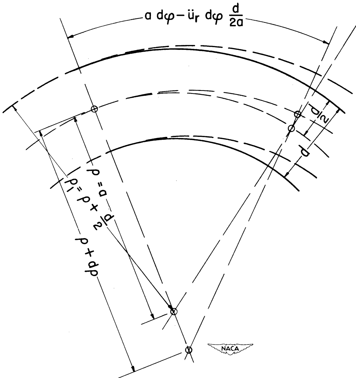
Figure 8.- Contribution of curvature of cutout ring to extension at outer
