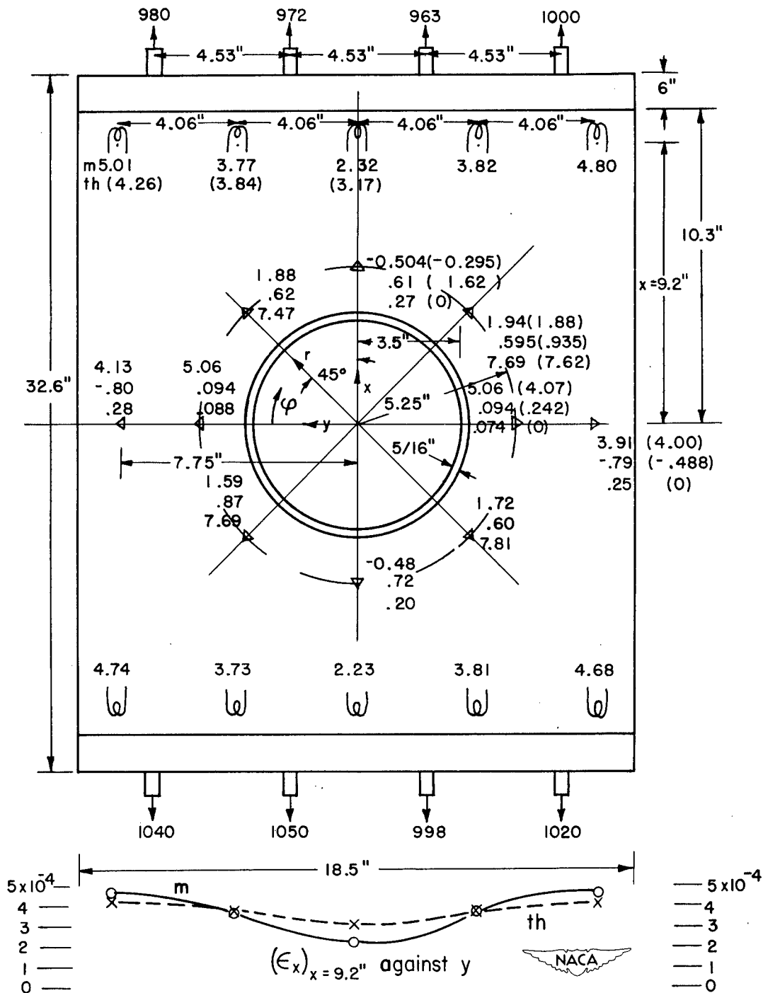
Figure 7.- Strain measurements on plane sheet with reinforced cutout. Total load, 4020 pounds; rosette, \Delta ; simple strain gage, \bigcirc ; values in parentheses are corresponding theoretical values for reinforced cutout but for an infinite sheet (see appendix G). For each rosette, the top, middle, and bottom values are, respectively, normal transverse, normal radial, and shear strain times 10^4 . For each simple gage, values given are those of axial strains \epsilon_x \times 10^4 .
