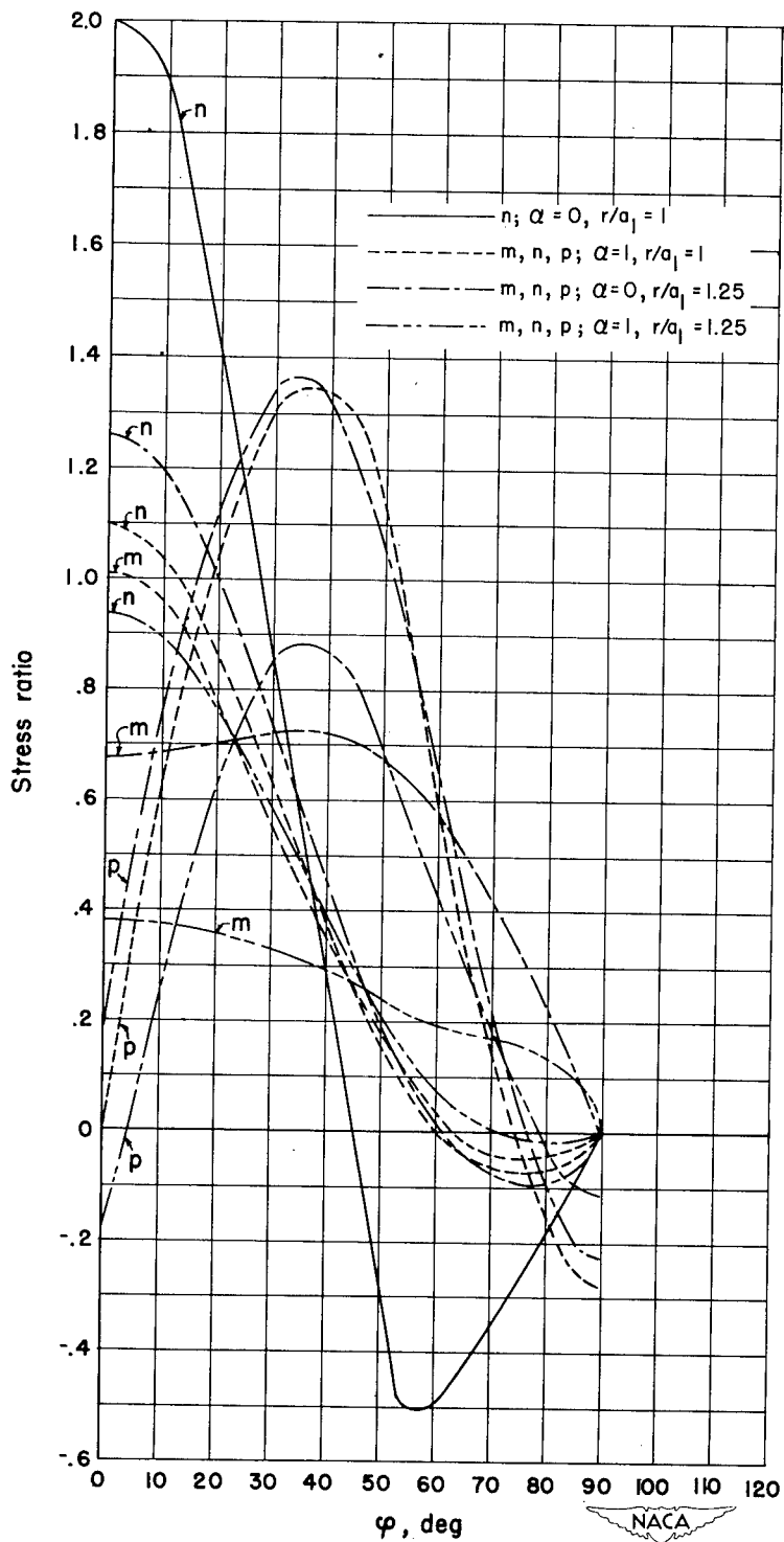
Figure 2.- Total-stress distribution in sheet produced by pure bending.
