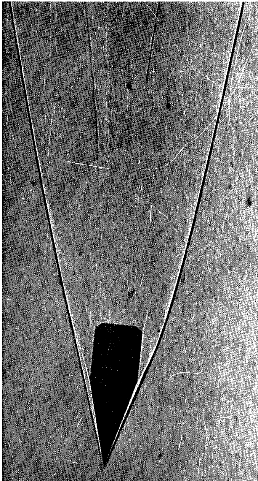
(a) 30° cone, Mach number 6.8.
