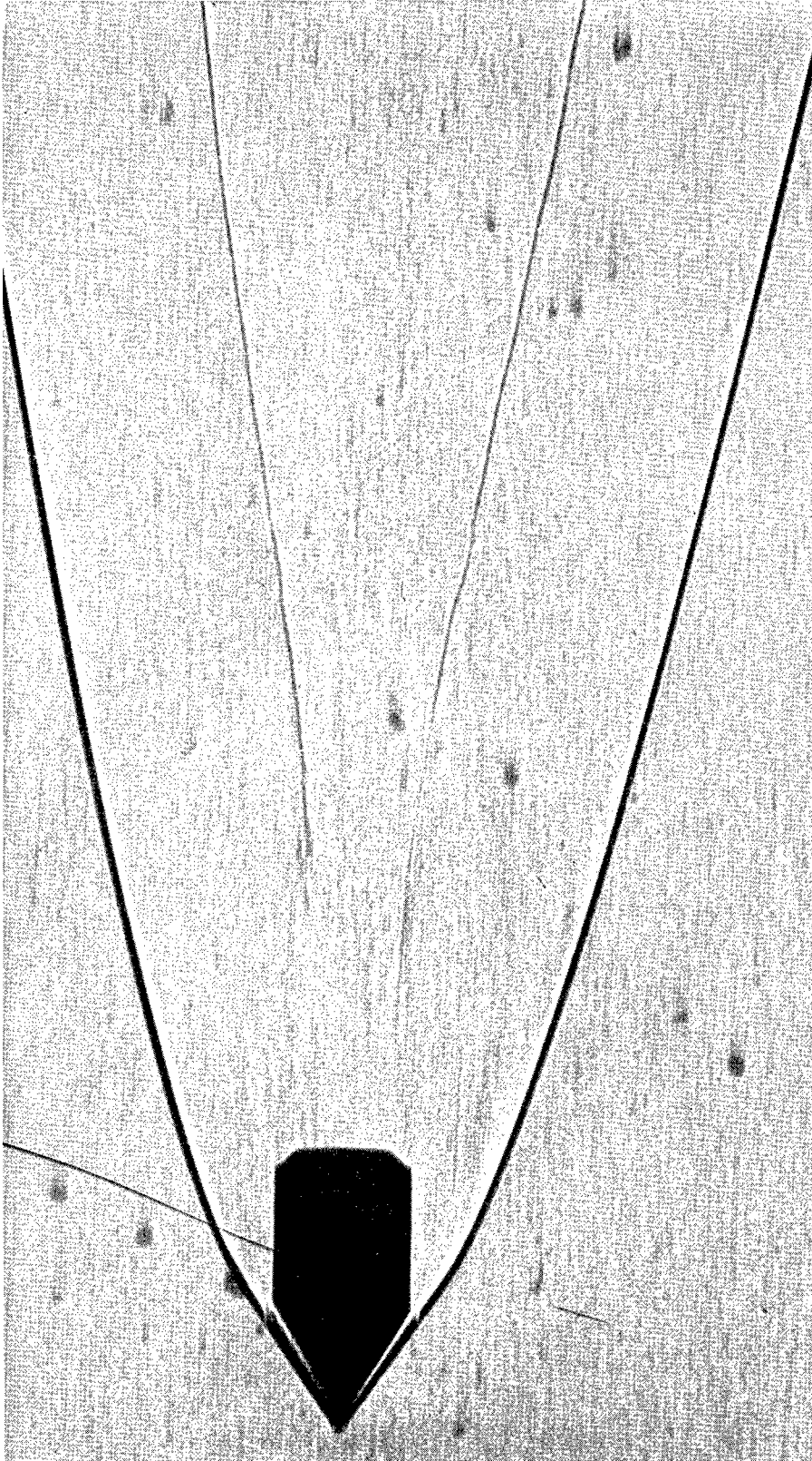
(c) 60° cone, Mach number 6.7.
