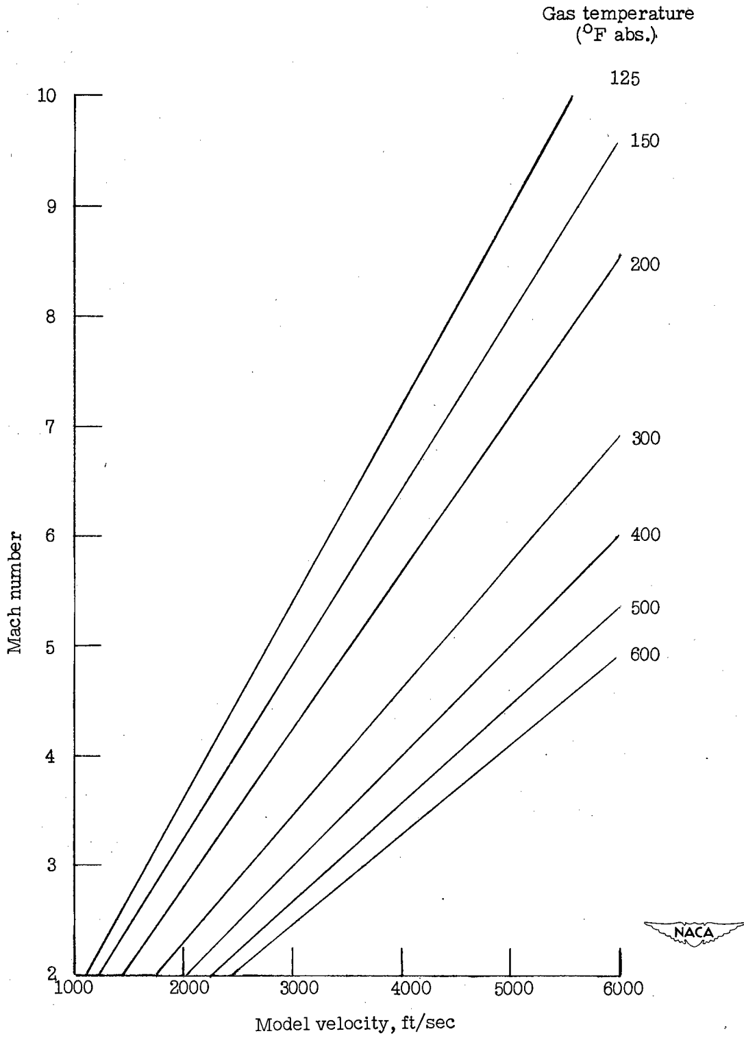
Figure 8.- Mach number, temperature, and model-velocity graph computed by using the velocity of sound at 0.1 atmosphere in nitrogen.
