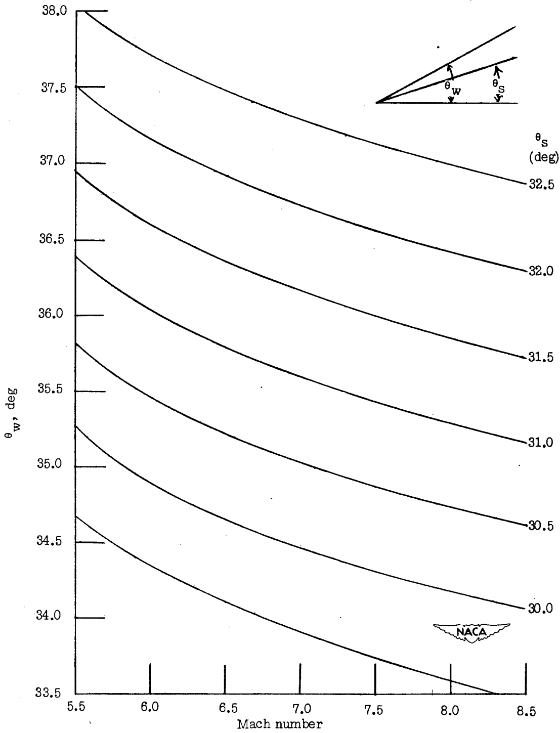
(b) 60^\circ cone.
