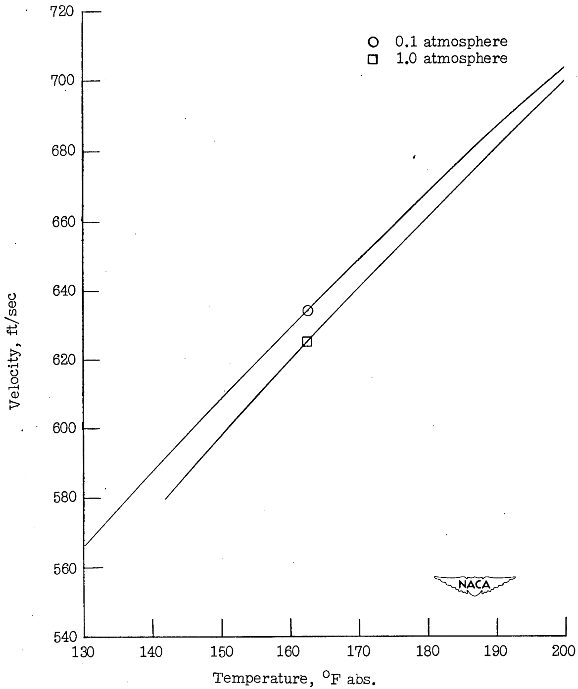
Figure 7.- Variation of the velocity of sound in nitrogen with absolute temperature. Indicated points from reference 5.
