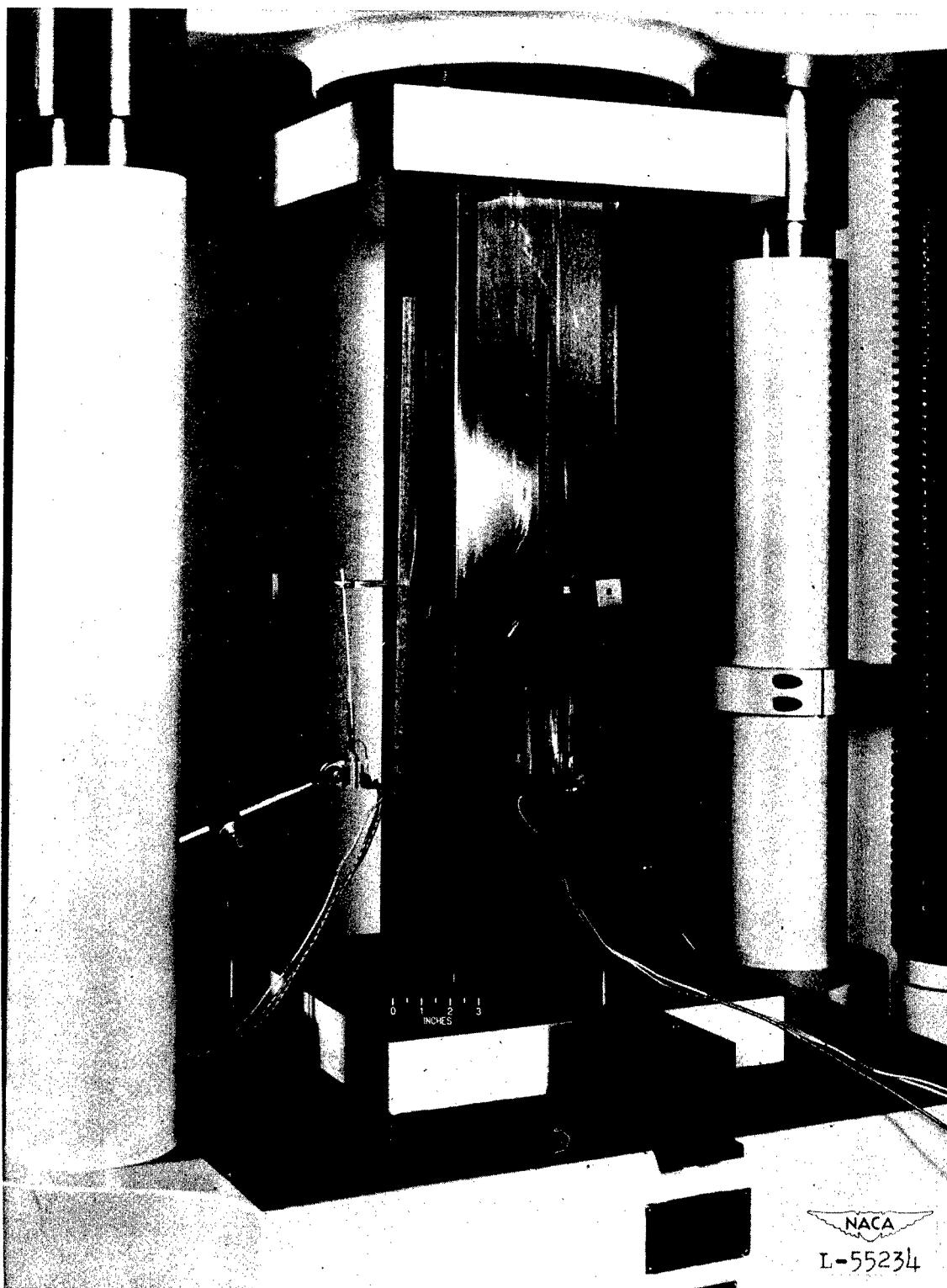
Figure 3.- Method of detecting buckling of plate elements of a square tube under test.
