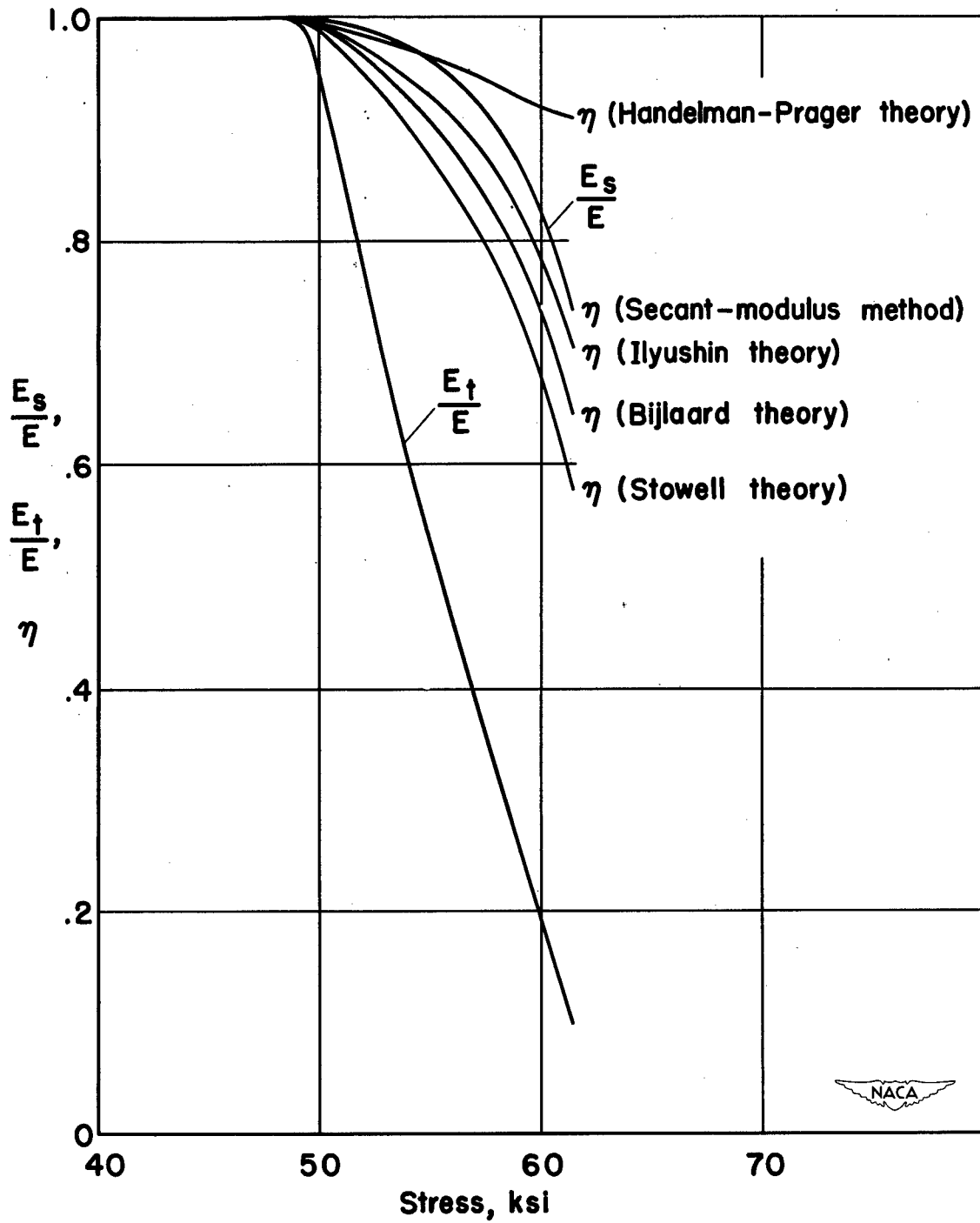
Figure 8.—Variation of \frac{E_s}{E} , \frac{E_t}{E} , and nondimensional coefficient \eta with stress for 14S-T6 aluminum alloy.
