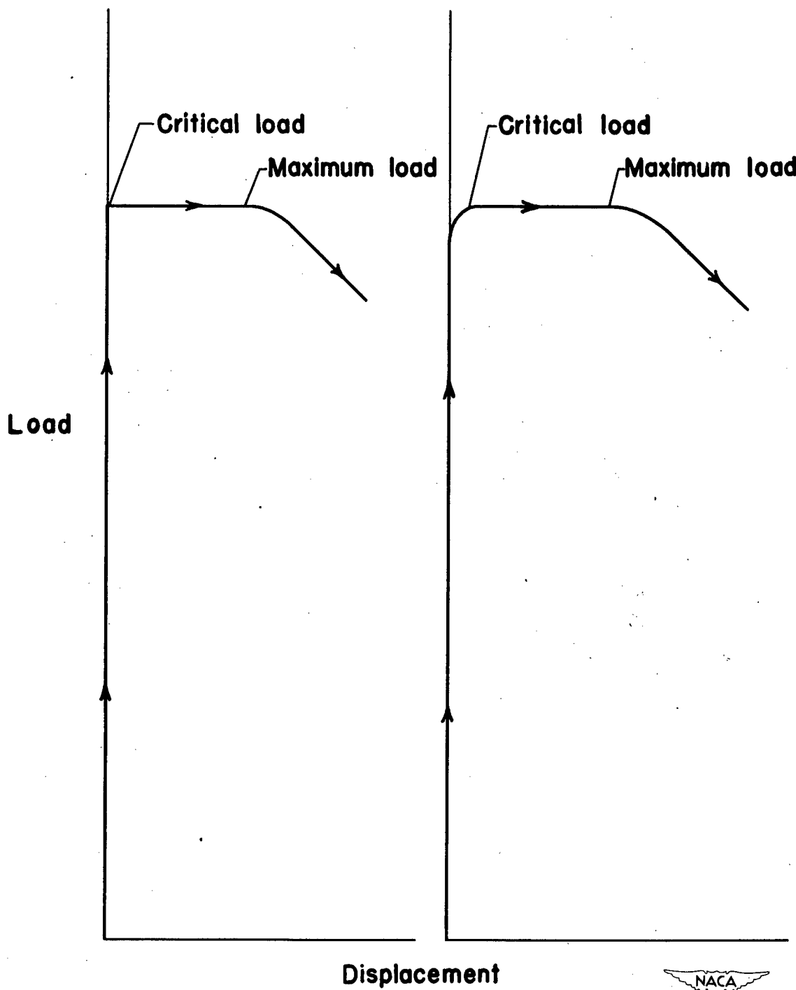
Figure 4.— Load-displacement curves for two adjoining plates of square tube specimen 9b.
