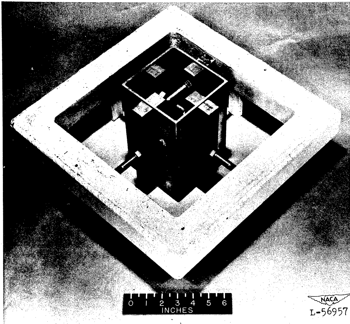
Figure 2.— Method of supporting individual plates of a square tube for compression stress-strain tests.
