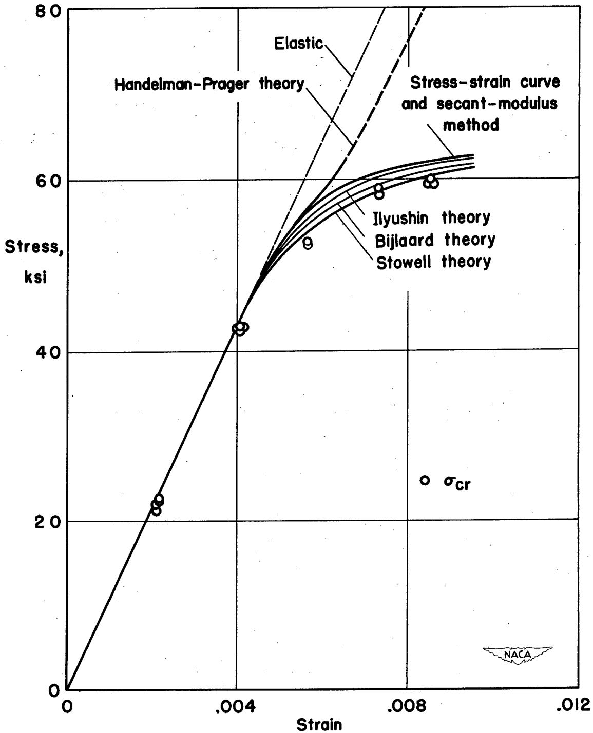
Figure 9.— Correlation of adjusted test results for the critical compressive stress with calculated plate buckling curves for long, simply supported, flat plates of 14S-T6 aluminum alloy. (Calculated elastic critical compressive strain used for plate tests.)
