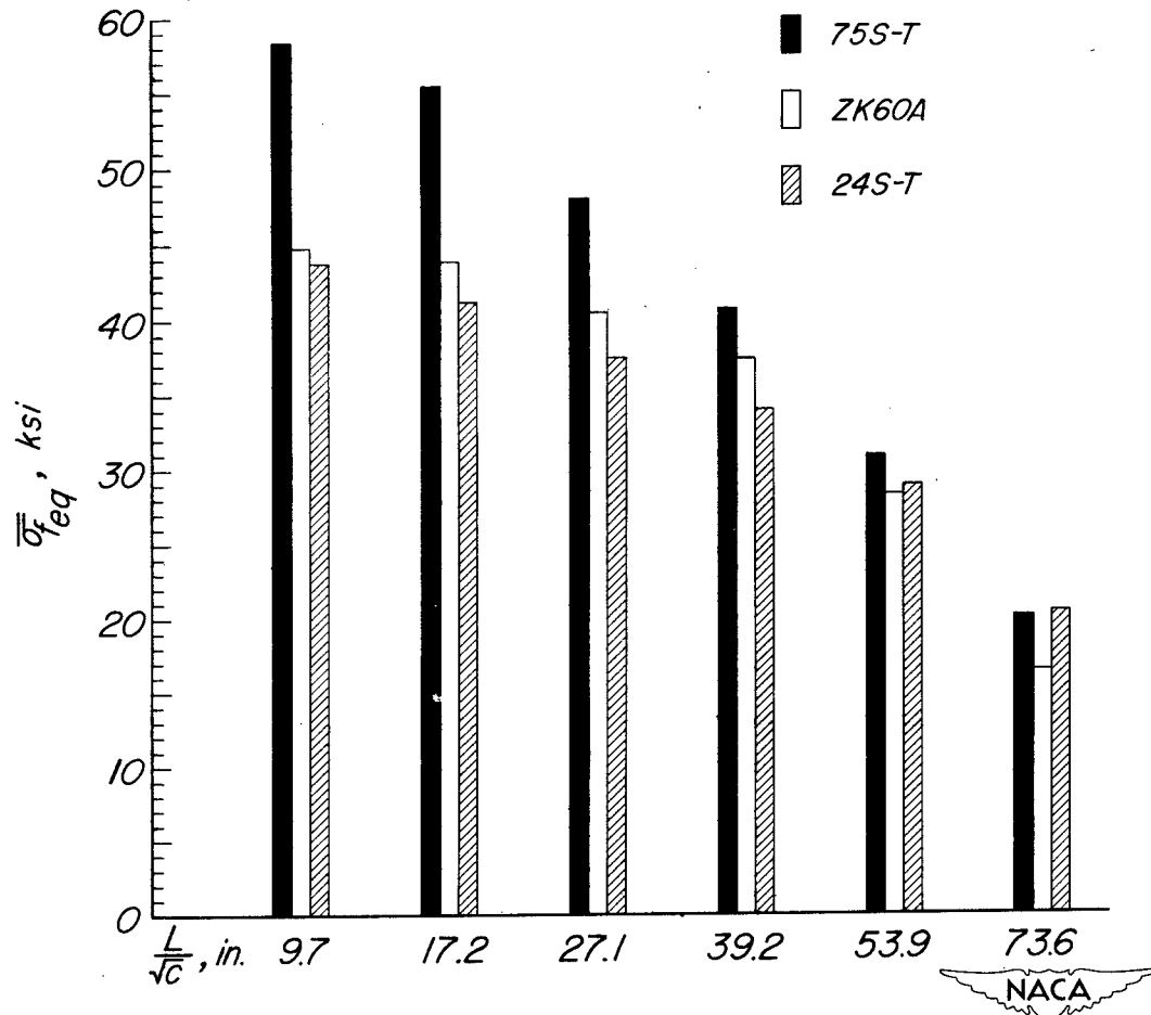
Figure 6.—Comparison of equivalent stresses carried by ZK60A extruded panels and the corresponding minimum weight designs of 24S-T and 75S-T Y-stiffened panels.
