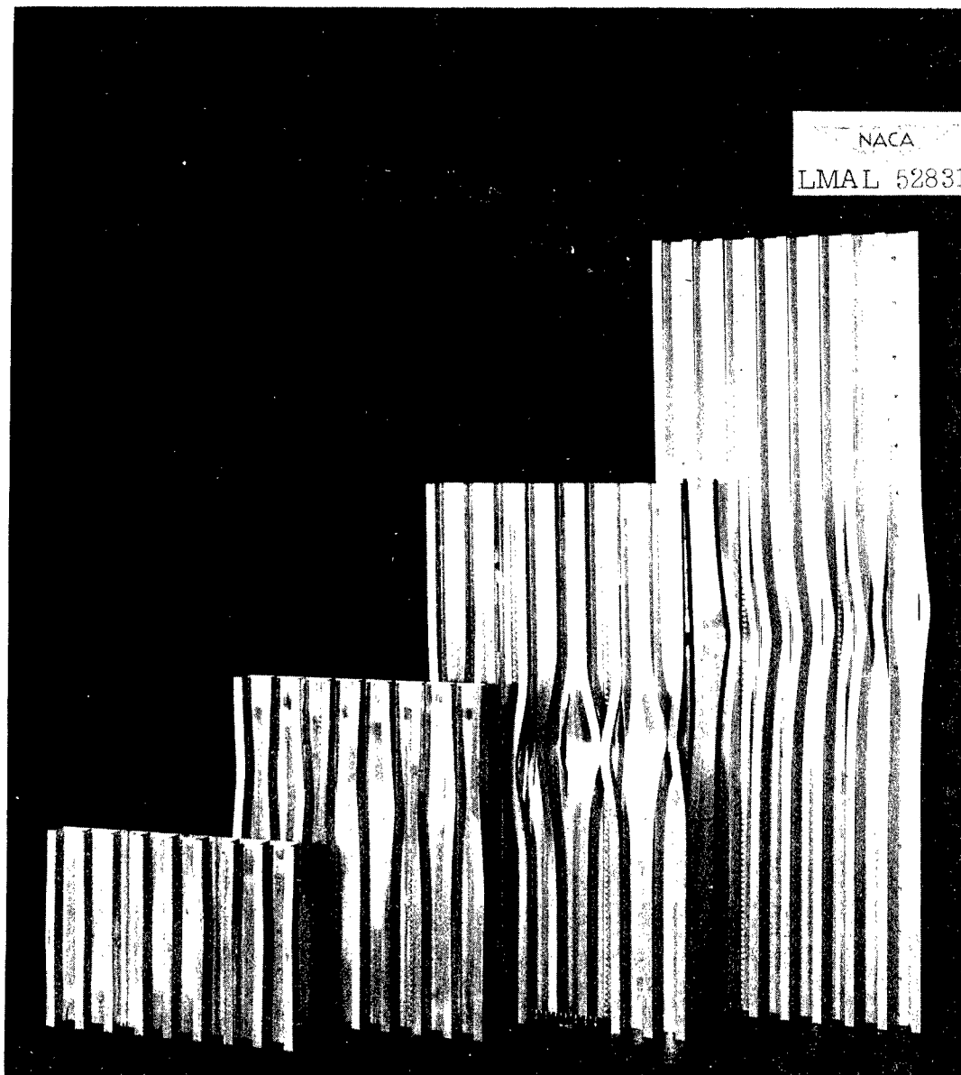
Figure 2.- Tested specimens having L/\rho of 20, 35, 55, and 80.
