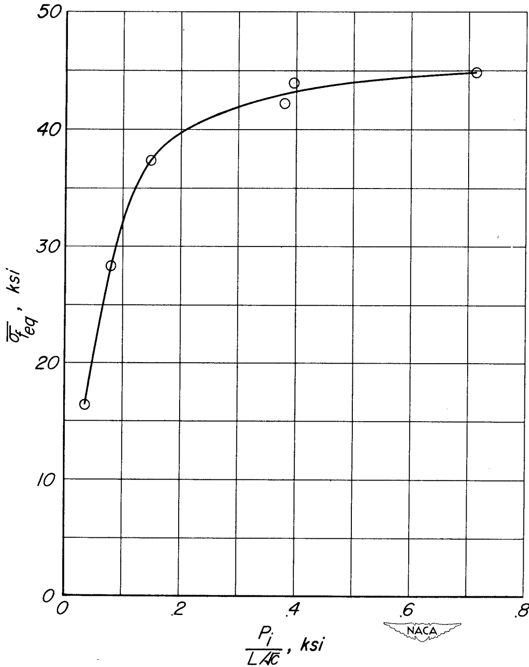
Figure 5.—Variation of stress with \frac{P_i}{LAc} for extruded panels.
