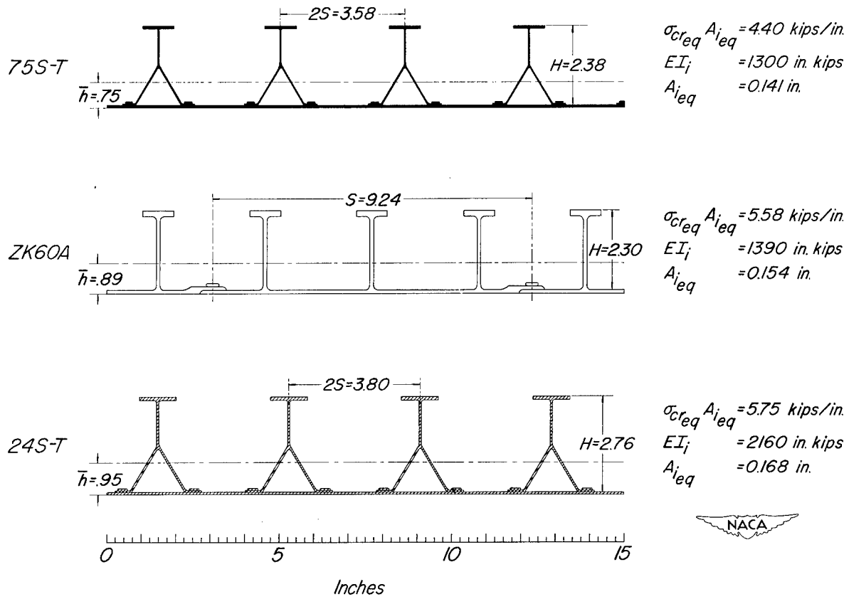
Figure 7.- Comparison of characteristics of the ZK60A extruded panel and 24S-T and 75S-T Y-stiffened panel designs for P_j = 5.75 kips per inch, t_{seq} = 0.064 inch, and \frac{L}{\sqrt{c}} = 39.2 inches.
