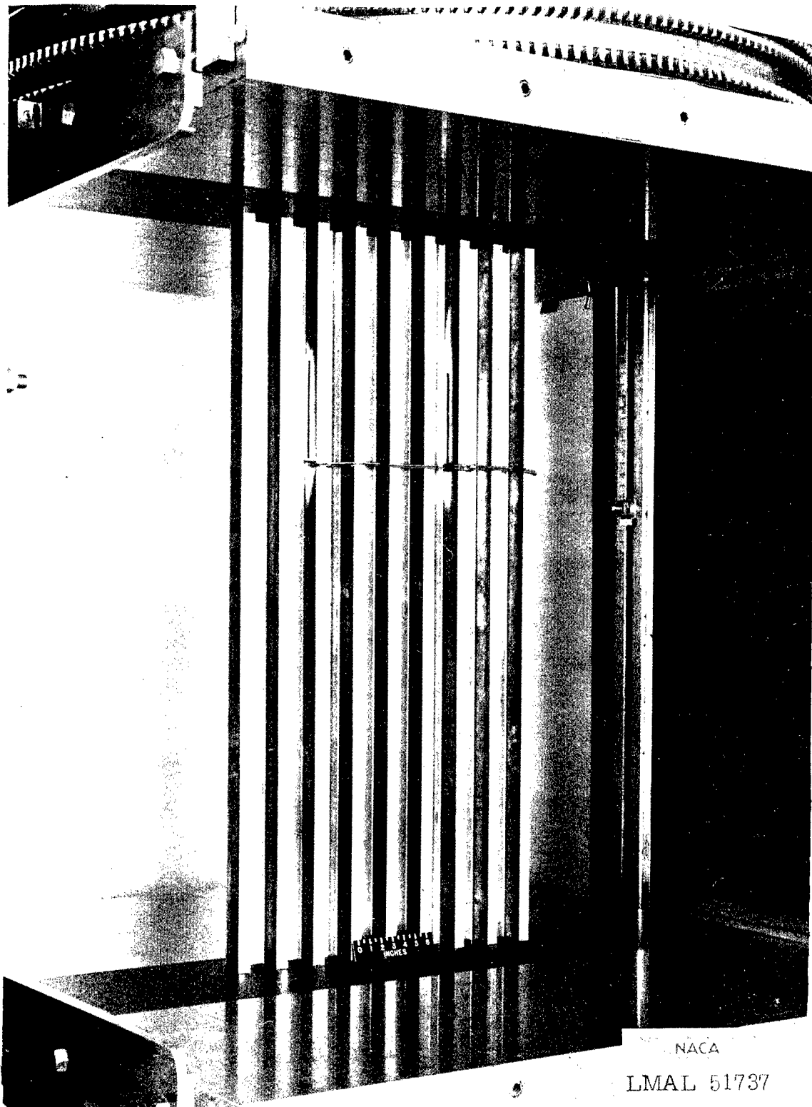
Figure 4.- Test specimen in testing machine. \frac{L}{p} = 55.
