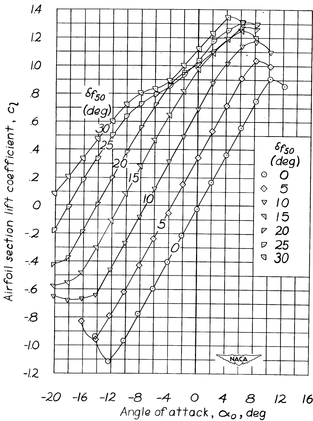
Figure 5.- Aerodynamic section characteristics of an NACA 0009 airfoil with a 0.50c plain flap and sealed gap.
