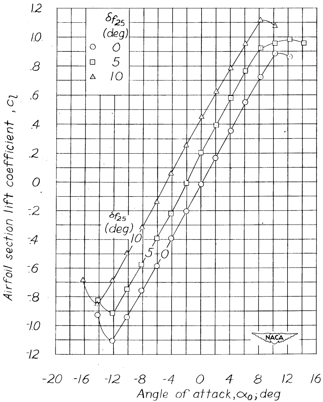
Figure 2 . - Aerodynamic section characteristics of an NACA 0009 airfoil with a 0.25c plain flap and 0.005c gap.
