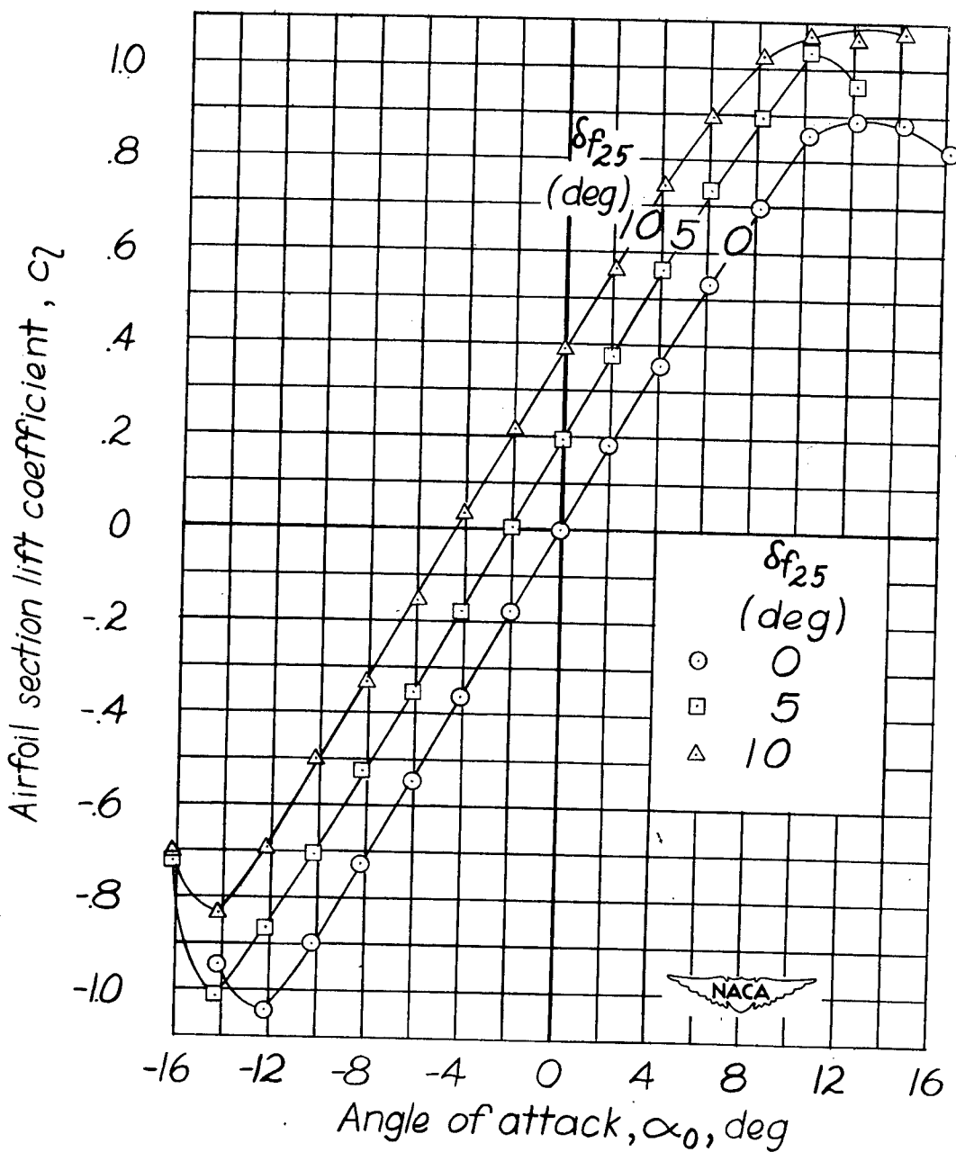
Figure 7.- Effect of deflecting the 0.25c flap on the aerodynamic section characteristics of an NACA 0009 airfoil having a 0.25c and a 0.50c plain flap. \delta f_{50} = 0^\circ ; gaps, 0.005c.
