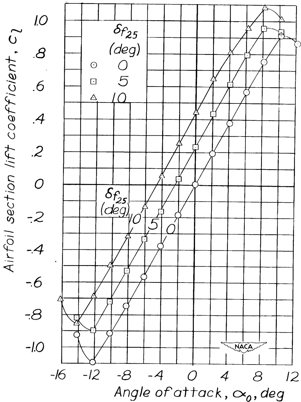
Figure 9.- Effect of deflecting the 0.25c flap on the aerodynamic section characteristics of an NACA 0009 airfoil having a 0.25c and a 0.50c plain flap. \delta f_{50} = 0^\circ ; gaps, sealed.
