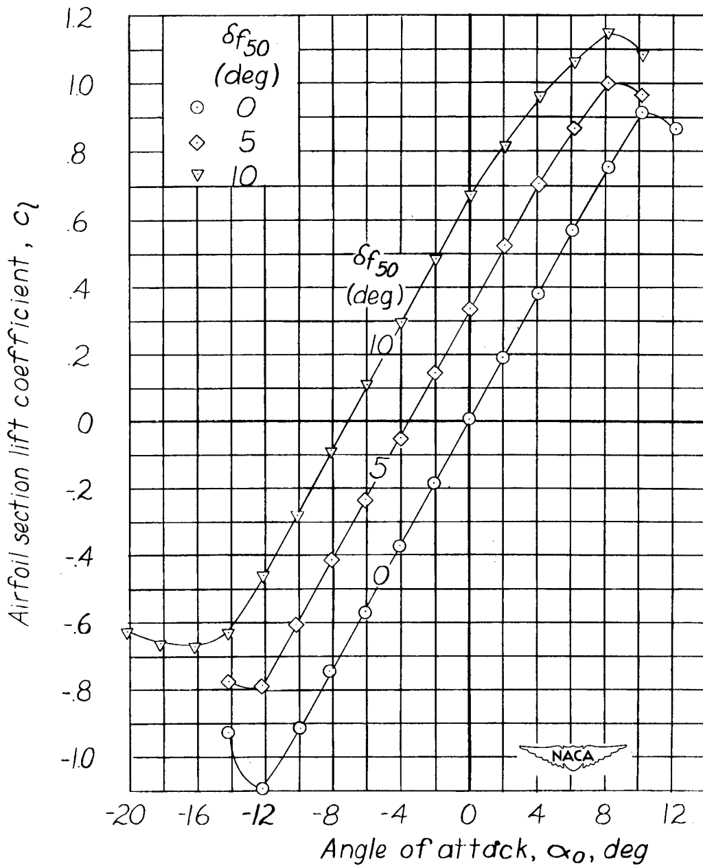
Figure 10 - Effect of deflecting the 0.50c flap on the aerodynamic section characteristics of an NACA 0009 airfoil having a 0.25c and a 0.50c plain flap. \delta f_{25} = 0^\circ ; gaps, sealed.
