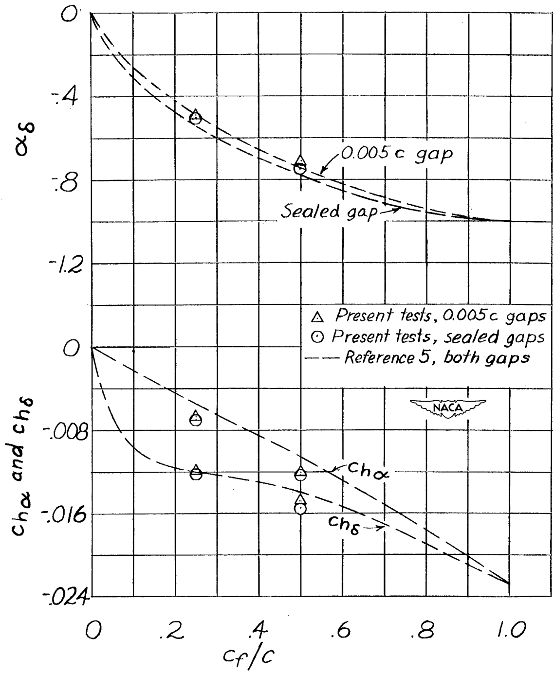
Figure 6.- Variation of lift-effectiveness and flap section hinge-moment parameters with ratio of flap chord to airfoil chord. Curves from reference 5 for plain flaps on NACA 0009 airfoil.
