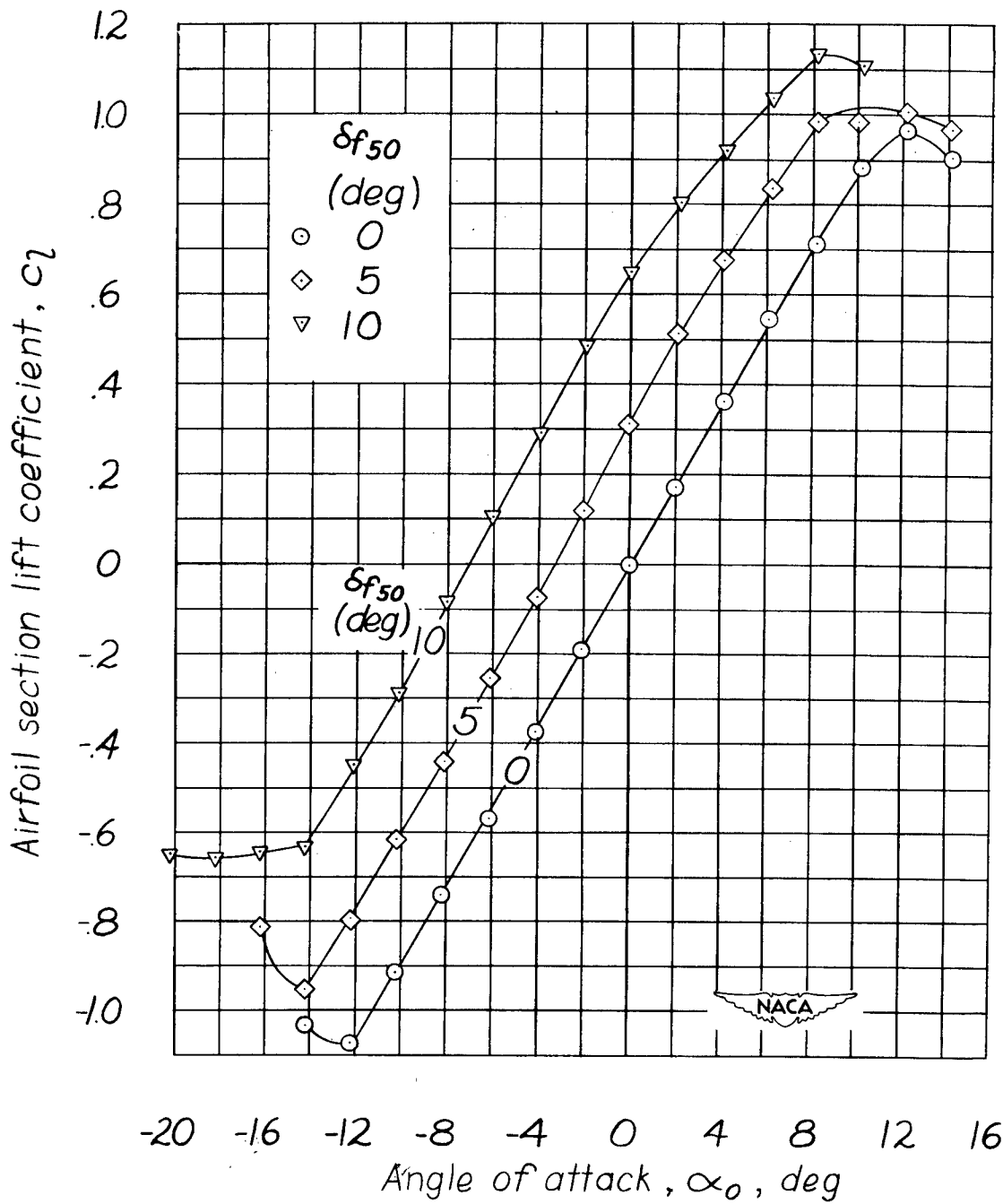
Figure 4.- Aerodynamic section characteristics of an NACA 0009 airfoil with a 0.50c plain flap and 0.005c gap.
