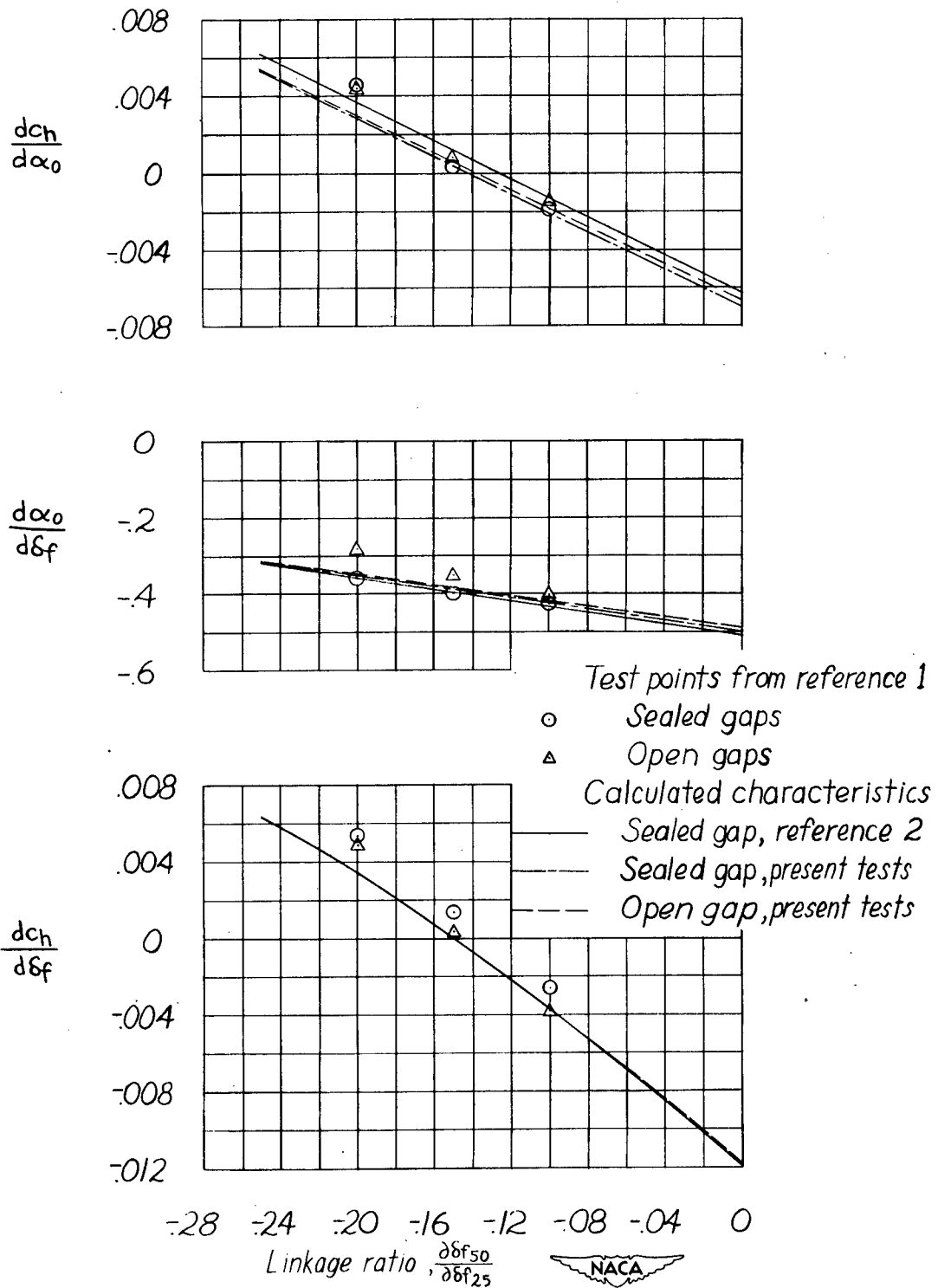
Figure 11.-Comparison of the aerodynamic characteristics of an NACA 0009 airfoil with a 0.25c flap and a 0.50 c tab obtained from experiment and from theory.
