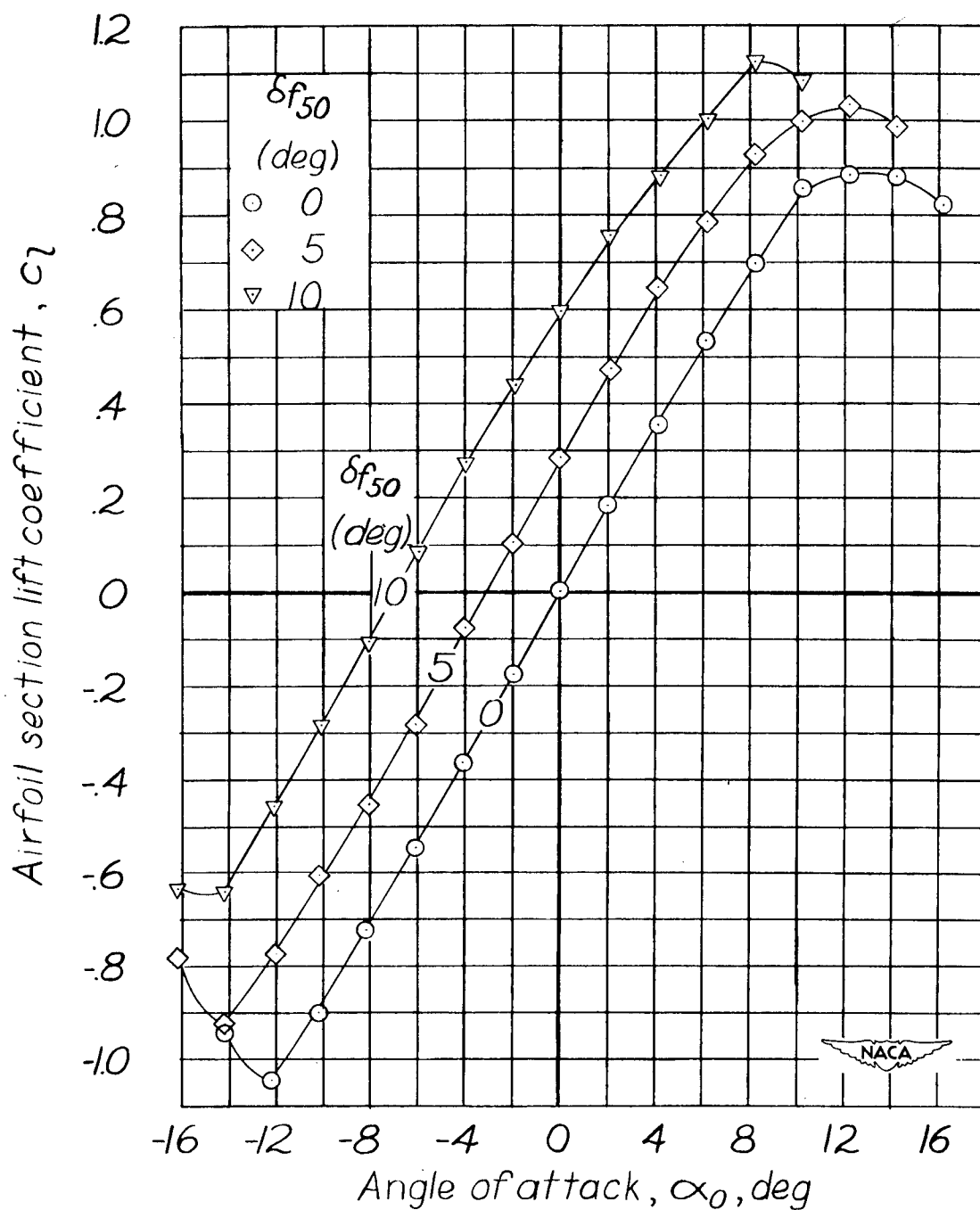
Figure 8.- Effect of deflecting the 0.50c flap on the aerodynamic section characteristics of an NACA 0009 airfoil having a 0.25c and a 0.50c plain flap. \delta_{f25} = 0^\circ ; gaps, 0.005c.
