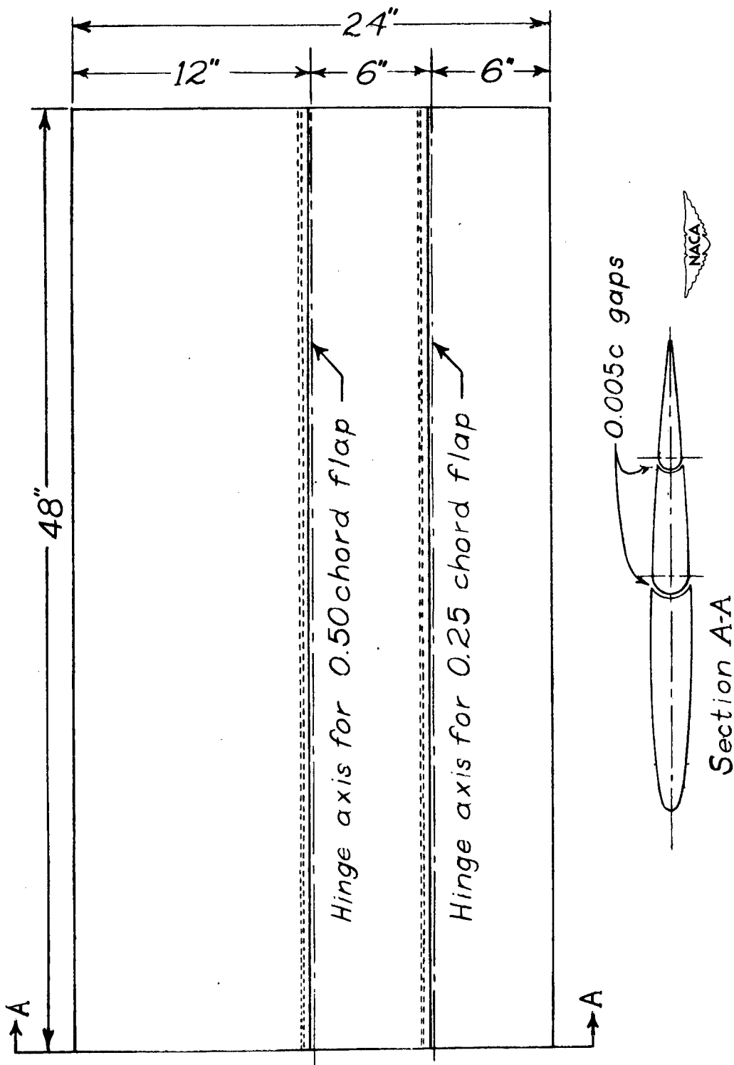
Figure 1.- Details of NACA 0009 model with 0.25c and 0.50c plain flaps.
