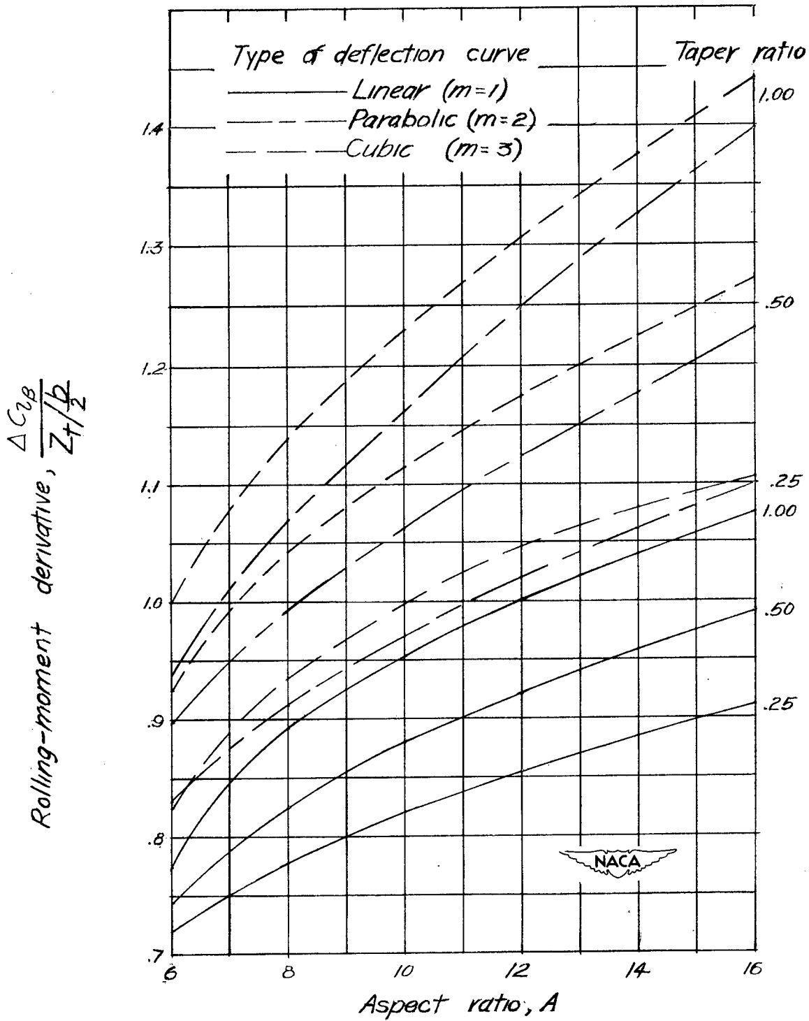
Figure 2.— Variation of increment in rolling-moment derivative with aspect ratio and taper ratio for several types of deflection curves.
