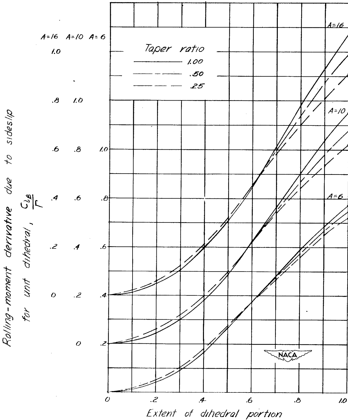
Figure 1.- Rolling-moment derivative due to sideslip plotted against extent of dihedral portion. (From fig. 16 of reference 1.)
