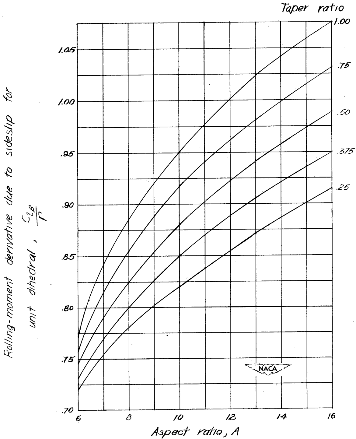
Figure 4.- Variation of rolling-moment derivative with aspect ratio and taper ratio for rigid wing ( m=1 ).
