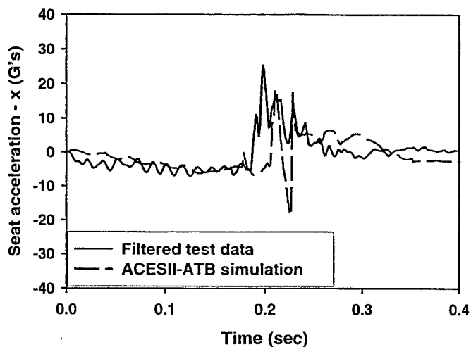
Figure 10. Comparison of seat accelerations-X (144 KEAS case).
