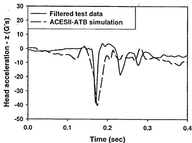
Figure 12. Comparison of pilot head accelerations-Z (144 KEAS case).
