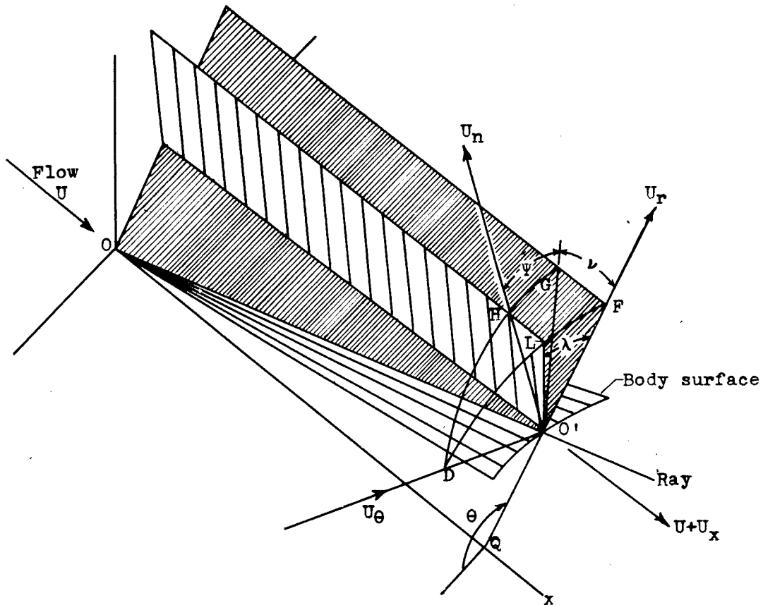
(a) Projection sketch of body surface and velocity components.
