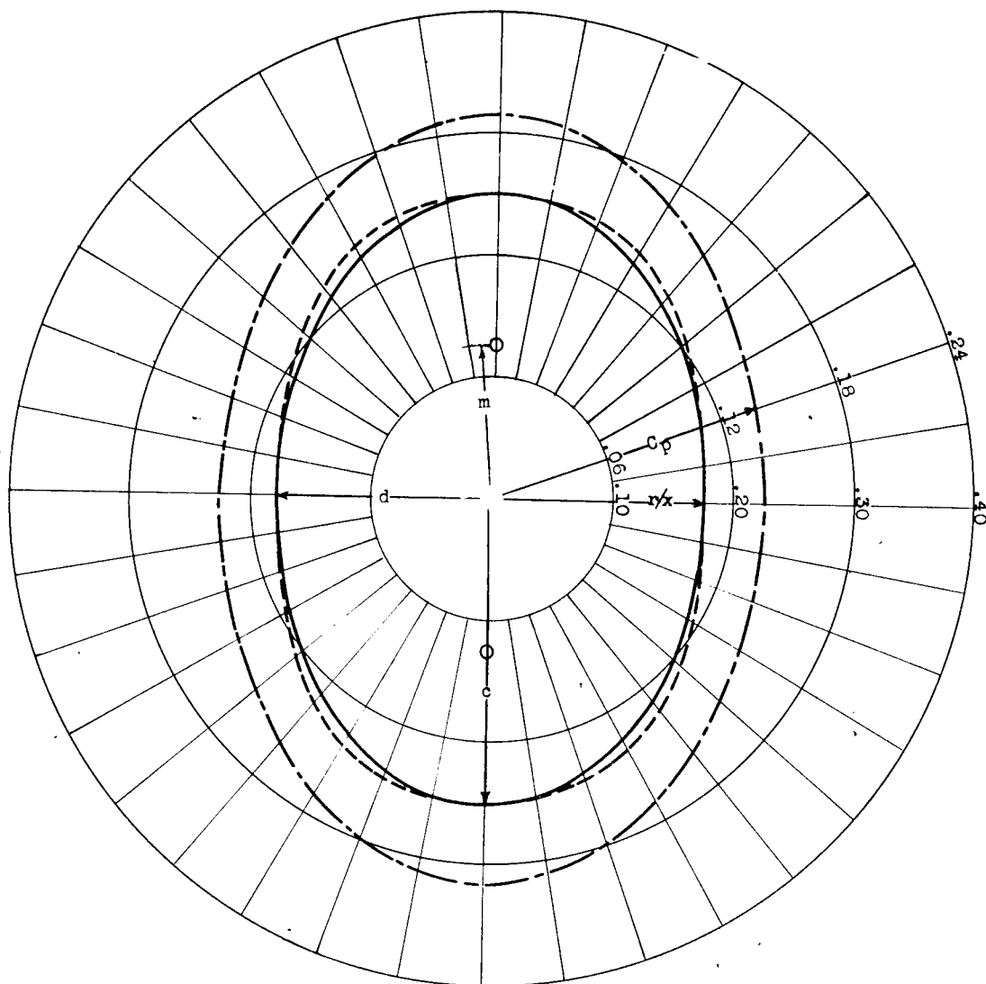
Figure 3. - Comparison of desired elliptical body with calculated body and resulting pressure distribution. \beta = 1.5 ; m = 0.125 ; K/U = 0.0220 .
