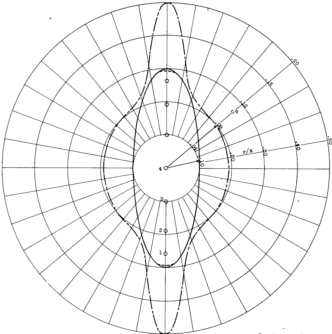
Figure 6. - Comparison of desired slender elliptical body with calculated body and resulting pressure distribution. \beta = 1.5 .
