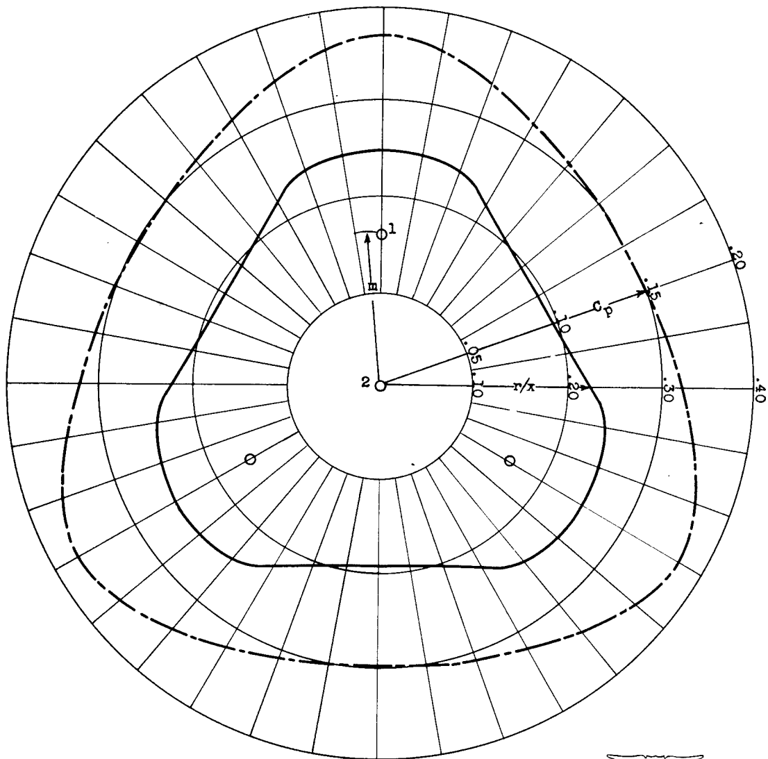
Figure 7. - Comparison of desired modified triangular body with calculated body and resulting pressure distribution. \beta = 1.5 ; m = 0.16 ; K_1/U = 0.0102 ; K_2/U = 0.0154 .
