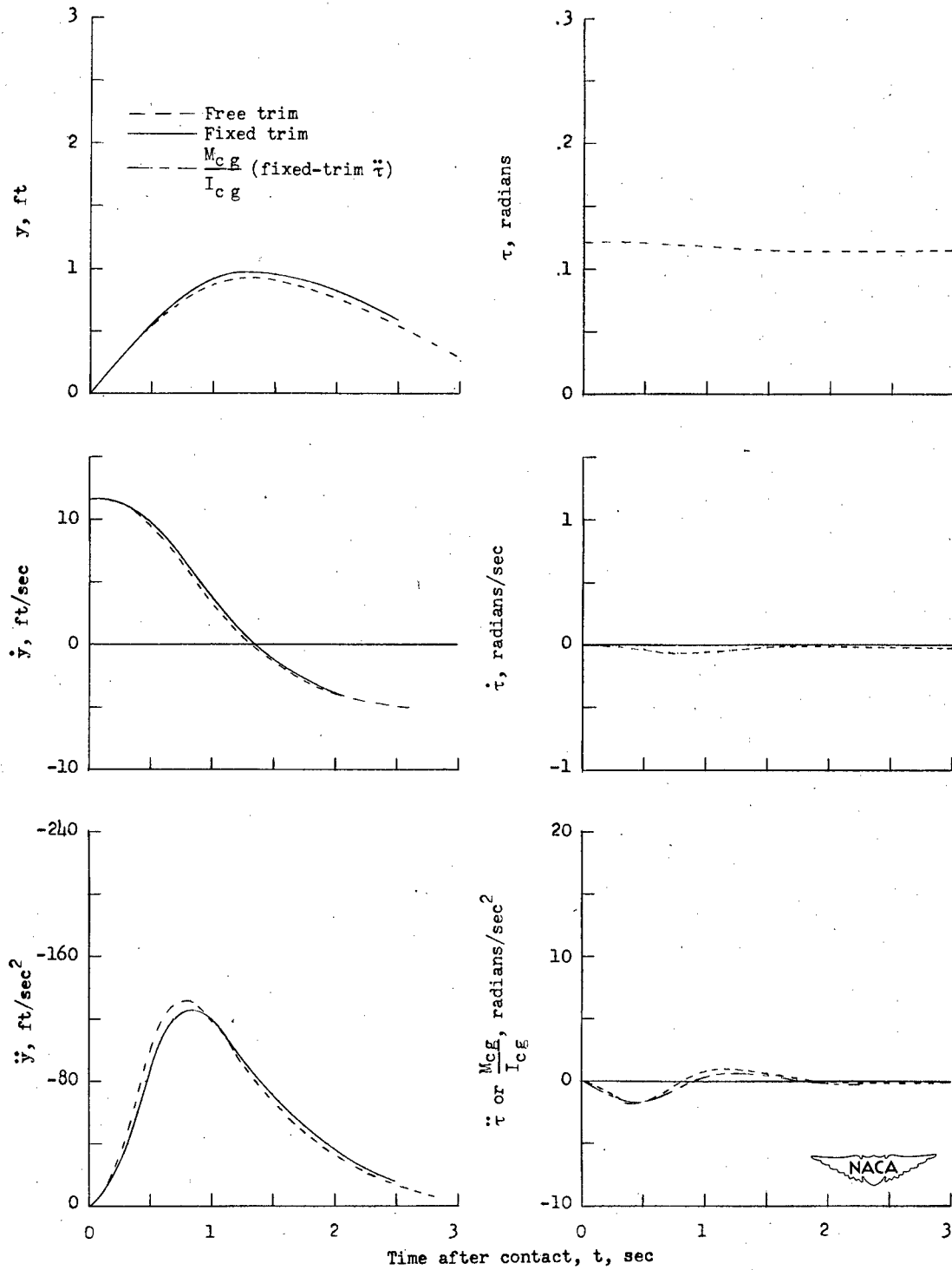
(a) Case I; \tau_0 = 7.0^\circ or 0.122 radian; \gamma_0 = 5.4^\circ .
