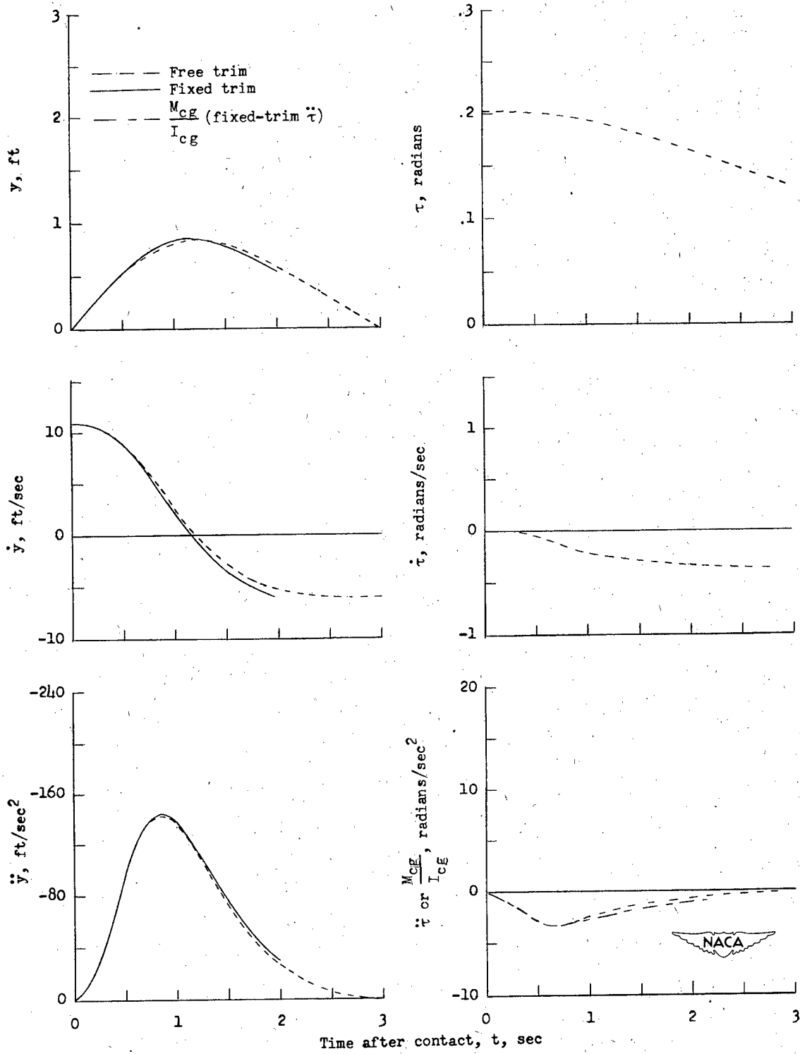
(b) Case II; \tau_0 = 11.5^\circ or 0.201 radian; \gamma_0 = 5.0^\circ .
