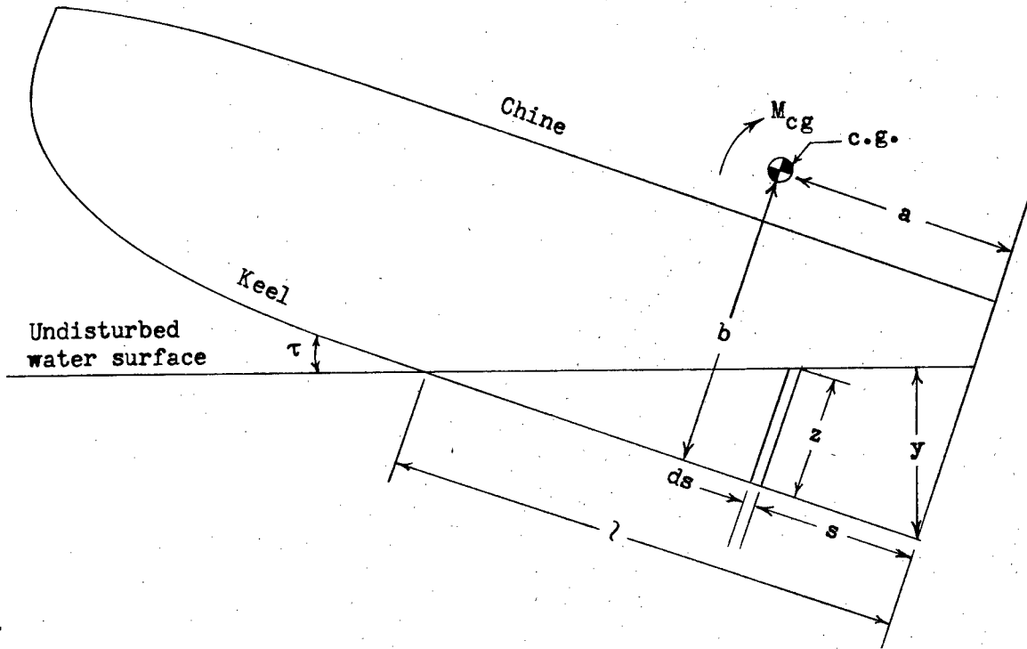
(a) Sketch of float during impact.
