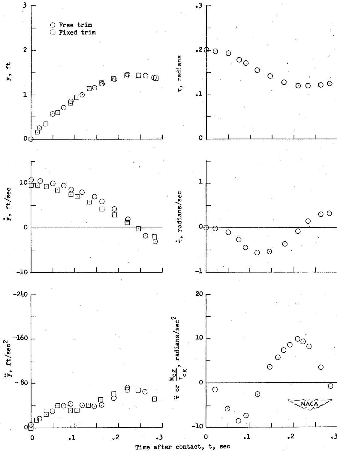
(b) Case II; \tau_0 = 12.0^\circ or 0.209 radian; \gamma_0 = 5.0^\circ .
