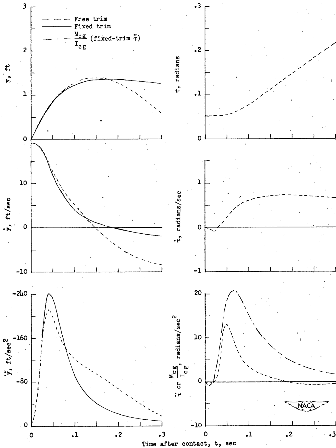
(c) Case III; \tau_0 = 3.0^\circ or 0.052 radian; \gamma_0 = 12.0^\circ .
