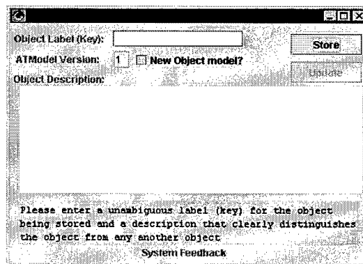
Figure 30: StoreGUI
