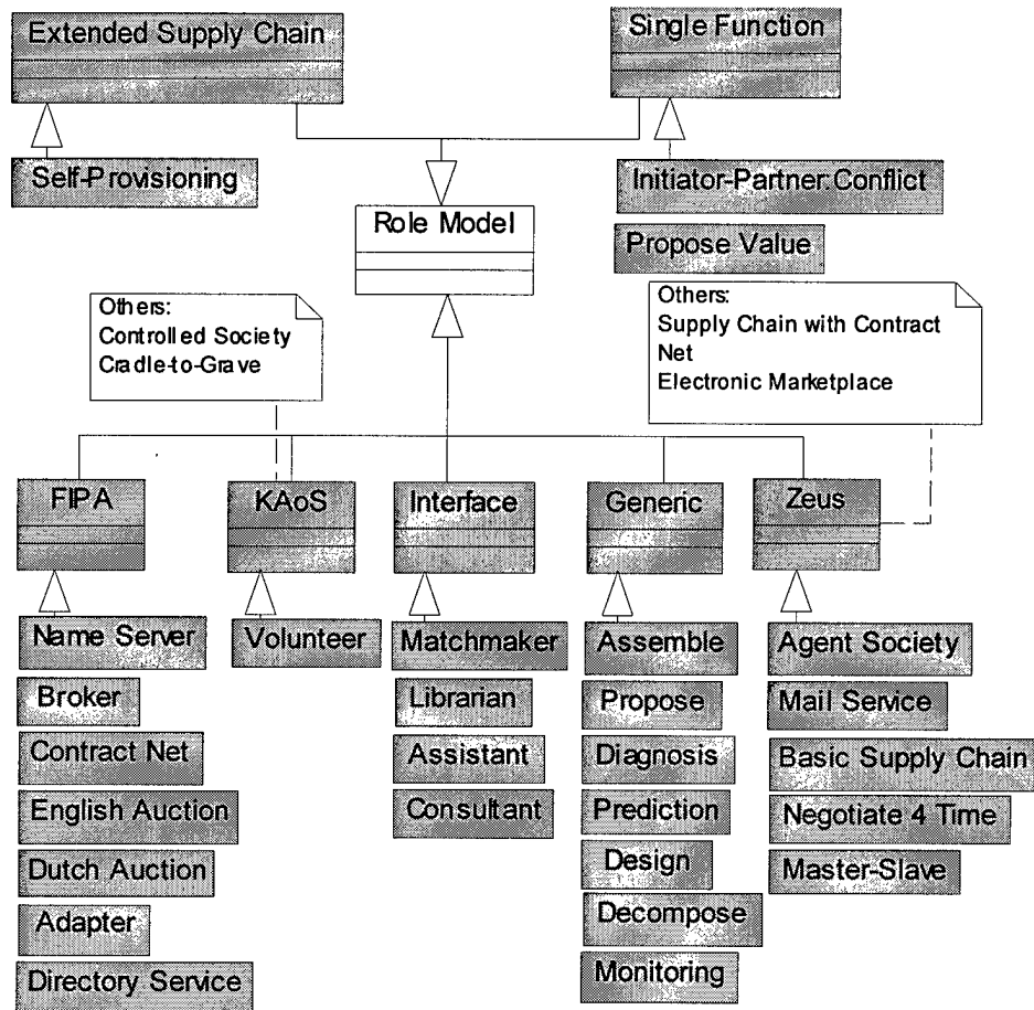
Figure 20: Role Model Taxonomy (Kendall 1998a)
