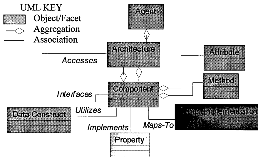
Figure 14: Agent Entity Sub-Domain
