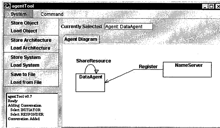
Figure 28: AgentTool GUI
