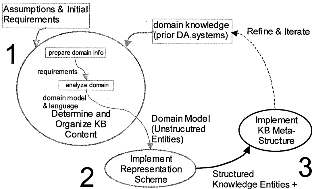
Figure 11: KBDM Stage 3 – Implementing KB Meta-Structure
