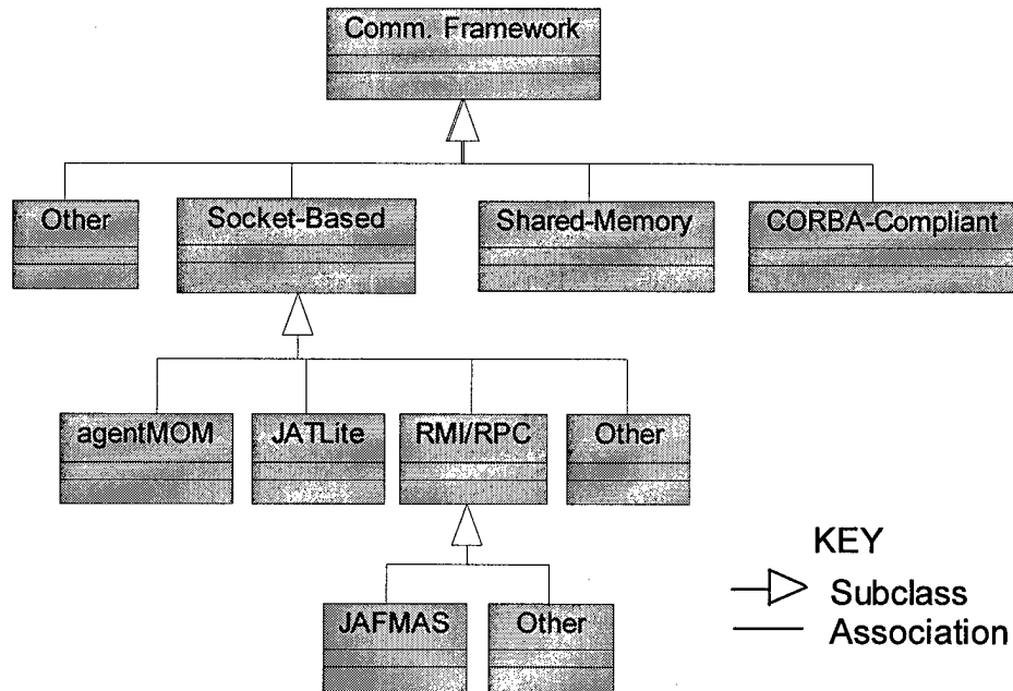
Figure 19: Agent System Framework Hierarchy
