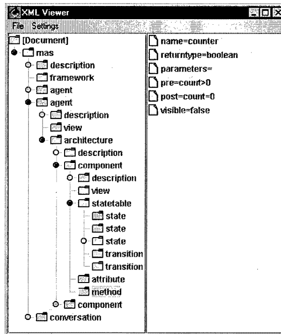
Figure 33: DOM-viewer Showing an Agent System Represented by MAML
