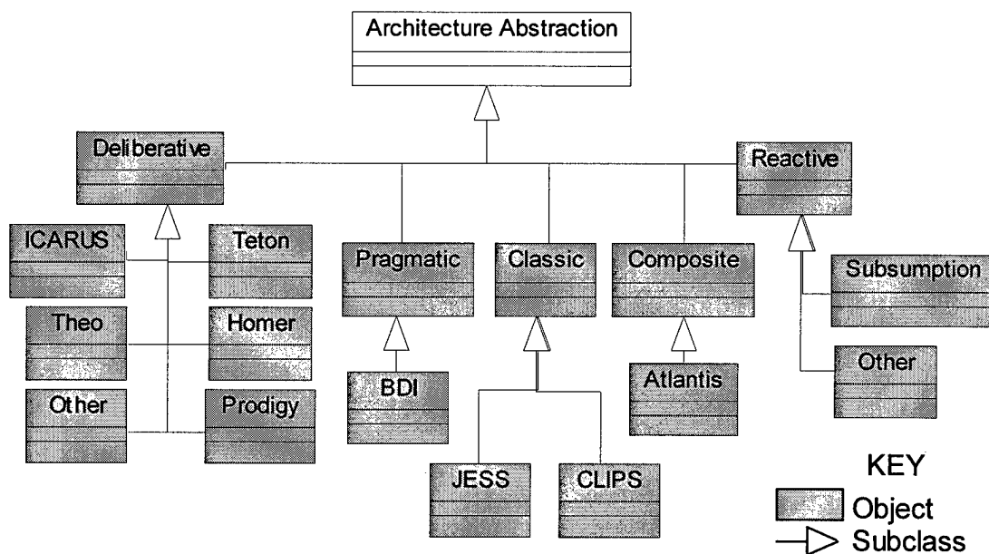
Figure 16: Architecture Abstraction Hierarchy
