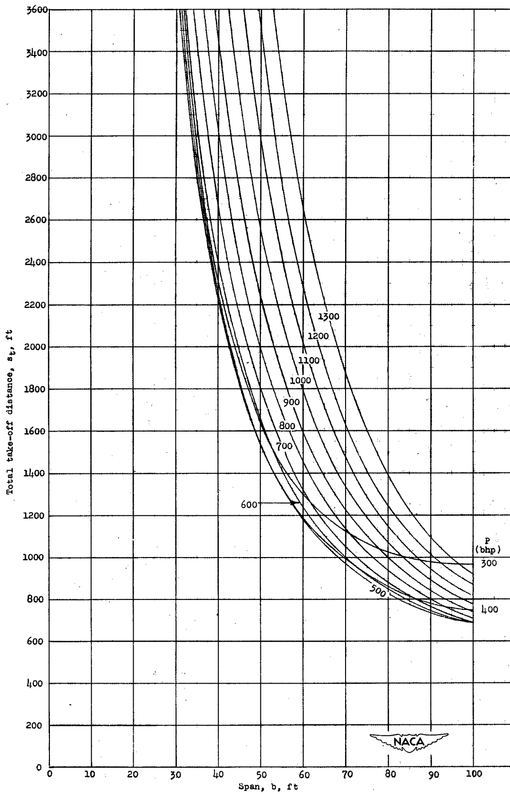
(c) A = 15 . Figure 9.- Concluded.
