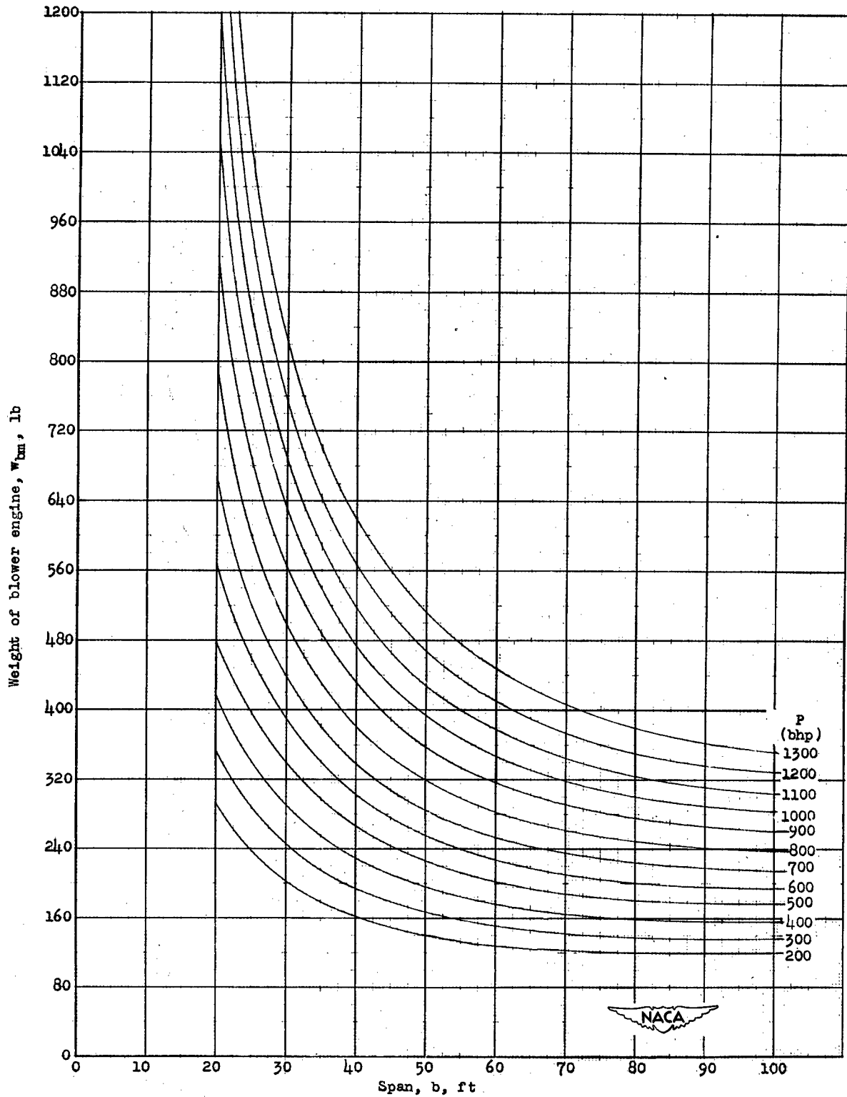
(a) Weight of blower engine.
