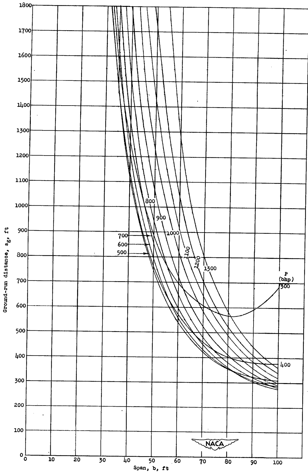
(b) A = 10 . Figure 15.- Continued.
