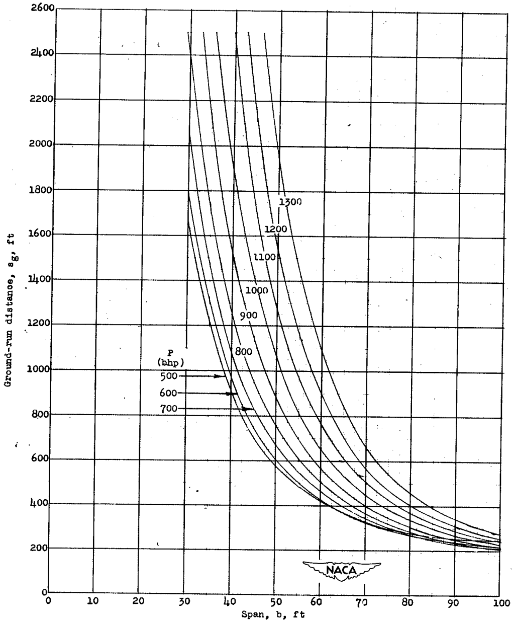
(b) A = 10 . Figure 16.- Continued.
