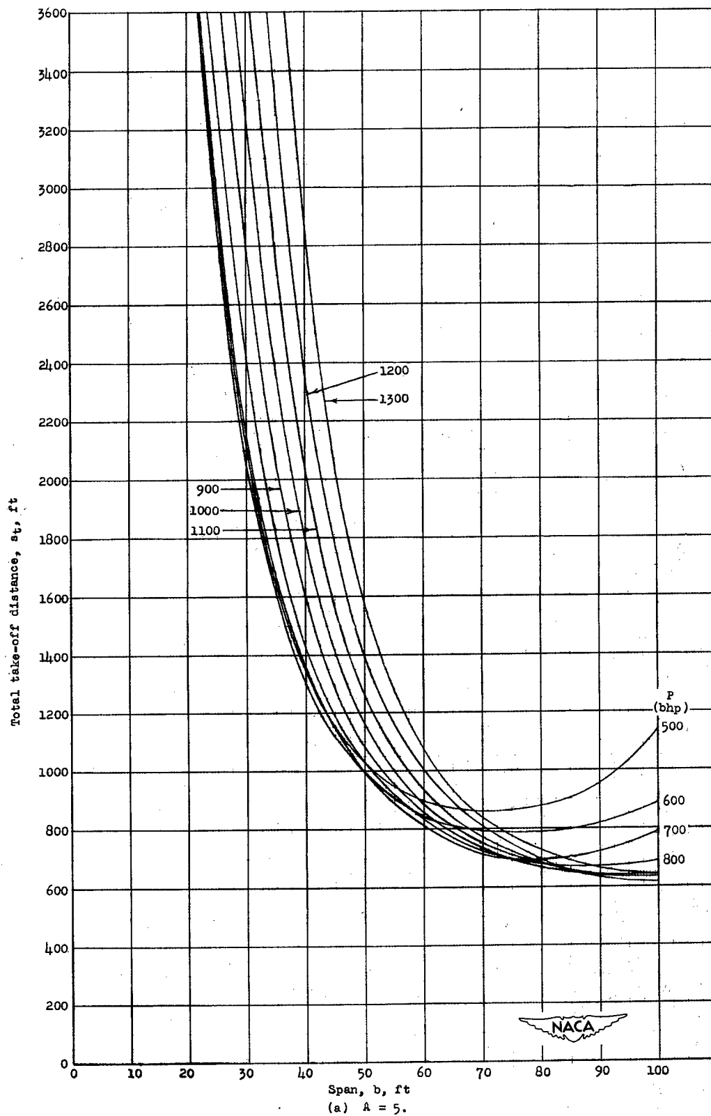
Figure 10.- Total take-off distance of an airplane with boundary-layer control as a function of span for various powers. (a) A = 5 .
