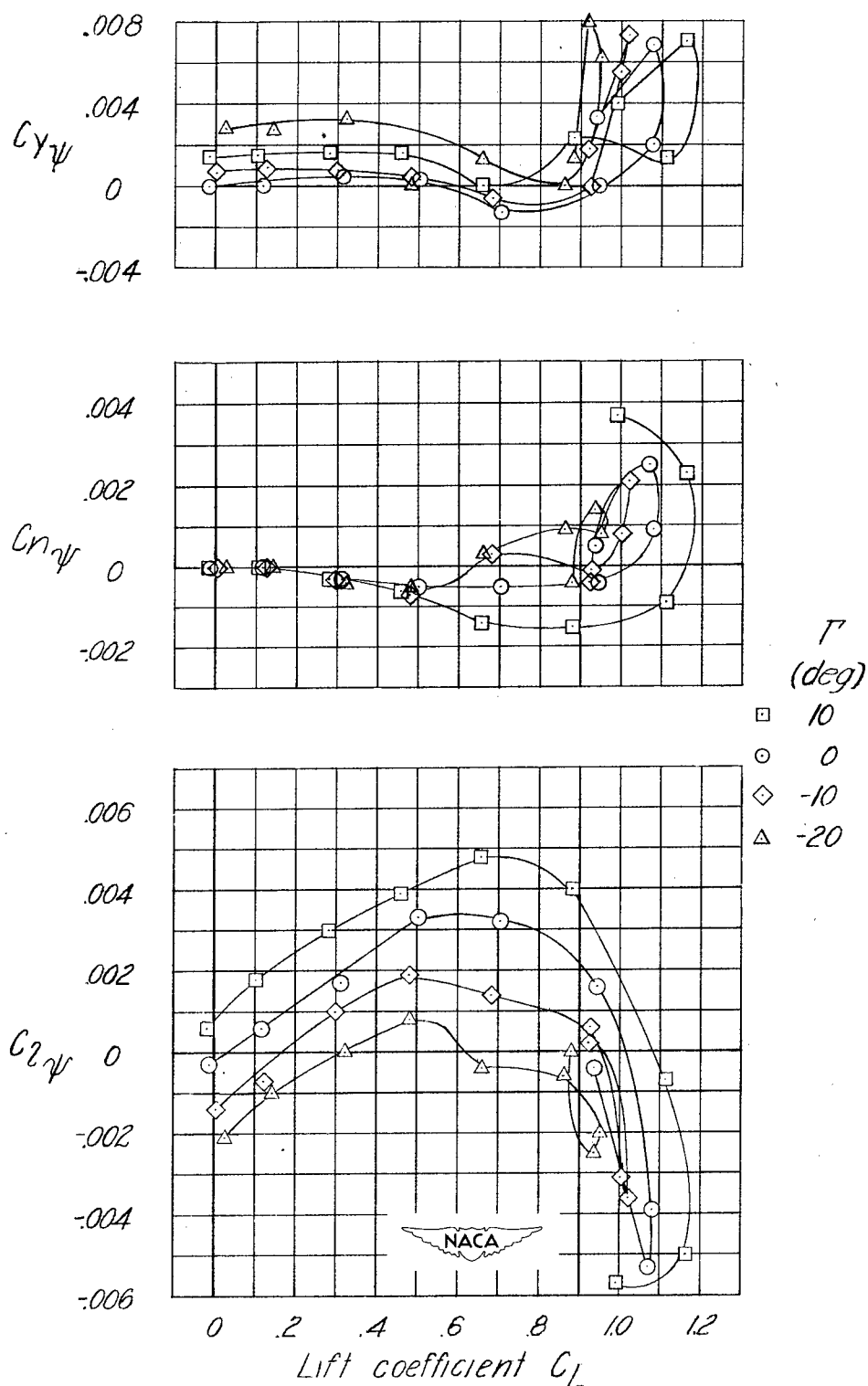
Figure 7.- Effect of dihedral angle on the variation of C_{l\psi} , C_{n\psi} , and C_{y\psi} with lift coefficient for a 45° sweptback wing of aspect ratio 2.61.
