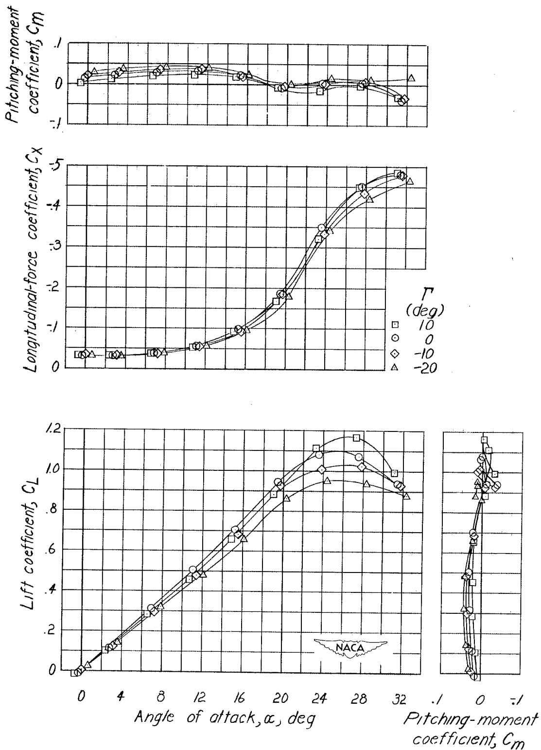
Figure 4.-Basic longitudinal-stability data of a 45° sweptback wing of aspect ratio 2.61 in straight flow. \psi = 0^\circ .
