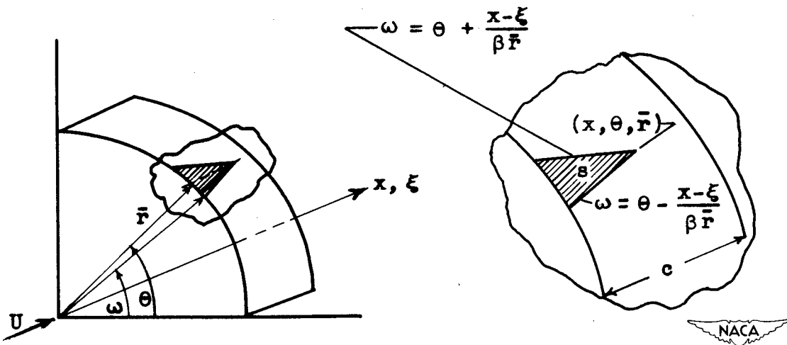
(b) Source distribution about circular cylinder (first quadrant shown).
