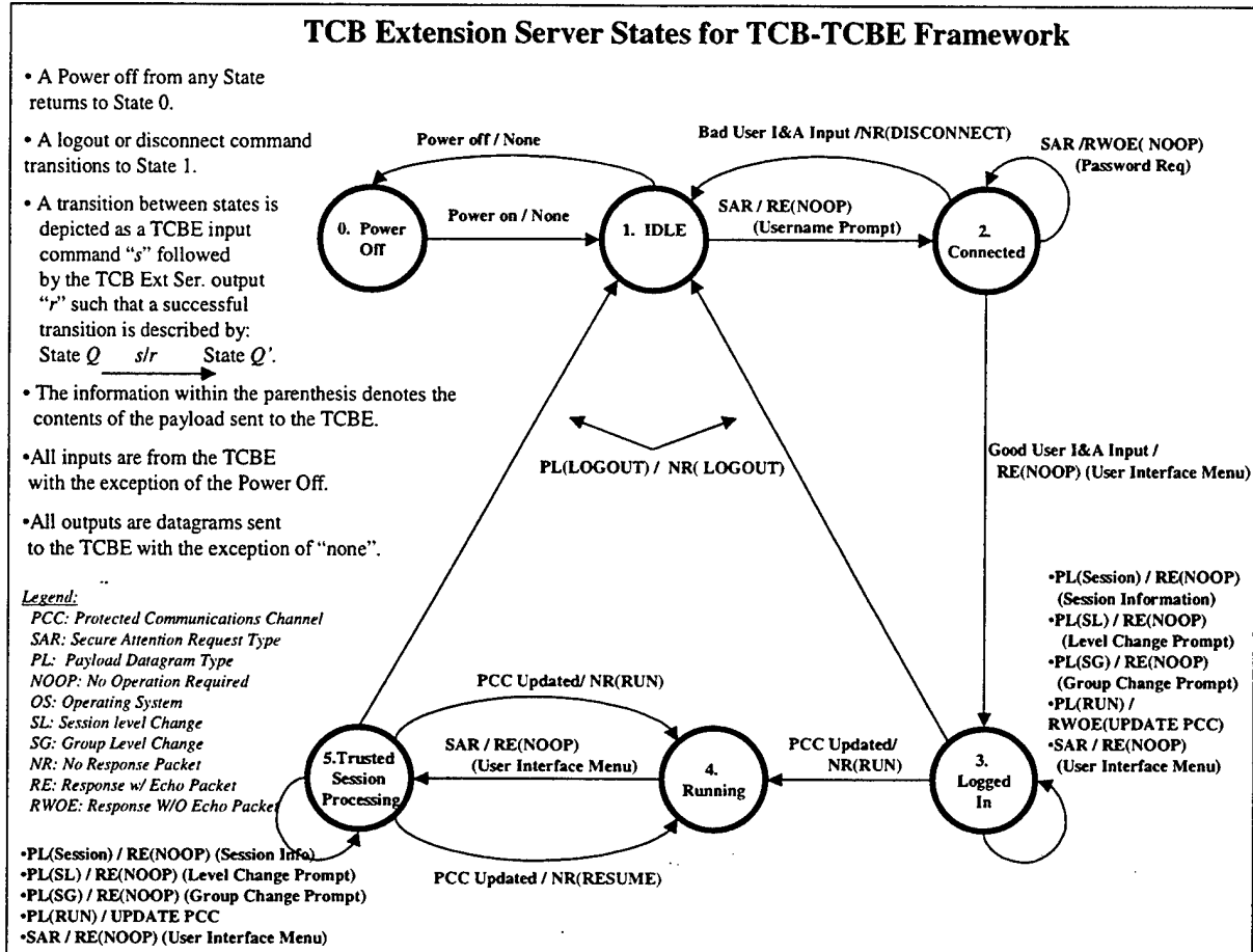
Figure 2. TCB Extension Server States for TCB-TCBE Framework
