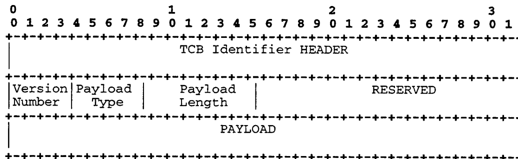
Figure 3. TCBE-to-TCB Extension Server Payload Datagram Format
