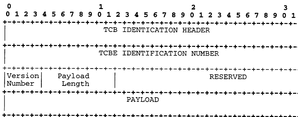
Figure 8. TCBE-to-Session Server Datagram Format
