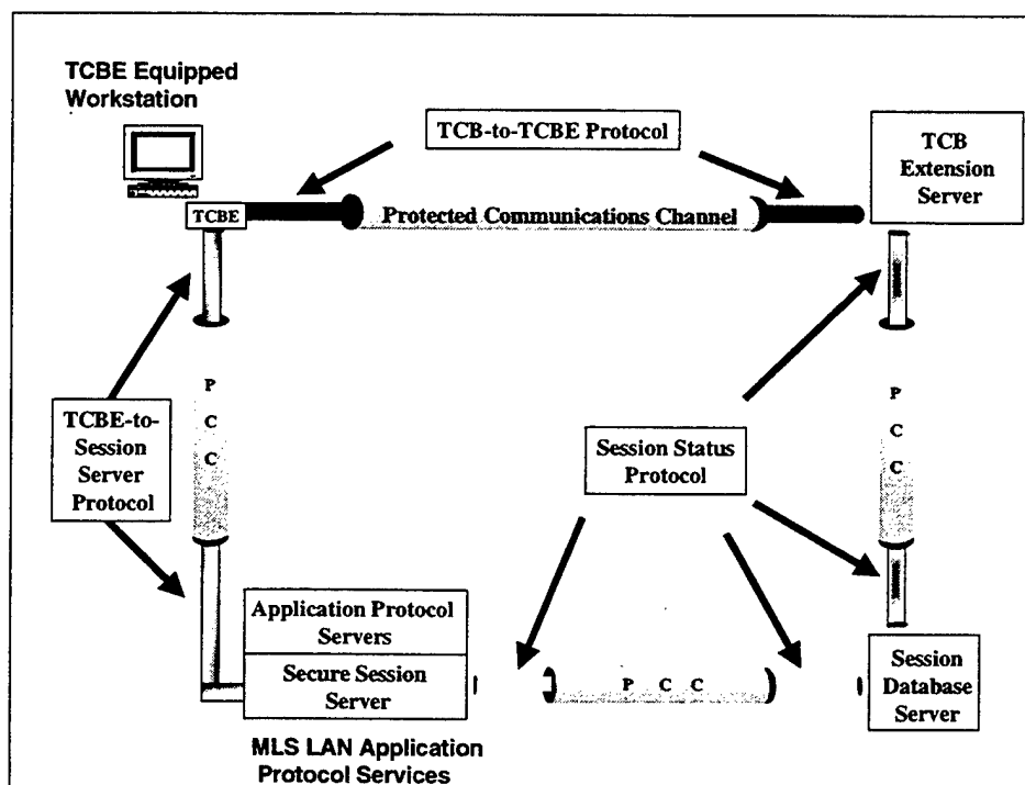
Figure 2.4 MLS LAN Connection Protocols
