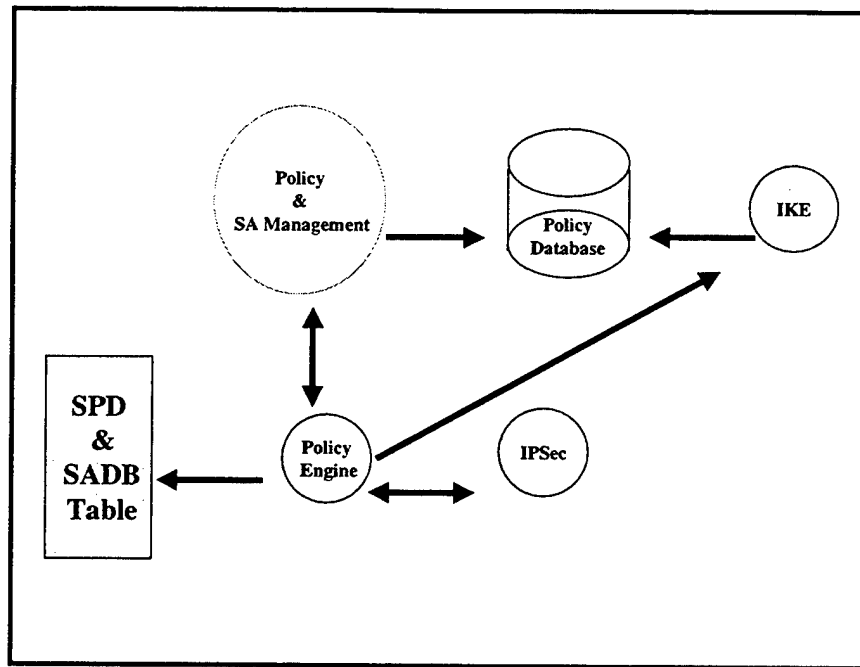
Figure 3.4 IPSec Implementation Architecture, from [Ref. 20]
