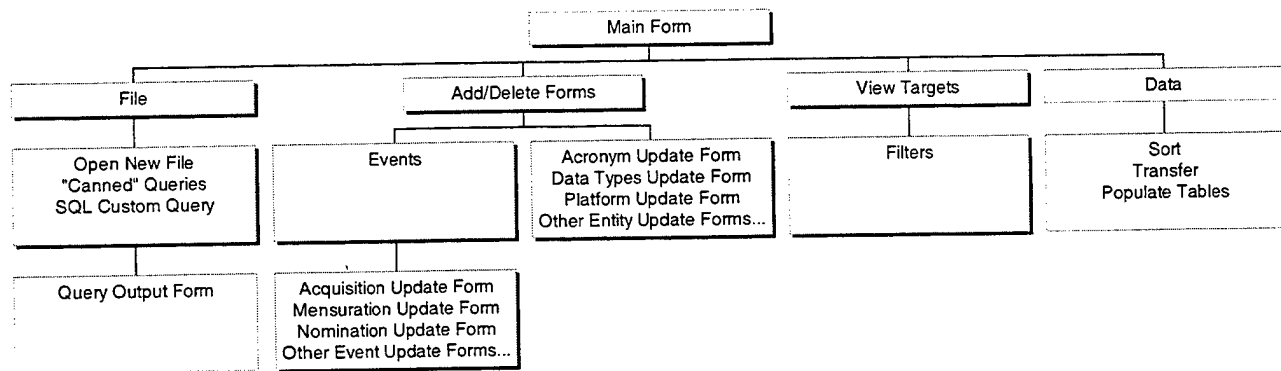
Figure 14 Hierarchical Chart of Menu Options.
