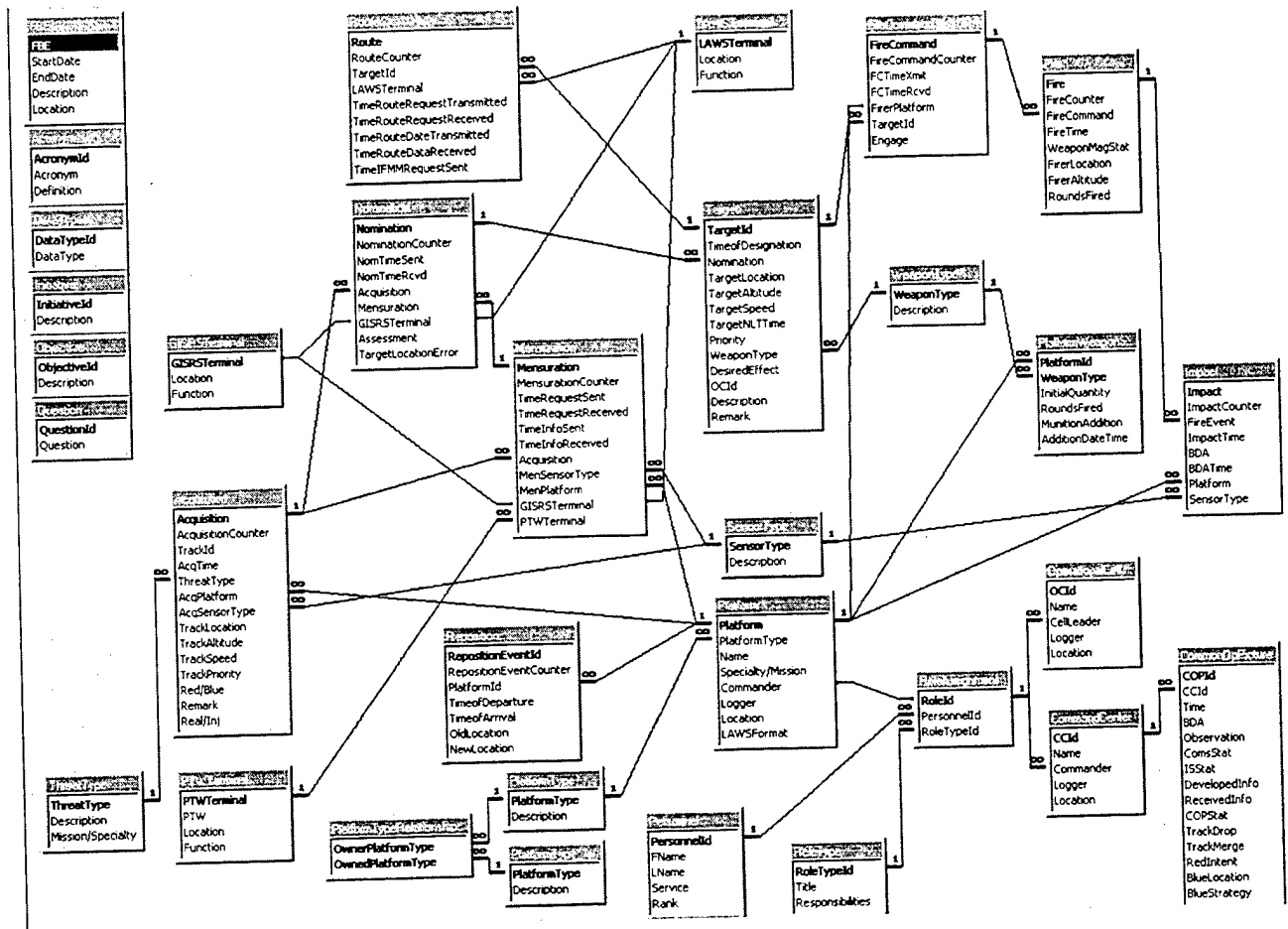
Figure 6 Fleet Battle Experiment Database Schema with All Entities Represented.
