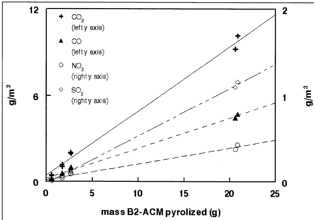
Figure 4. Concentrations of CO 2 , CO, NO 2 , and SO 2 as a function of the mass of B2-ACM pyrolyzed.
