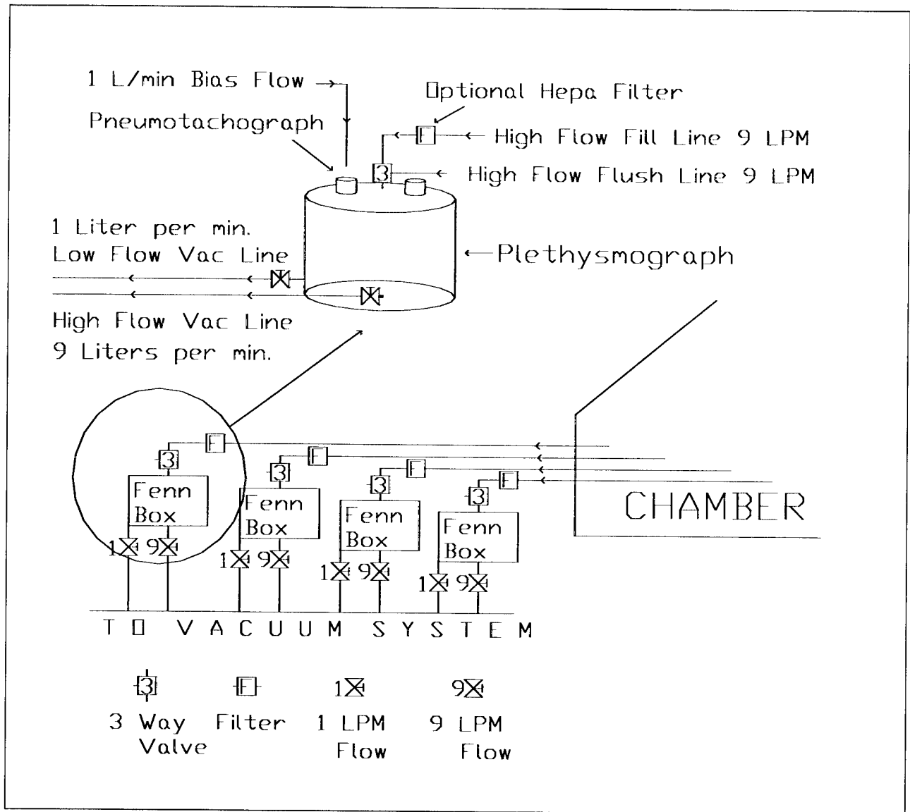
Figure 1. Schematic of the plethysmograph(s)/exposure system.
