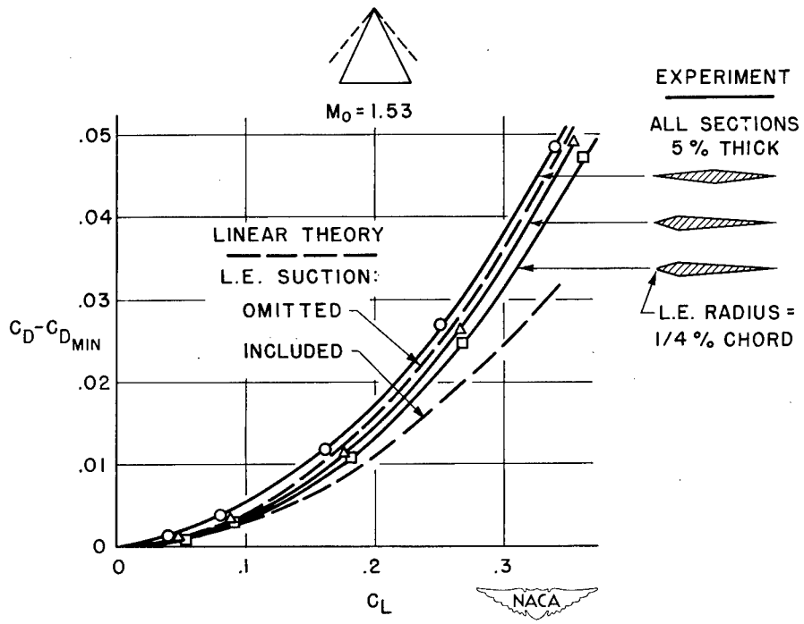
FIGURE 11.- EFFECT OF WING SECTION ON DRAG RISE OF TRIANGULAR WINGS.
