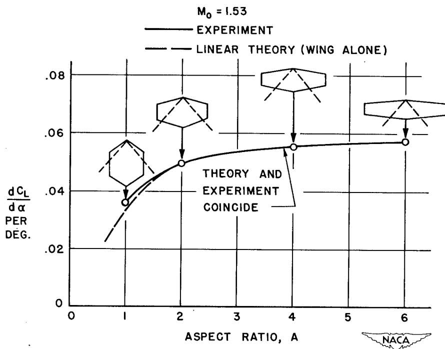
FIGURE 4.— EFFECT OF ASPECT RATIO ON LIFT-CURVE SLOPE.
