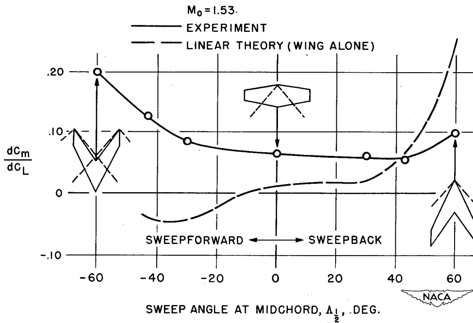
FIGURE 7.— EFFECT OF SWEEP ON MOMENT-CURVE SLOPE.
