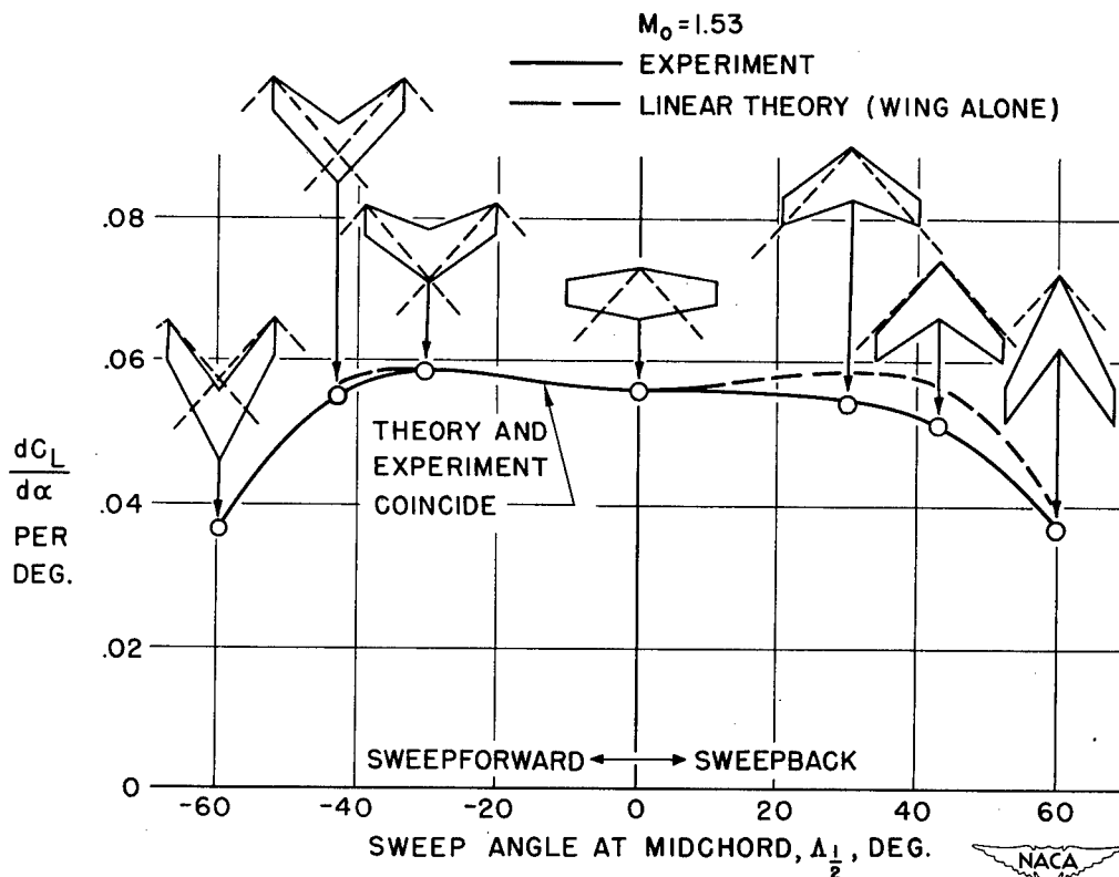
FIGURE 5.— EFFECT OF SWEEP ON LIFT-CURVE SLOPE.
