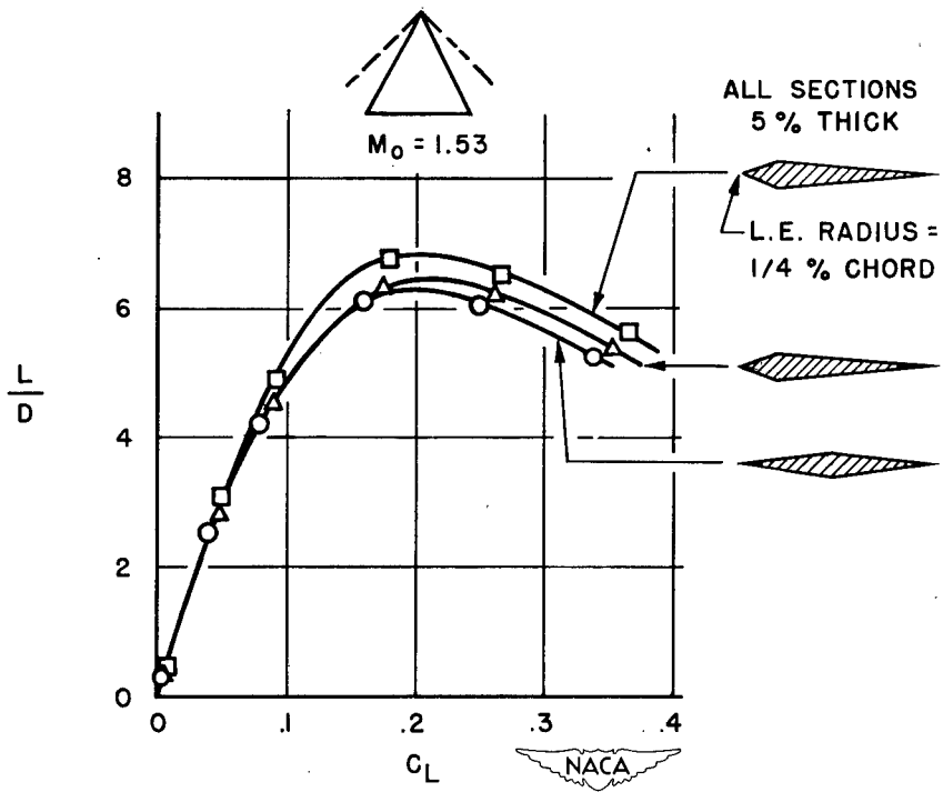
FIGURE 12.- EFFECT OF WING SECTION ON LIFT-DRAG RATIO OF TRIANGULAR WINGS.
