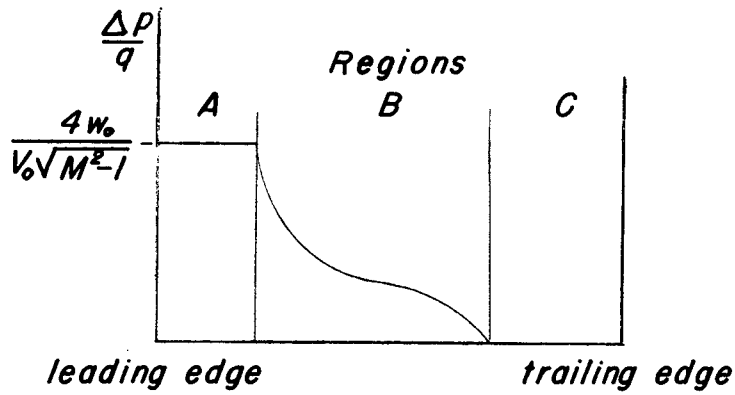
(a) Time interval I, 0 < t/c < 1/(M+1)
