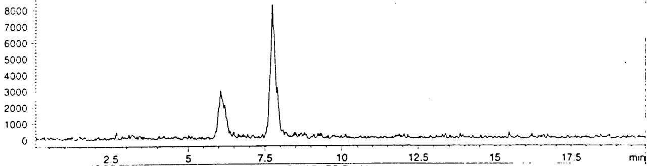
MSD1 434, EIC=433.7:434.7 (D:\072498\JTS00001.D) API-ES Positive
