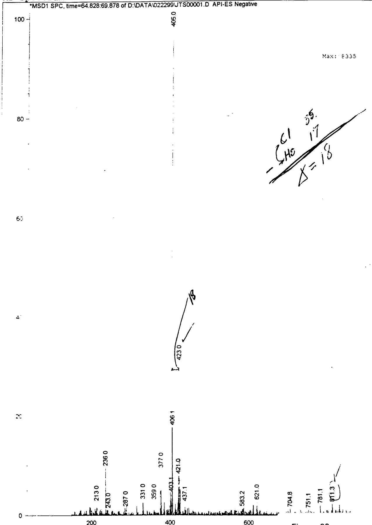
Figure 89 GPC-MS of 3-AT reaction aged MS of 65-70 min fraction
