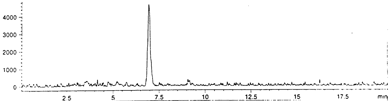
MSD1 377, EIC=376.7:377.7 (D:\072498\JTS00001.D) API-ES Positive
