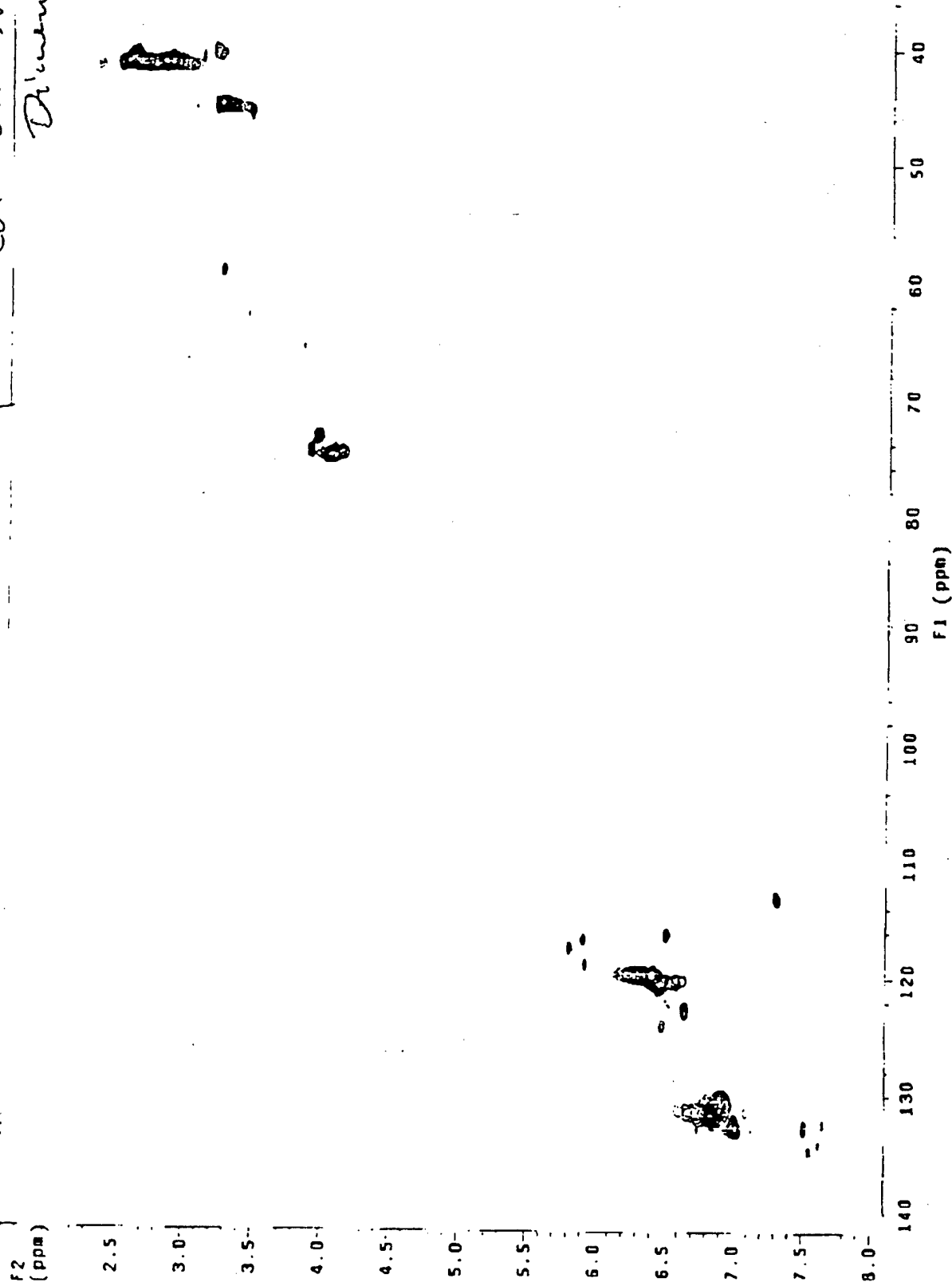
Figure 72 1H -13C HETCOR NMR of p-Tyr 2 f in D 2 O/NaOD 600 MHz NMR
