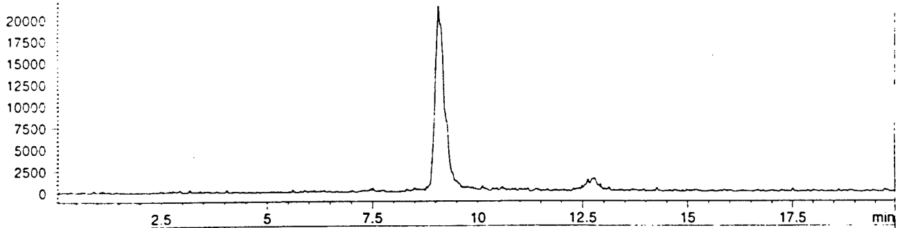
MSD1 491, EIC=490.7:491.7 (D:\072498\JTS00001.D) API-ES Positive
