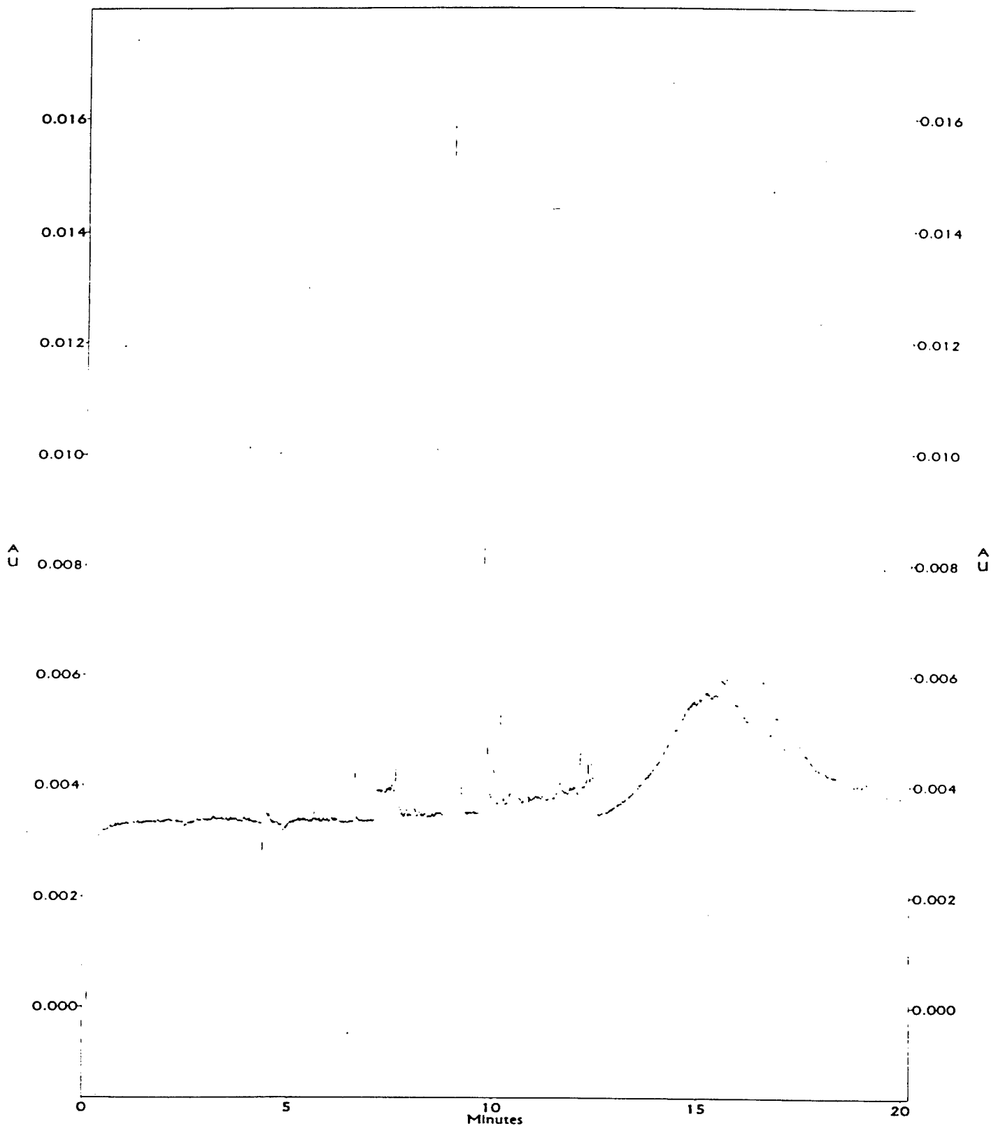
Figure 20 CE of Tyr reaction products 214 nm
