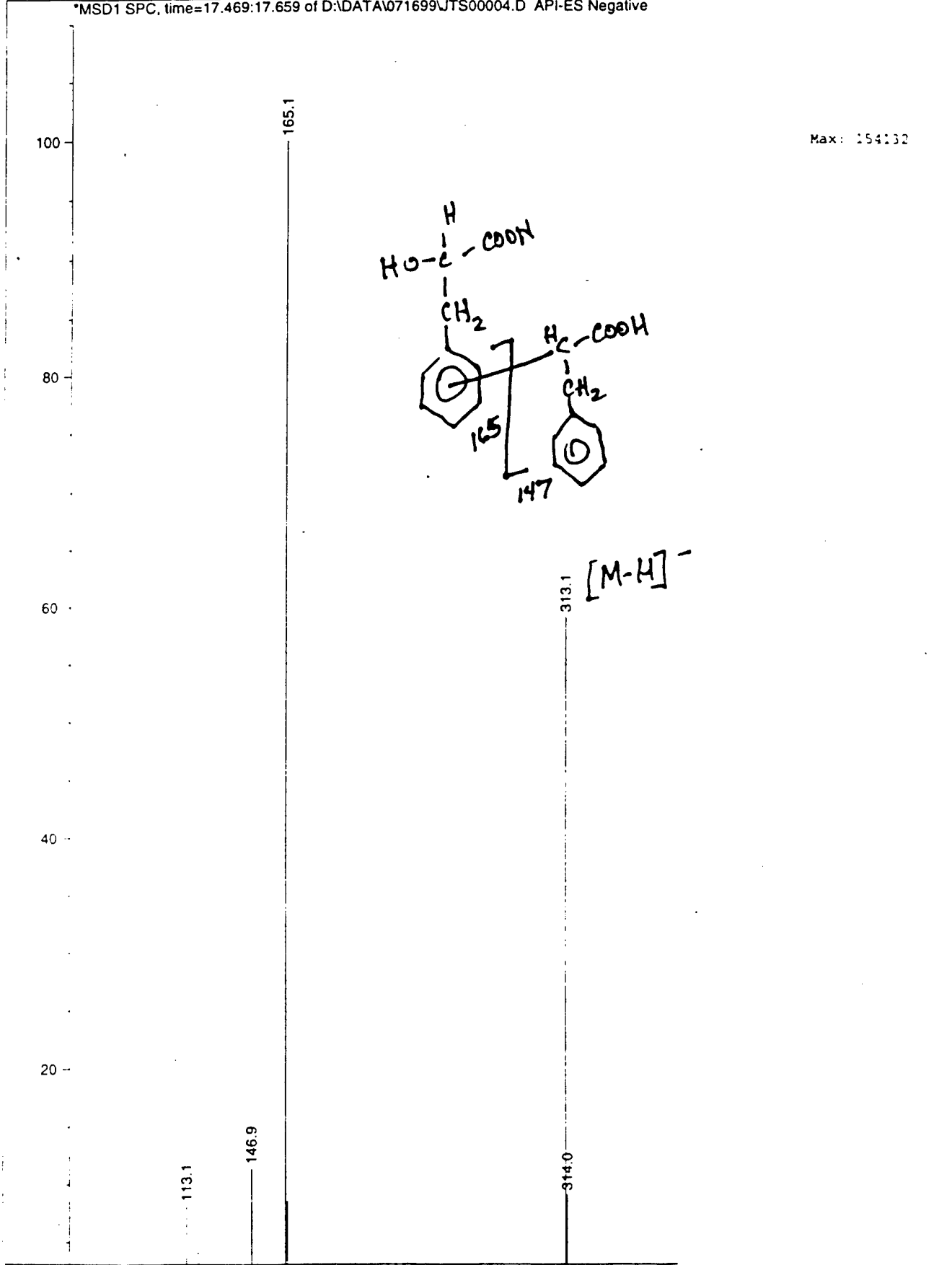
Figure 14 MS of 17.5 min component Phe reaction (-)-ESI
