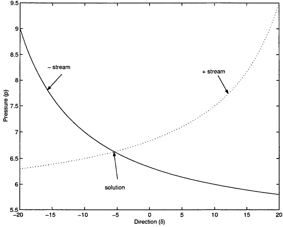
Figure 10. Pressure-Direction Curves Depicting the Riemann Problem
