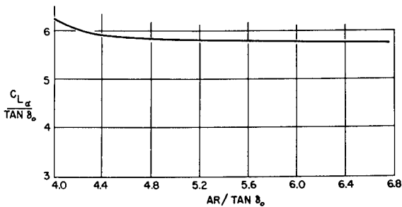
Figure 12.- Lift-curve slope as a function of aspect ratio for swept-back wing at M_0=1 .
