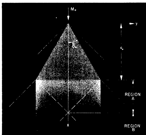
Figure 5.- Triangular wing and wake together with regions used in calculating downwash.
