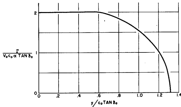
Figure 11.- Spanwise distribution of circulation for swept-back wing at M_0=1 , b=1.325 c_0 \tan \delta_0 and AR=4.57 \tan \delta_0 .
