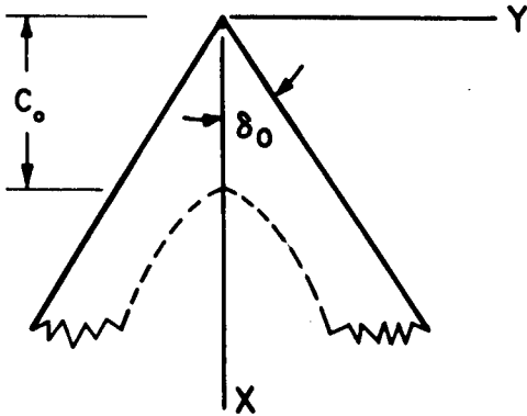
(a) Plan form with arbitrary trailing edge.
