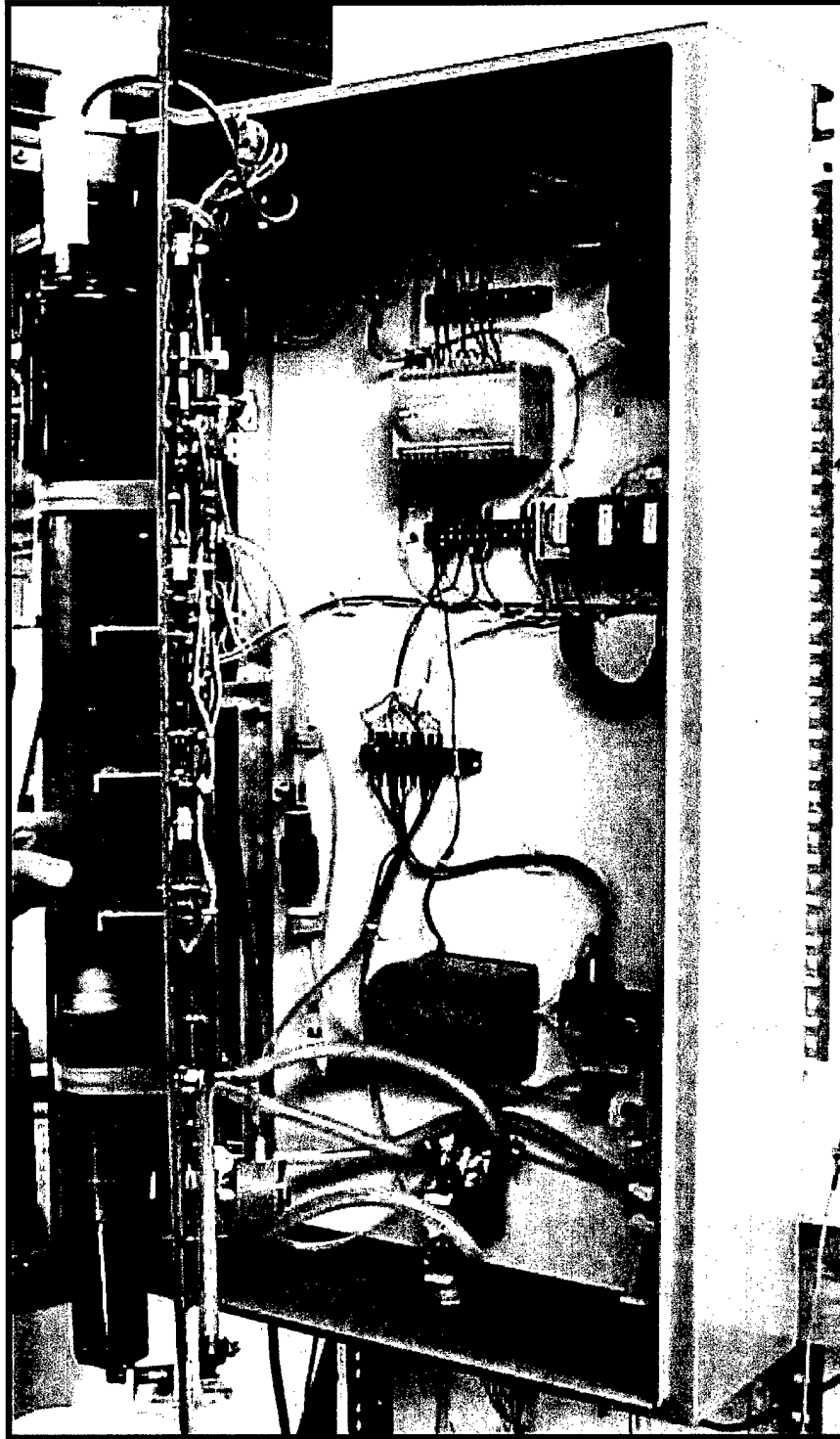
Figure 16. Detail of sub-panel of AFFF sensor.
