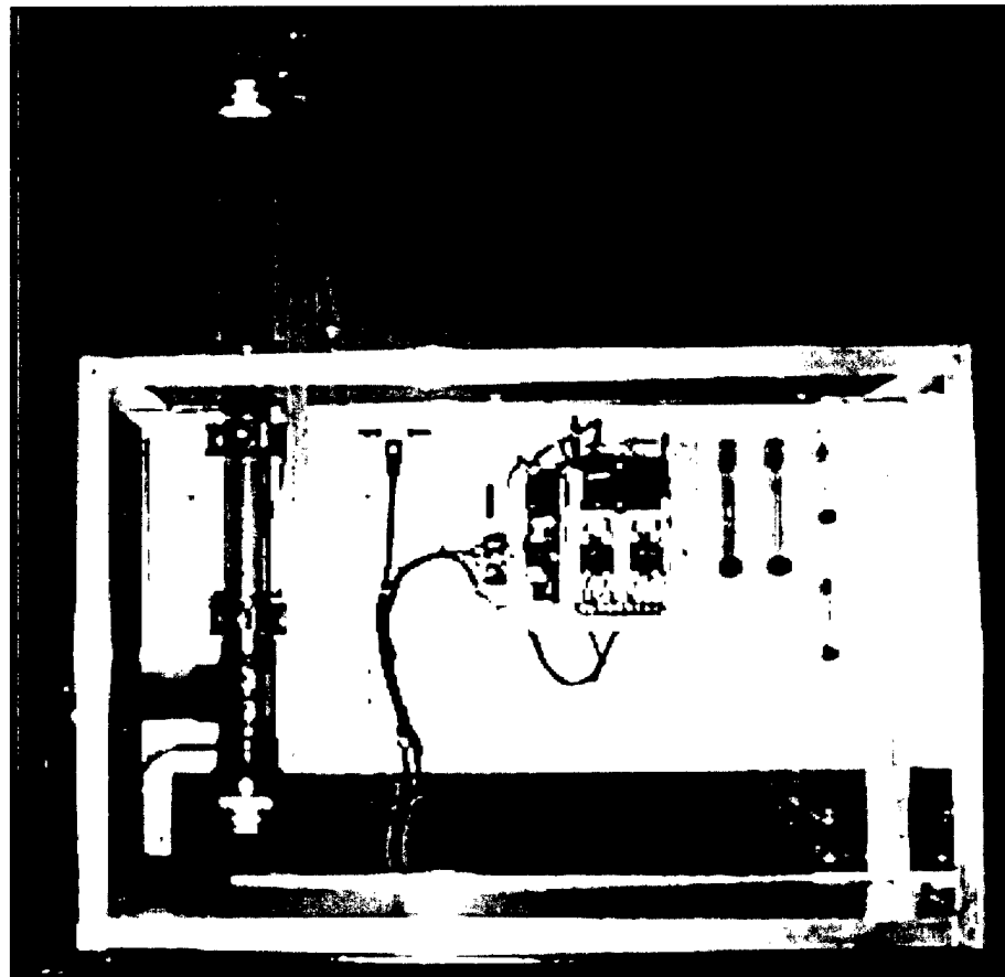
Figure 7. Prototype AFFF sensor system using tank level controller.
