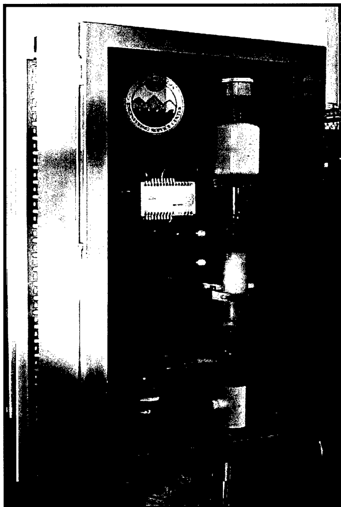
Figure 1. Prototype AFFF sensing unit.
