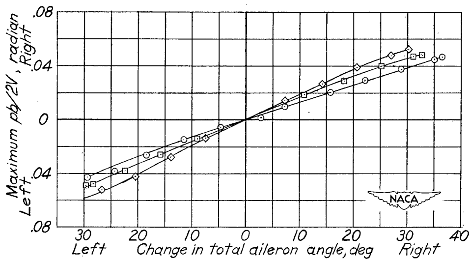
Figure 23.- Variation of aileron stick force and wing-tip helix angle \frac{pb}{2V} with change in total aileron angle in rolls with rudder fixed. Power for level flight; flaps up; nose wheel up.
