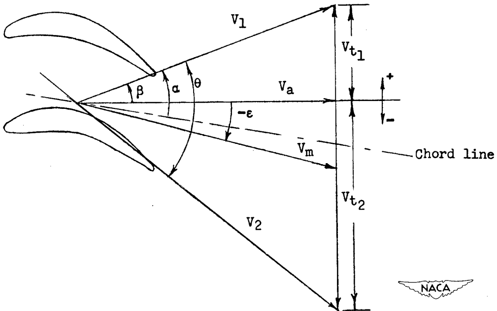
Figure 4.- Velocity diagram.
