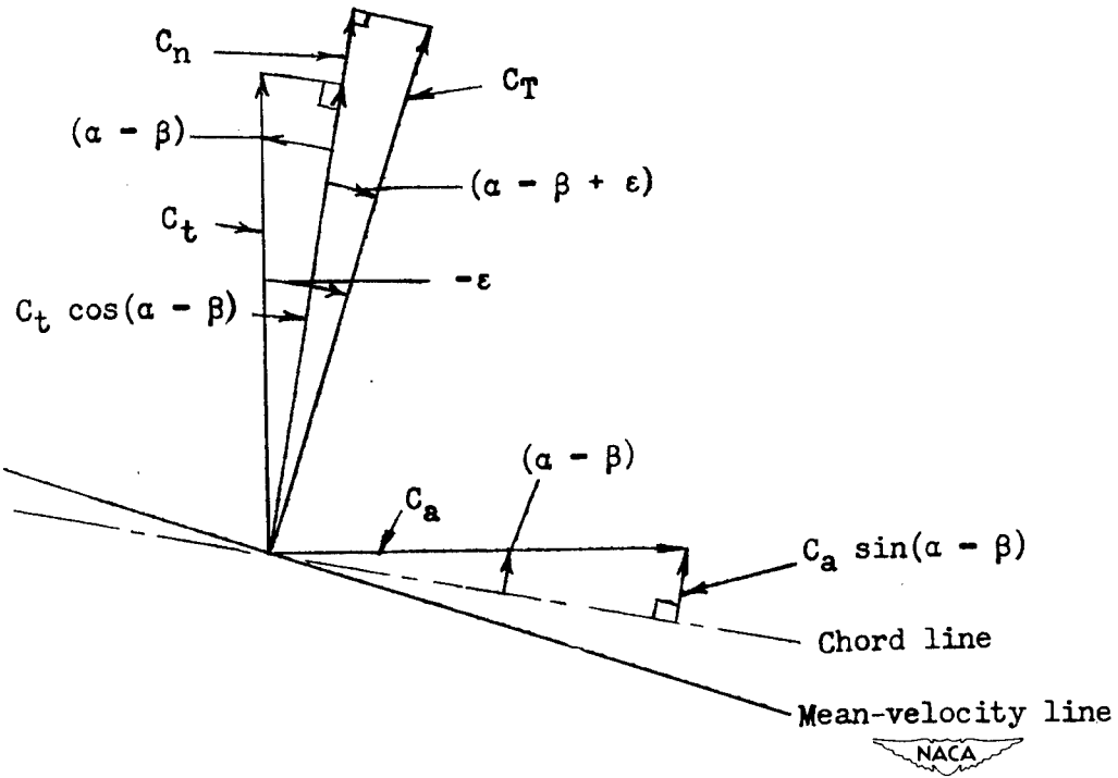
Figure 3.- Force diagram.
