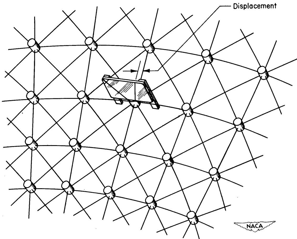
Figure 1.- Wire-mesh alinement.
