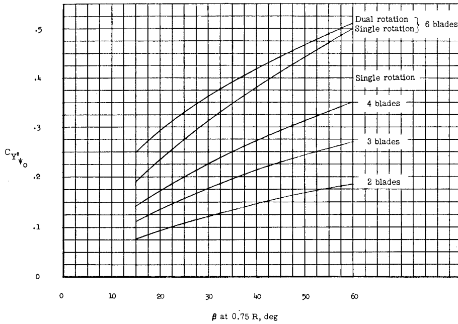
(a) Hamilton Standard 3155-6 propeller with 0.164-diameter spinner; S.F.F. = 80.7.
