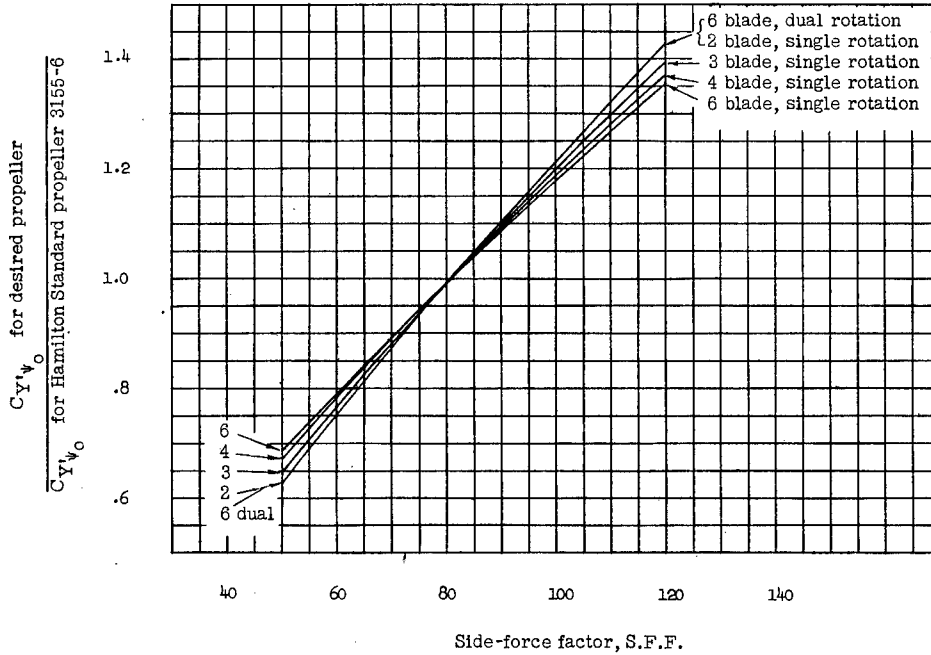
(a) Hamilton Standard propeller 3155-6; S.F.F. = 80.7.
