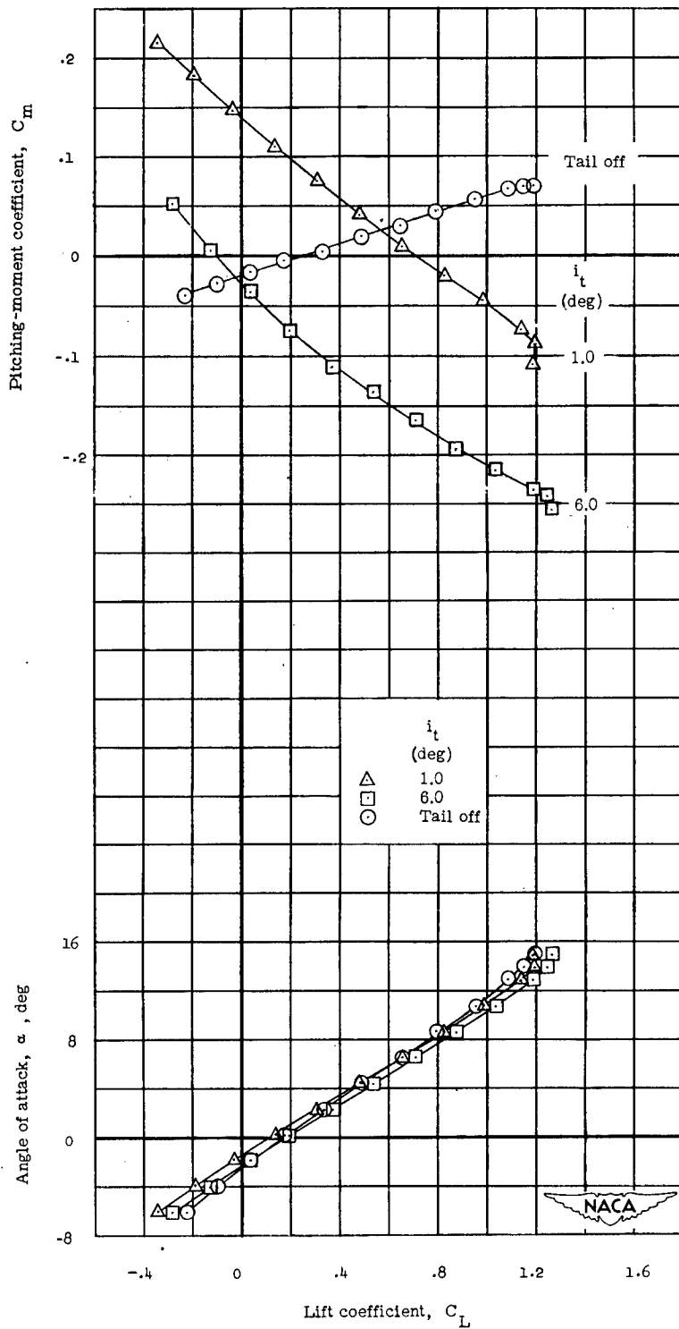
(a) Wind-tunnel data with propeller windmilling.
