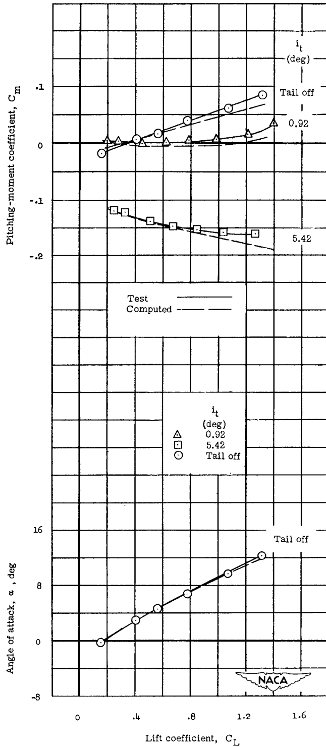
(b) Comparison of computed and experimental data for constant power condition.
