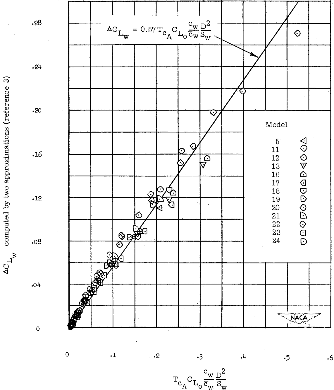
Figure 6.- Variation of the increment of wing lift attributable to the propeller slipstream as computed from two approximations by the method of reference 3 with the parameter T_{c_A} C_{L_o} \frac{c_w D^2}{\bar{c}_w S_w} .
