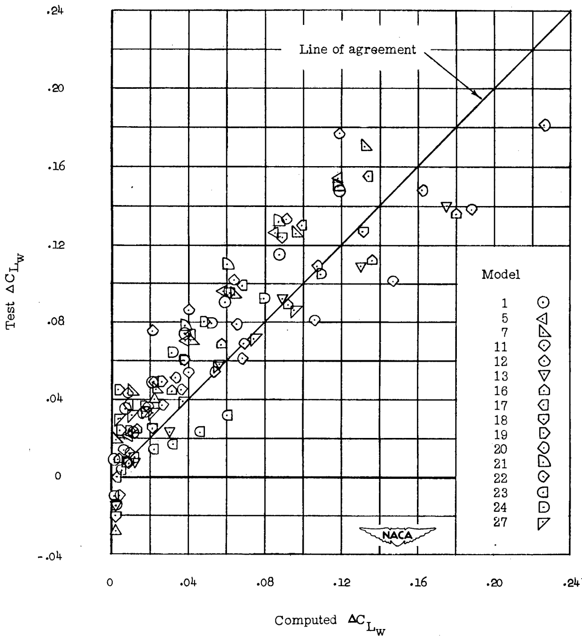
Figure 7.- Comparison of \Delta C_{Lw} computed by equation 3 and obtained from
