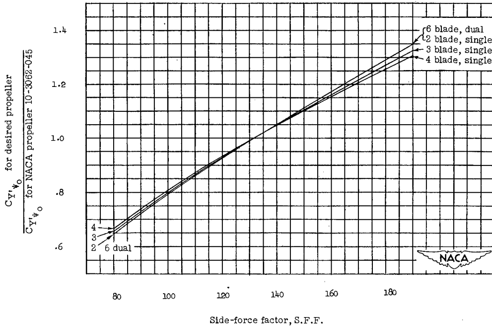
(b) NACA propeller 10-3062-045; S.F.F. = 131.6.
