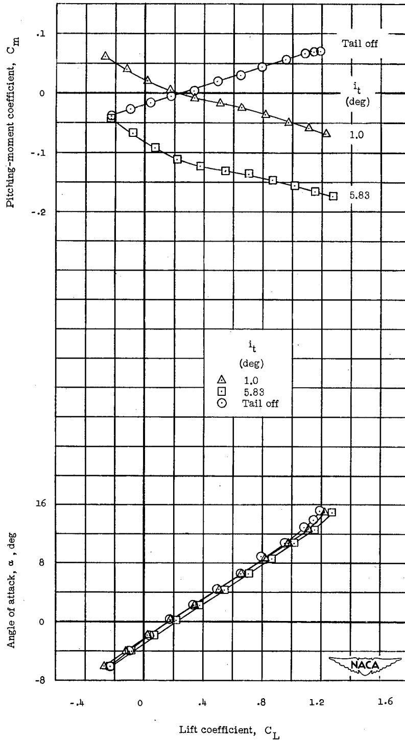
(a) Wind-tunnel data with propeller windmilling.
