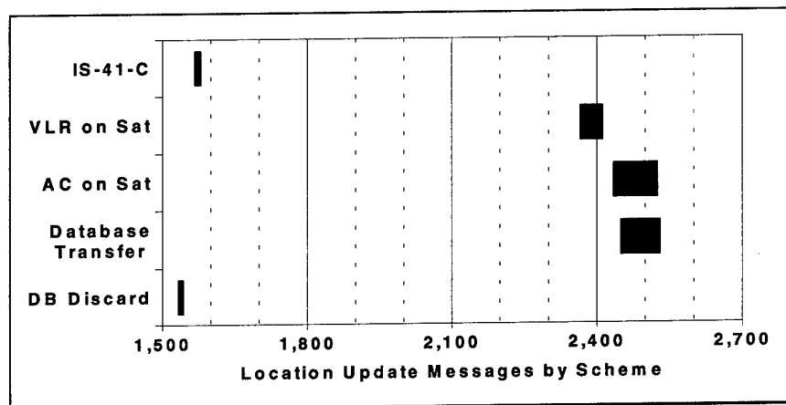
Figure 24. Location Updates (High Load)
