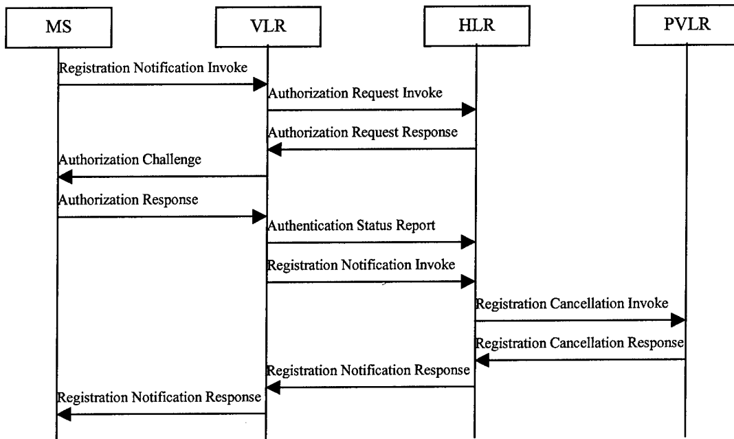
Figure 6. IS-41 Location Update Trace Diagram
