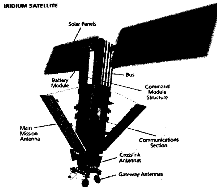
Figure 9. Iridium Satellite
