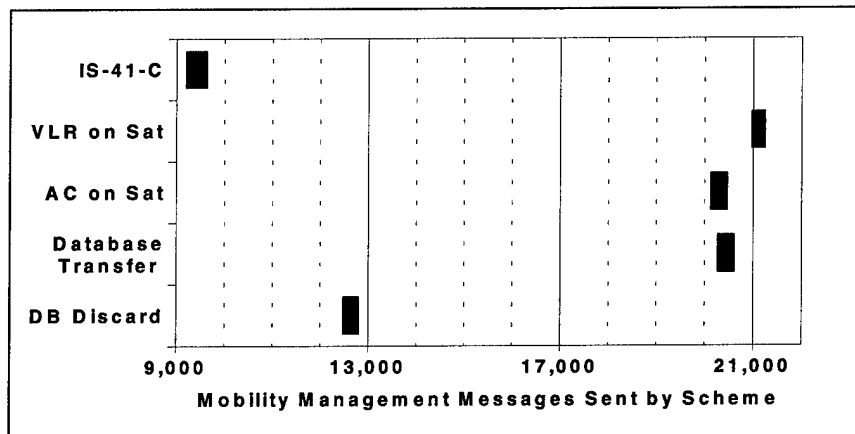
Figure 34. Total Management Messages Sent (Modified Load)
