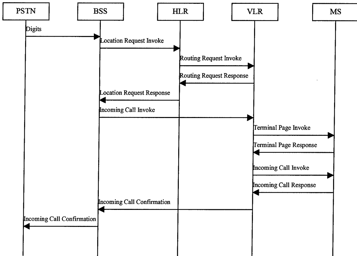
Figure 7. IS-41 PSTN to MS Call Setup
