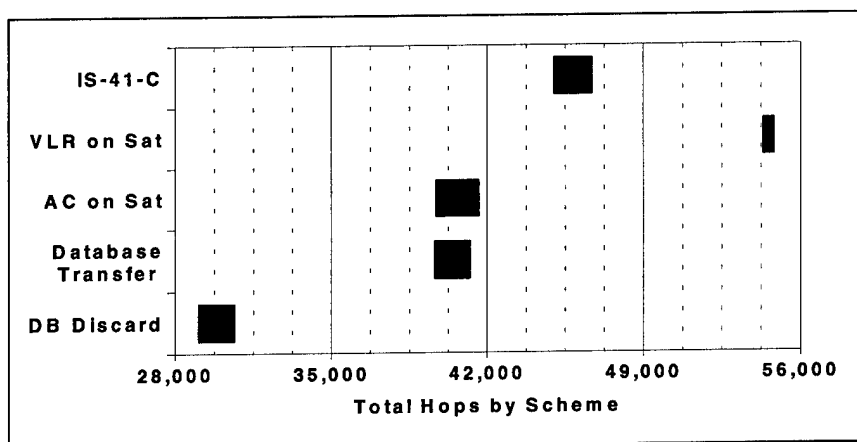
Figure 31. Total Hops (Modified Load)
