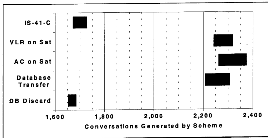
Figure 20. Number of Conversations (Low Load)
