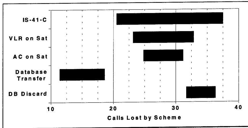
Figure 28. Number of Lost Calls (Modified Load)
