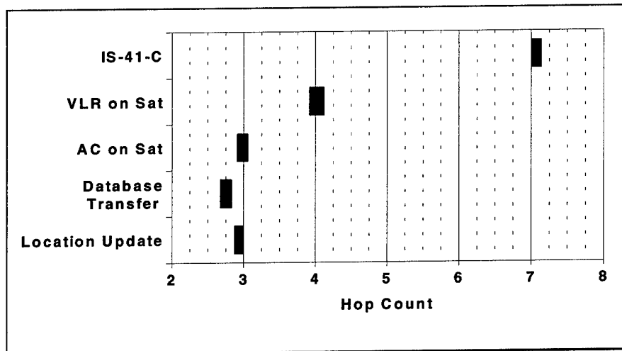
Figure 17. Average Number of Hops (Low Load)
