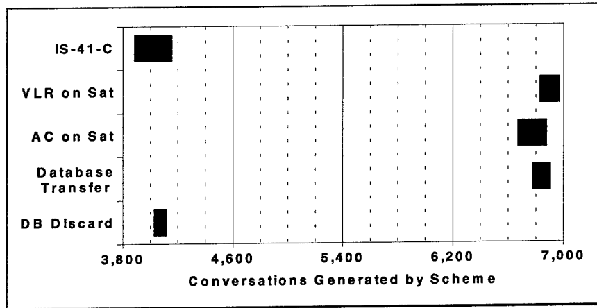
Figure 22. Number of Conversations (Modified Load)
