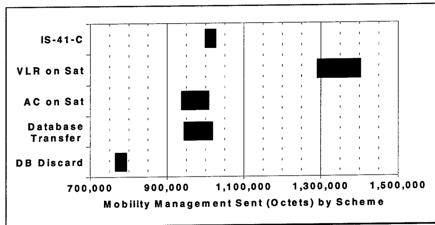
Figure 35. Total Management Bytes Sent (Low Load)
