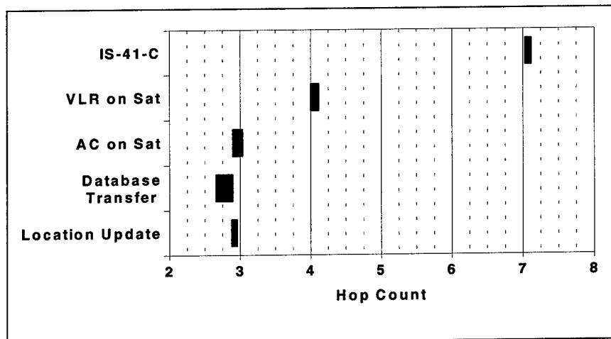
Figure 18. Average Number of Hops (High Load)
