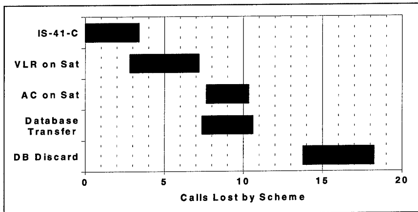
Figure 27. Number of Call Lost (High Load)
