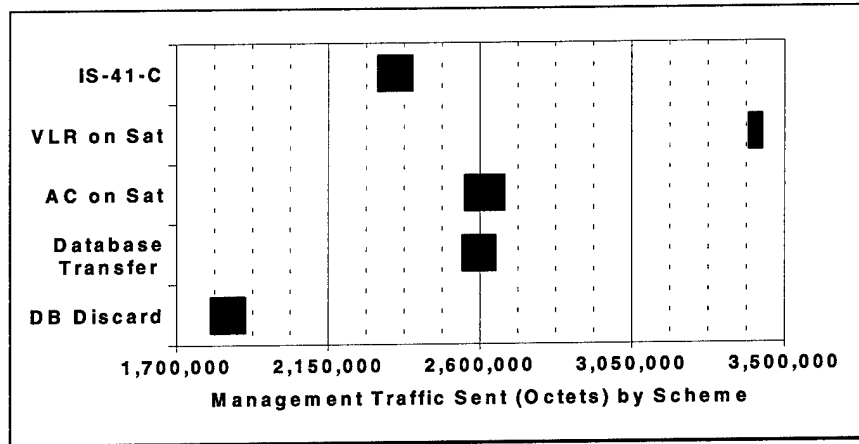
Figure 37. Total Management Bytes Sent (Modified Load)
