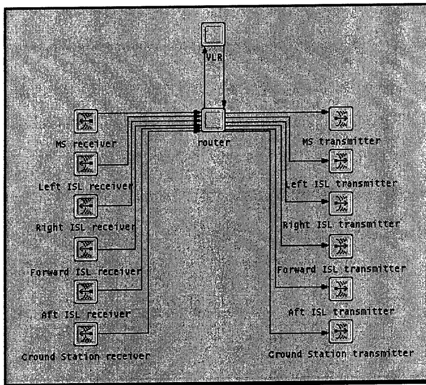
Figure 16. The Enhanced Iridium ® Satellite Model
