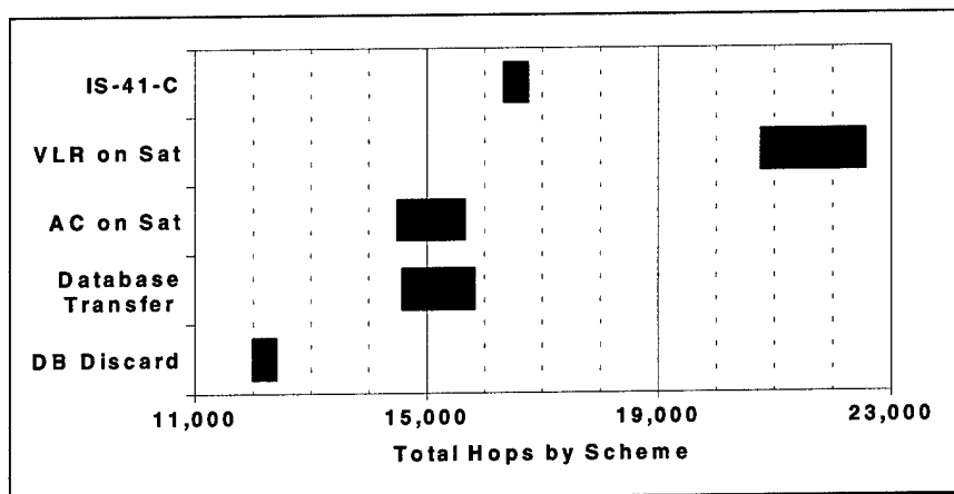
Figure 29. Total Hops (Low Load)
