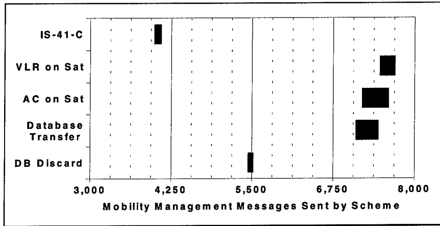
Figure 32. Total Management Messages Sent (Low Load)
