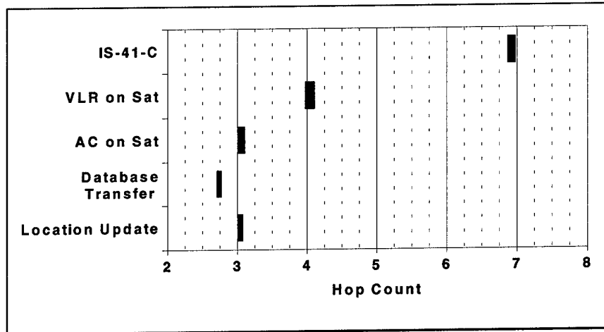
Figure 19. Average Number of Hops (Modified Load)
