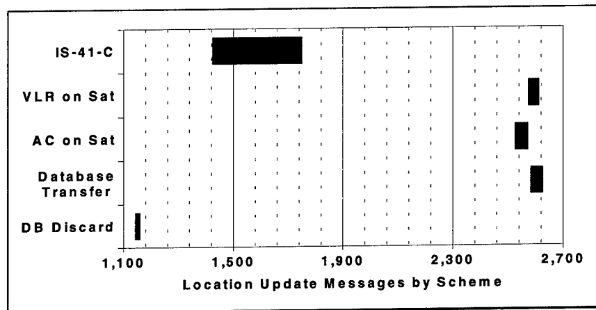
Figure 25. Location Updates (Modified Load)
