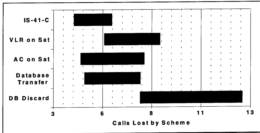
Figure 26. Number of Calls Lost (Low Load)
