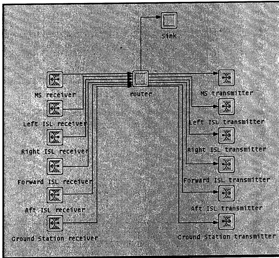
Figure 15. The Standard Iridium ® Satellite Model
