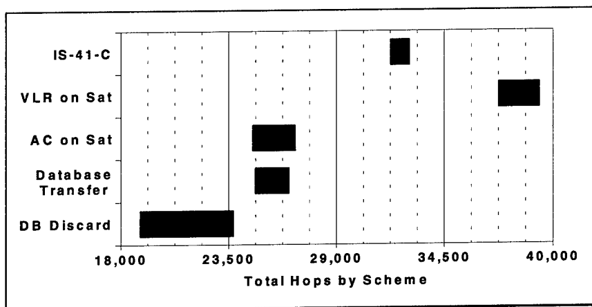
Figure 30. Total Hops (High Load)
