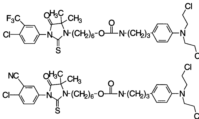
Figure 1. Phenylthiohydantoin linked aniline mustard compounds.
