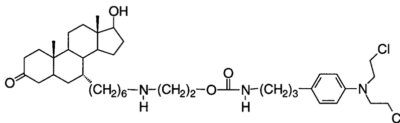
Figure 3. Structure of the 7α-DHT-linked aniline mustard.
