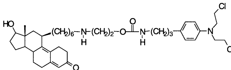
Figure 4. Bifunctional, 11β-4,9-estradien-3-one C6NC2-mustard compound that binds to the AR.
