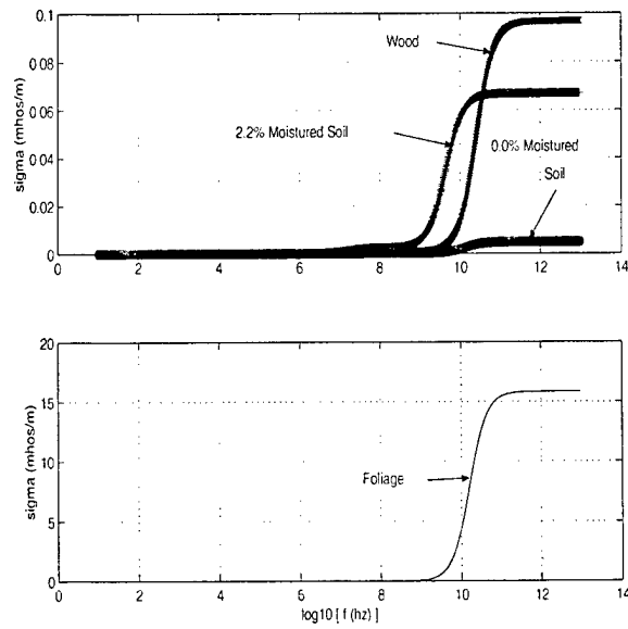
Figure 4: \sigma in the complex permittivity.
