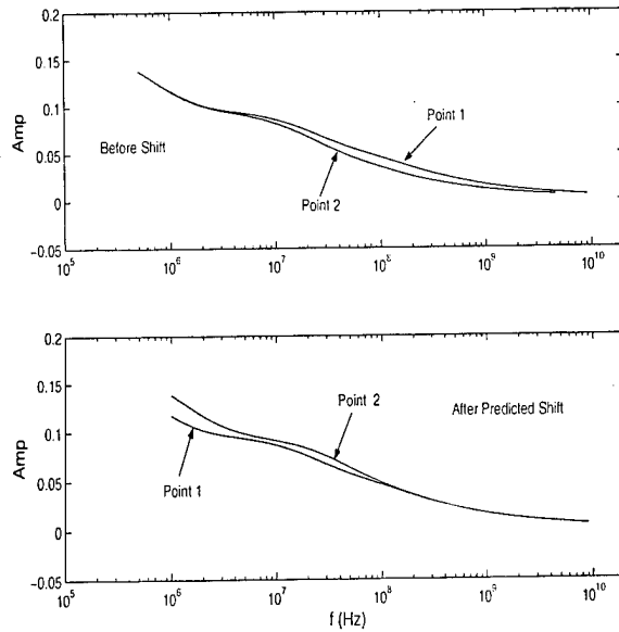
Figure 5: The Dispersive Case. Top: |F(\omega, x, y)| and |F(\omega, x_\lambda, y_\lambda)| , \lambda = 2 . Bottom: |F(\omega, x, y)| and |F(\frac{\omega}{\lambda}, x_\lambda, y_\lambda)| .
