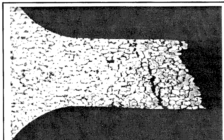
Figure 7 - Intergranular creep failure in nickel superalloy
