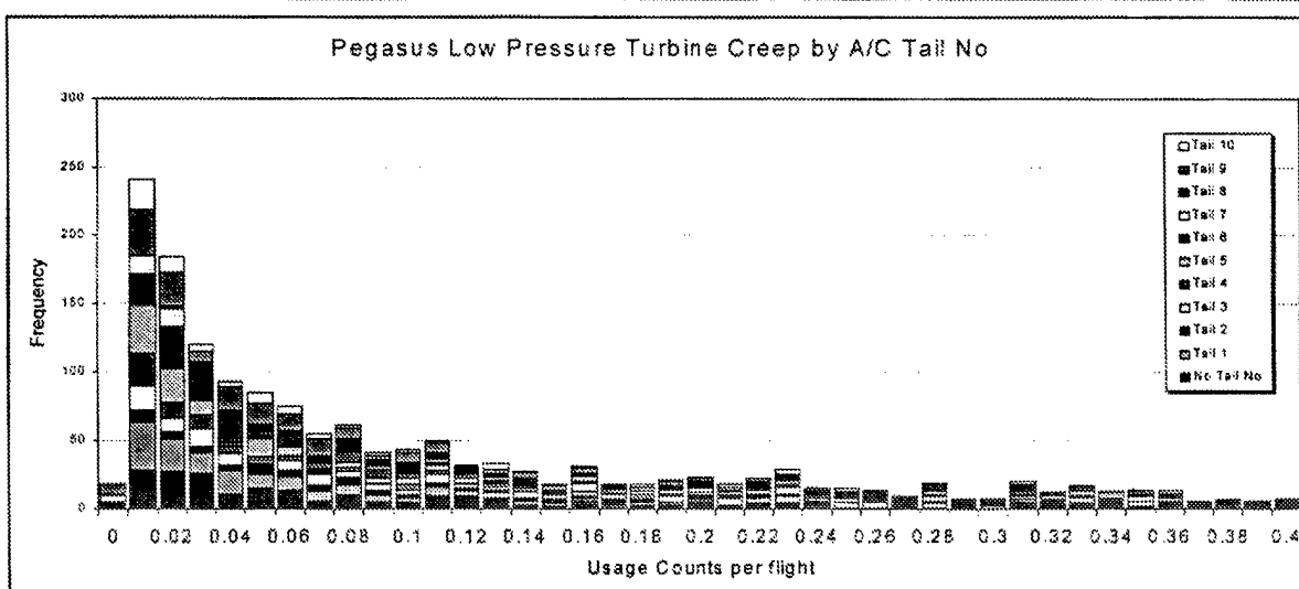
Figure 4 – Pegasus lp turbine blade creep life counts
