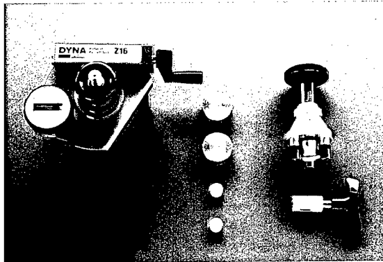
Fig. 10 – Portable adhesion testers with pull-off coupons: L) Dyna tester, R) Elcometer.
