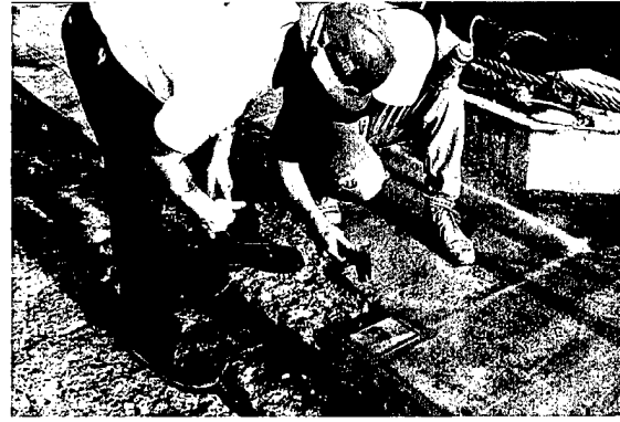
Fig. 14 – Sounding for delaminations.
