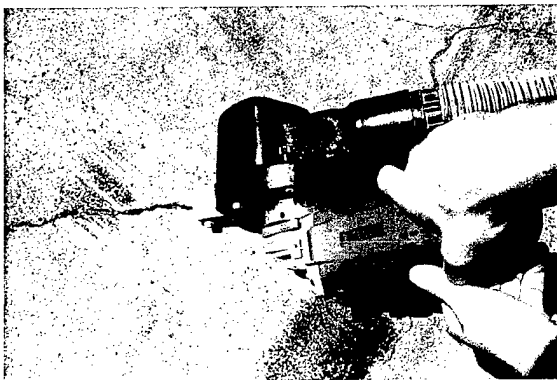
Fig. 15 – Chasing a crack.
