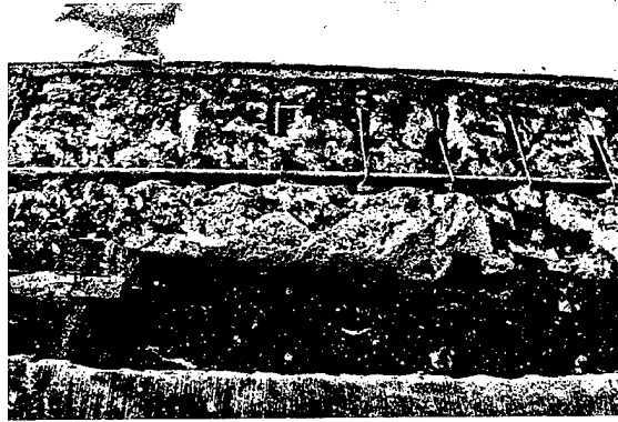
Fig. 16 – Grit blasted reinforcing steel.
