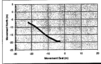
Cloud Centroid Movement During the First 60 Minutes after Release
