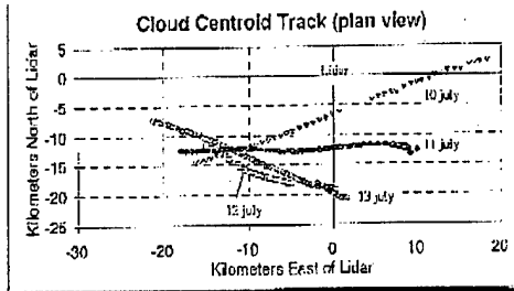
Cloud Centroid Movement During the First 60 Minutes after Release
