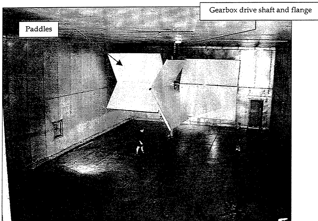
Photograph 1 Tuner assembly
