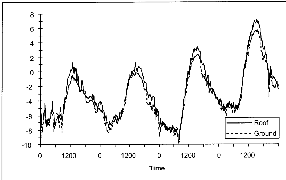
Figure 16. CSU Atmospheric Science Department air temperatures recorded by PRT for the period 29-31 January 2000.
