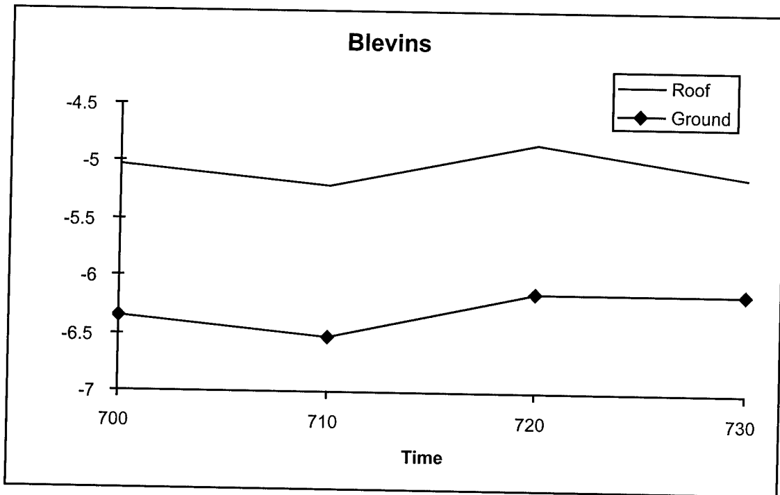
Figure 10. Blevins Junior High School morning air temperatures recorded by PRT for 13 January 2000.
