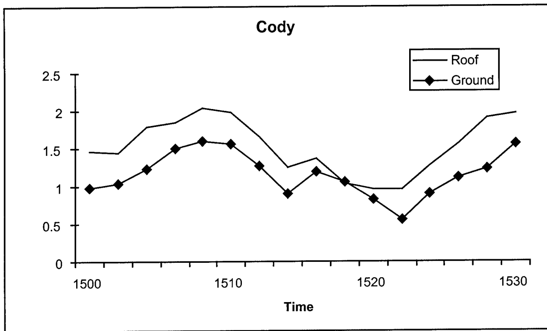
Figure 14. Cody Police Building air temperatures recorded by PRT on 20 January 2000.
