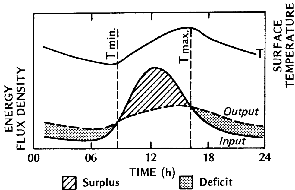
Figure 3. Relationship between surface temperature and surface energy flux where \text{Output} = K\uparrow + L\uparrow , \text{Input} = K\downarrow + L\downarrow , and Q^* = \text{Input} - \text{Output} . From Oke, 1978.
