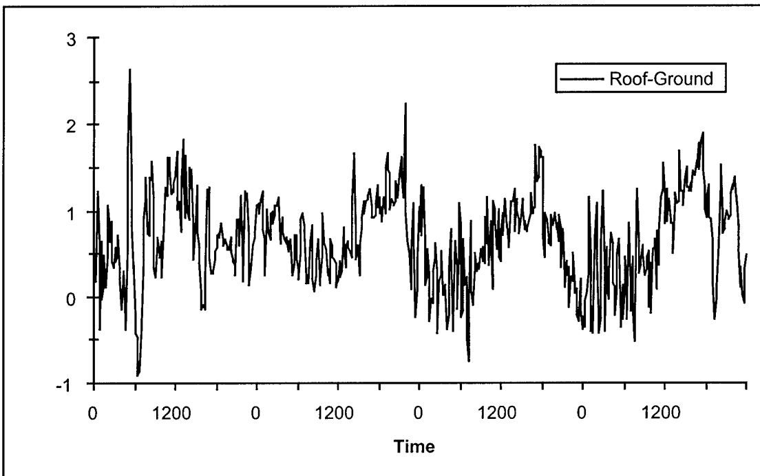
Figure 17. CSU Atmospheric Science Department air temperature differences (roof-ground) for the period 29-31 January 2000.
