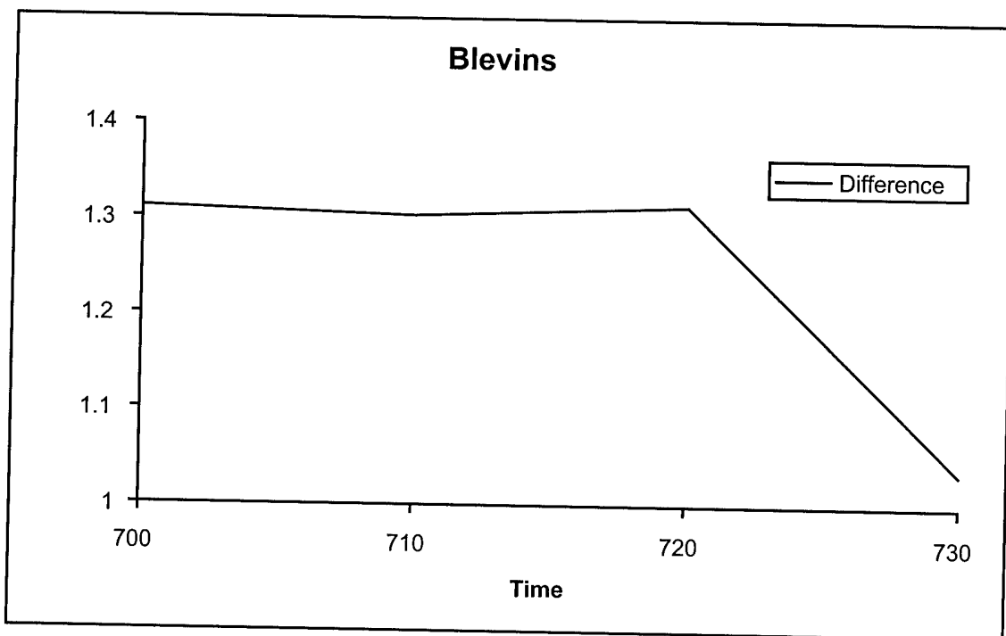
Figure 11. Blevins Junior High School morning air temperature differences (roof-ground) for 13 January 2000.
