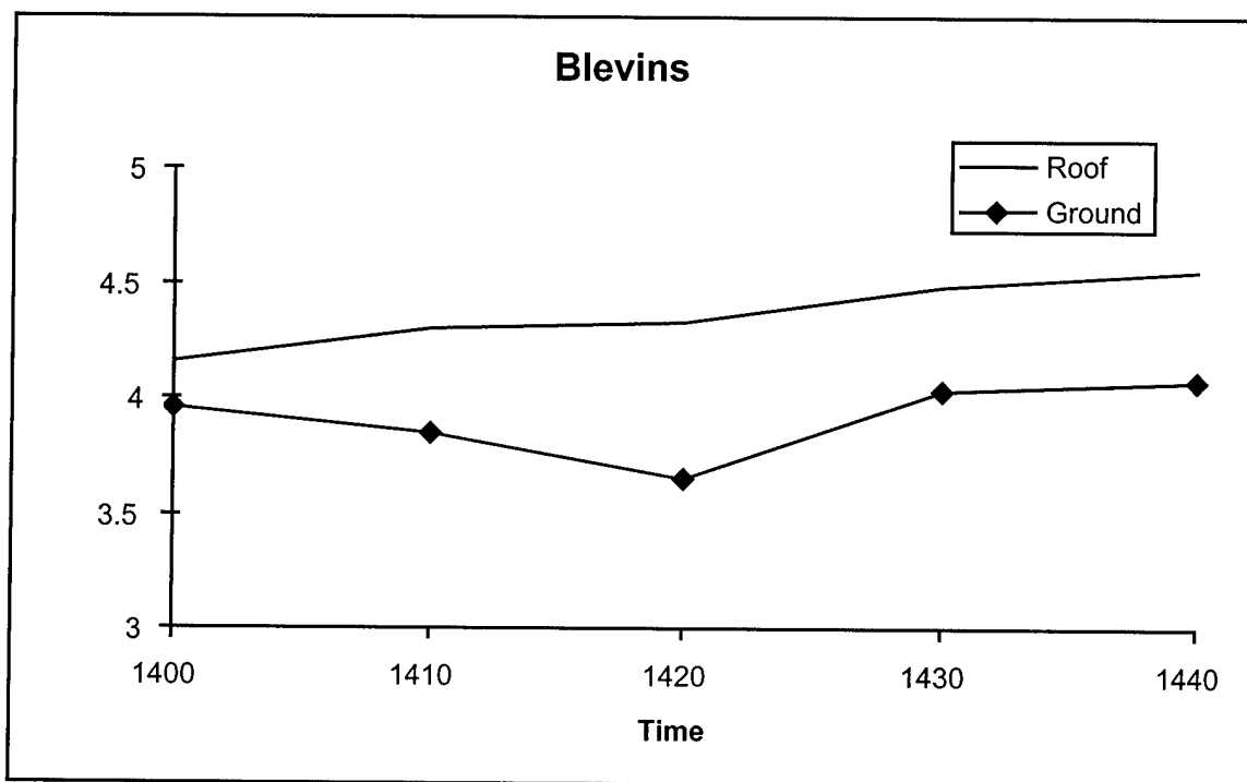
Figure 12. Blevins Junior High School afternoon air temperatures recorded by PRT for 13 January 2000.
