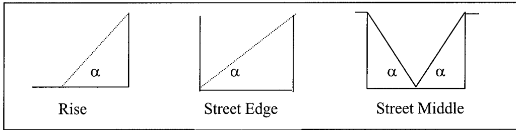
Figure 5. Common sky-view restrictions. Modified from Geiger, 1966.
