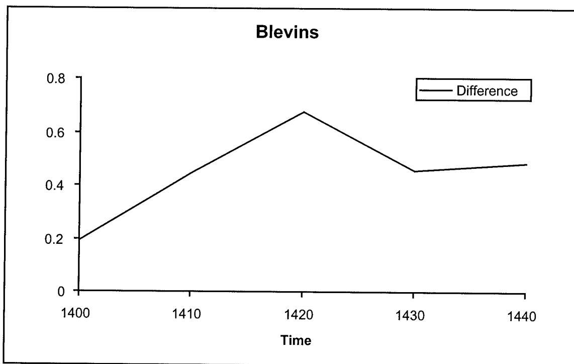
Figure 13. Blevins Junior High School afternoon air temperature differences (roof-ground) for 13 January 2000.
