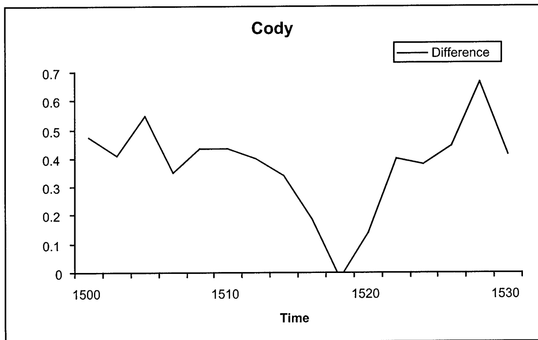
Figure 15. Cody Police Building air temperature differences (roof-ground) on 20 January 2000.
