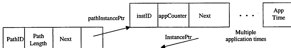
Figure 13: PathDB Module Initialization
