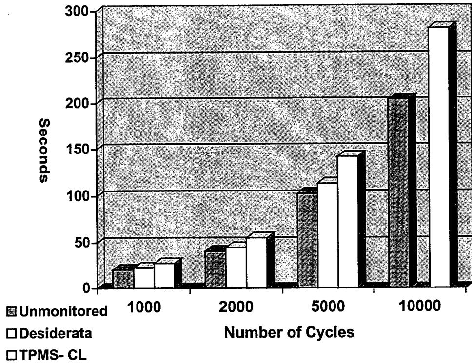
Figure 15. DynBench Overhead in Desiderata and TPMS
