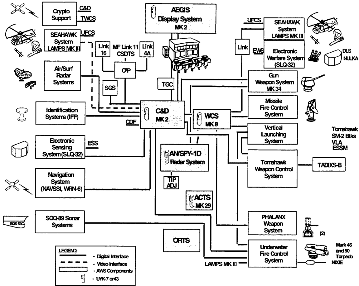
Figure 3. AEGIS Architecture [PERR98]
