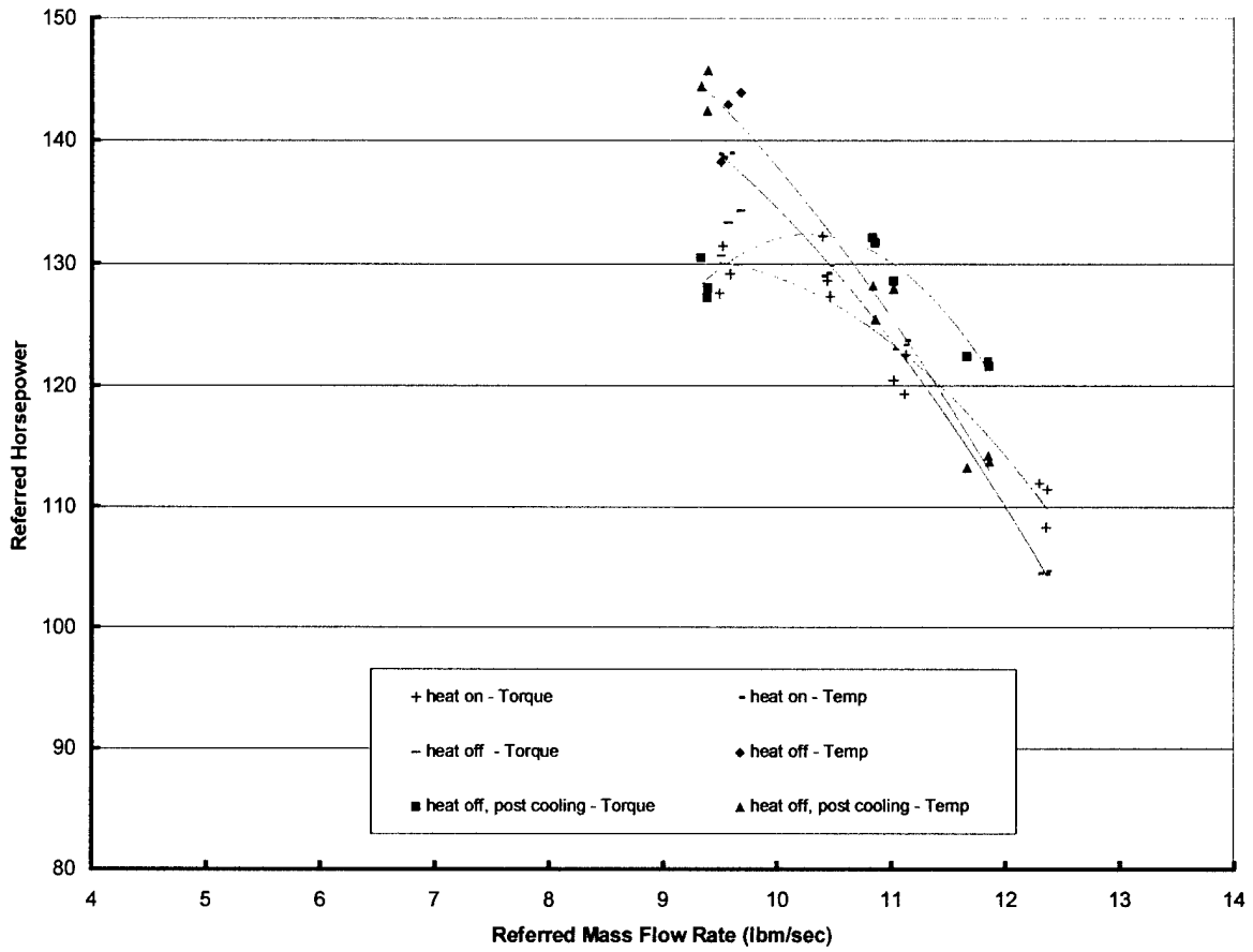
Figure 27. Referred Horsepower vs. Referred Mass Flow Rate Effect of Casewall Temperature
