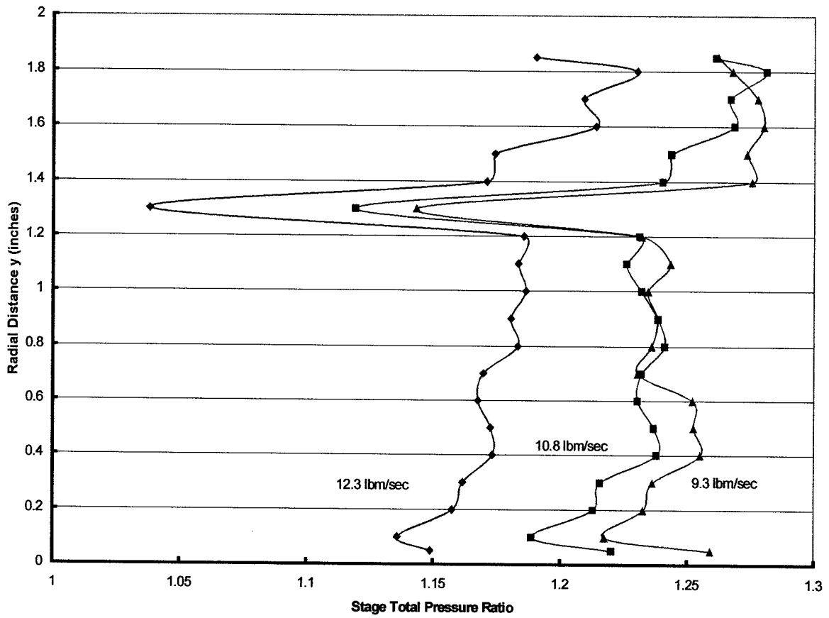
Figure 30. Exit Stagnation Pressure Distribution at 70% Speed
