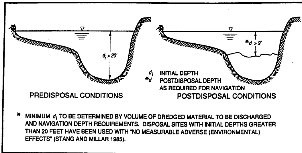
Figure 3. Section view of disposal site
