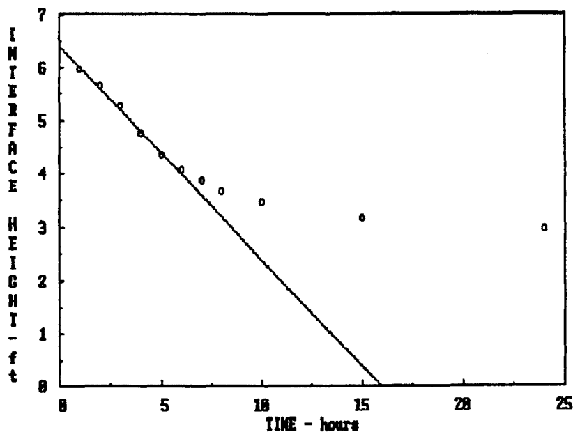
Figure 4. Example plot of zone settling data
