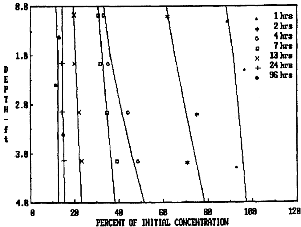
Figure 3. Example plot of flocculent settling data
