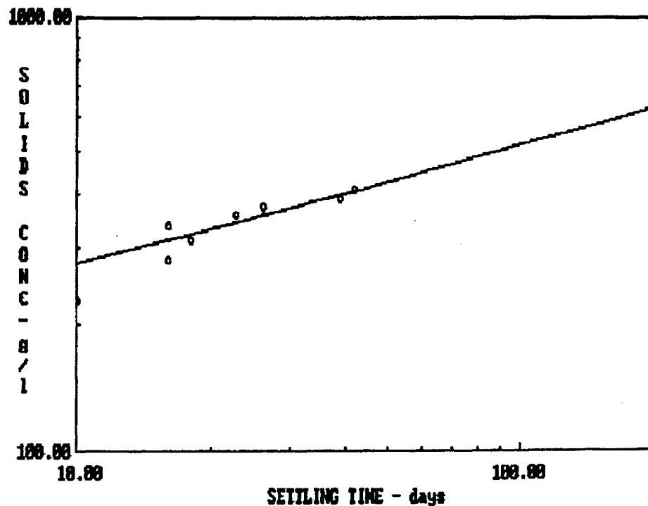
Figure 2. Example plot of compression settling data
