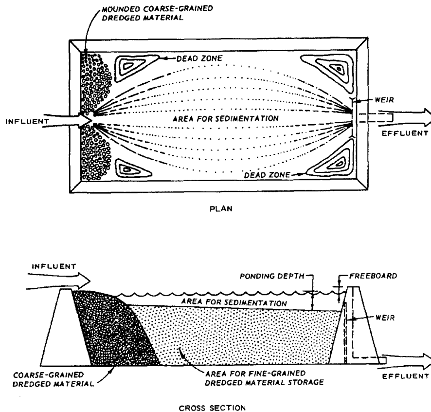
Figure 1. Schematic of a confined disposal facility
