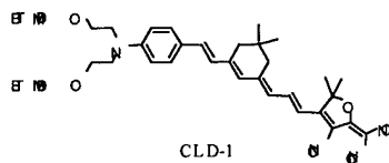
CLD-1 Tri-cyano dye
