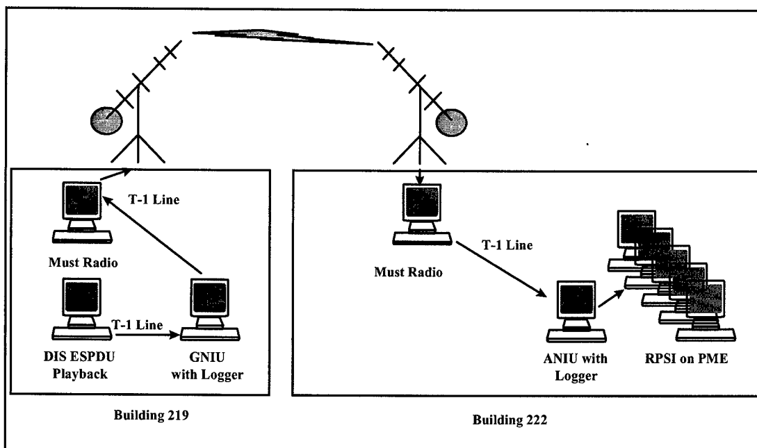
Figure 8. Laboratory PME Test of ANIU and RPSI
