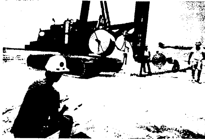
Figure 1. Typical vertical strip drain installation equipment
