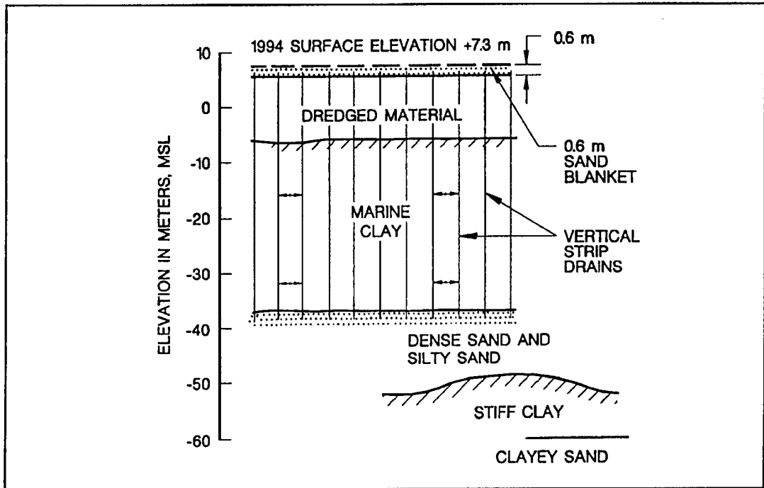
Figure 5. Radial drainage pattern using vertical strip drains
