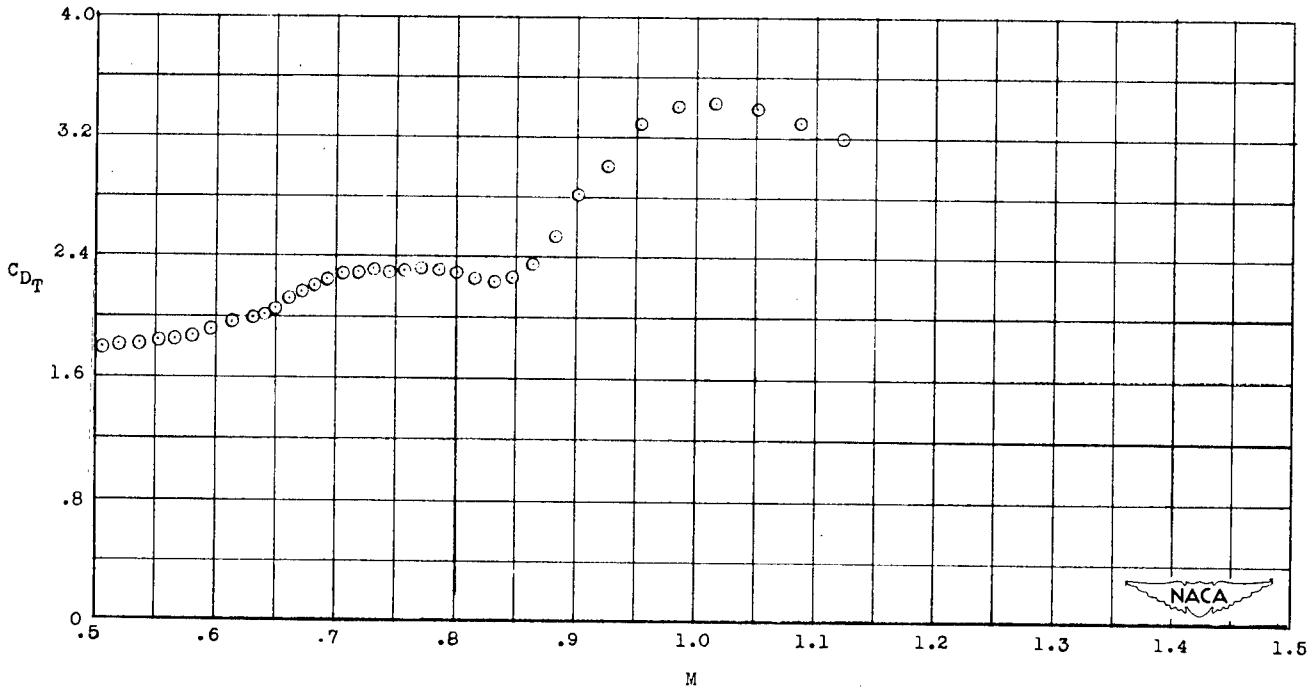
Figure 4.- Variation of total drag coefficients with Mach number for a typical cylinder configuration showing data points. n = 30 ; D = 1 inch.
