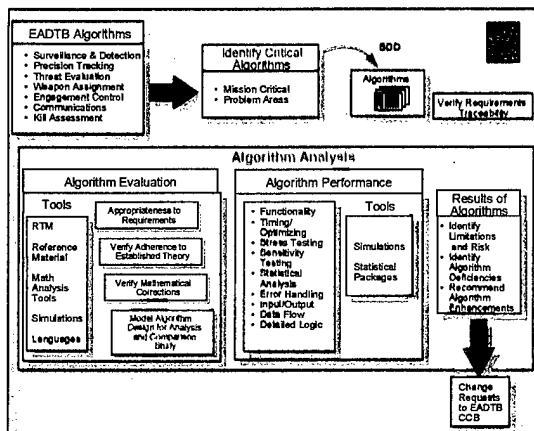
FIGURE 5.2-1 ALGORITHM ANALYSIS
