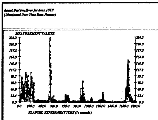
FIGURE 5.3-5 ACTUAL POSITION ERROR FOR HIGH MANEUVERING, HIGH PROCESS NOISE TARGET TRACK
