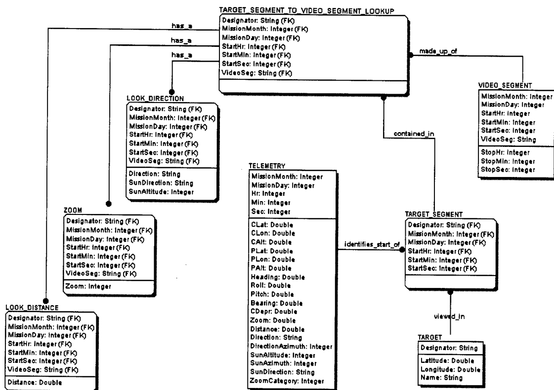
Figure 11: Entity-Relationship Diagram
