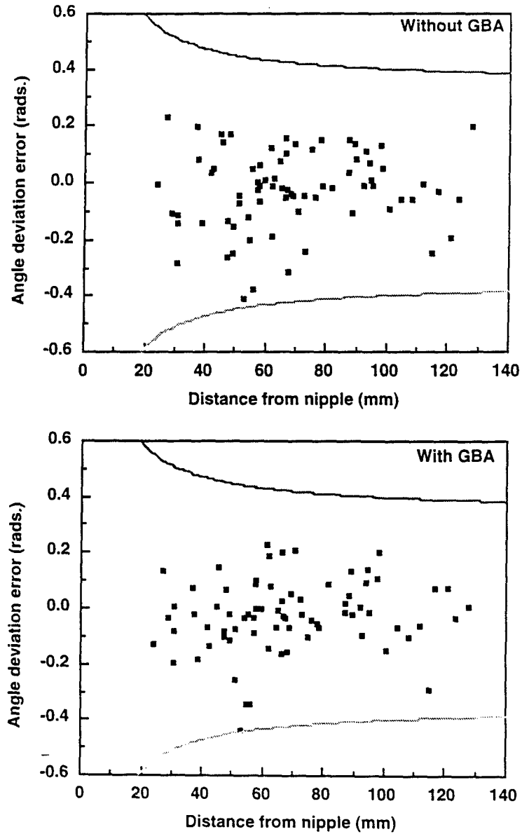
Figure 11. Angular deviation between the initial estimate of the centroid location of the corresponding object and the center of the radiologist-identified object on the previous mammogram with and without GBA. Also shown are the bounding lines defined using \epsilon = 0.35 + 5/r radians.
