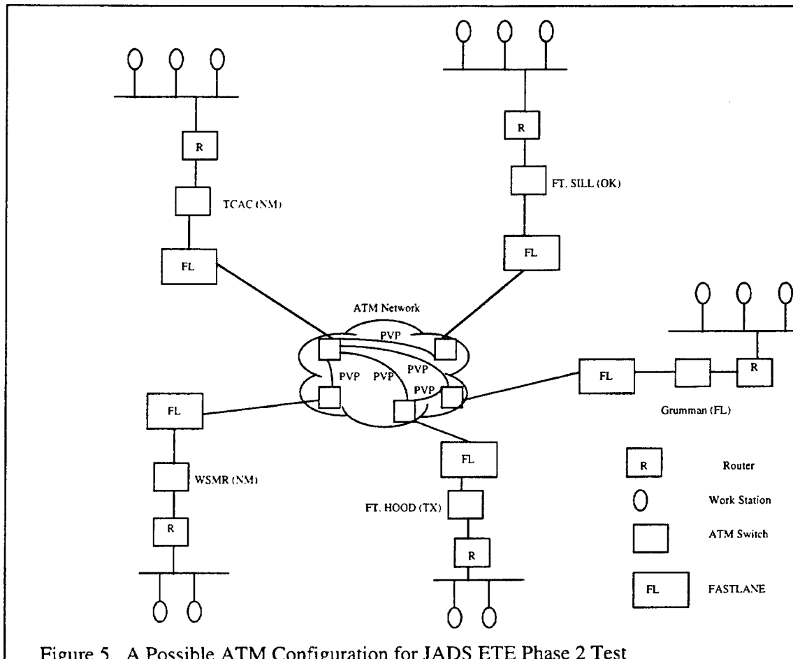
Figure 5. A Possible ATM Configuration for JADS ETE Phase 2 Test
