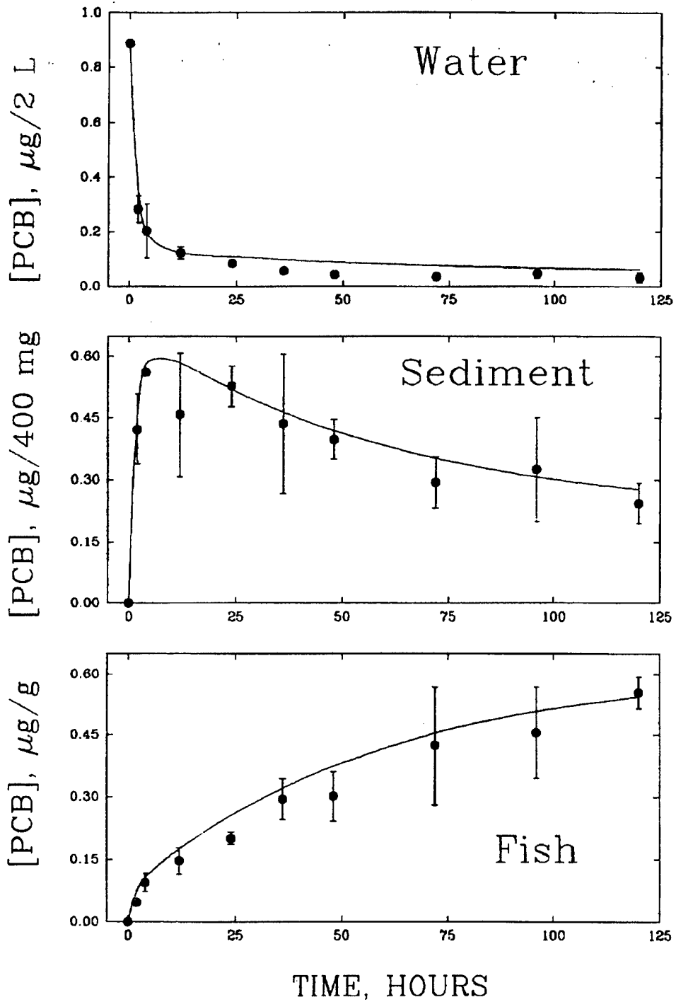
Figure 3. Distribution of PCB-52 among the three compartments — water, sediment, and fish over time; filled circles are means, vertical bars are plus/minus 1 standard deviation; lines are model-fitted estimates from the data
