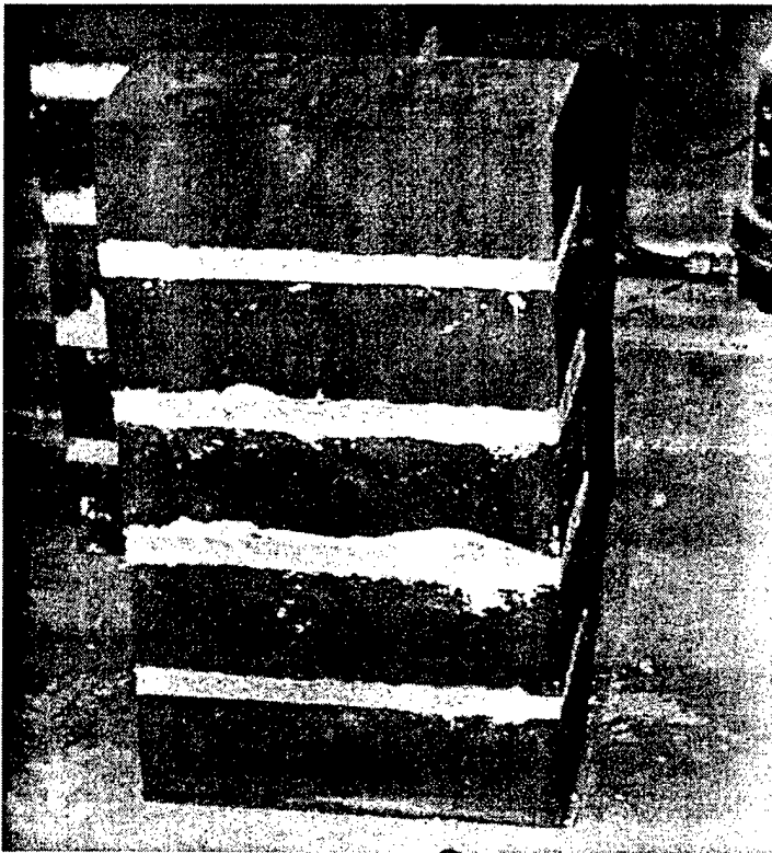
Figure 5. Brick prism.
