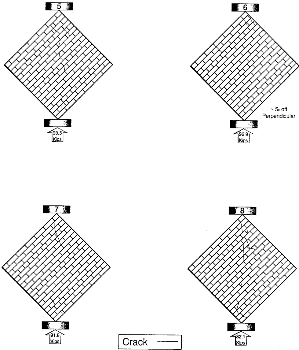
Figure 28. Brick controls.
