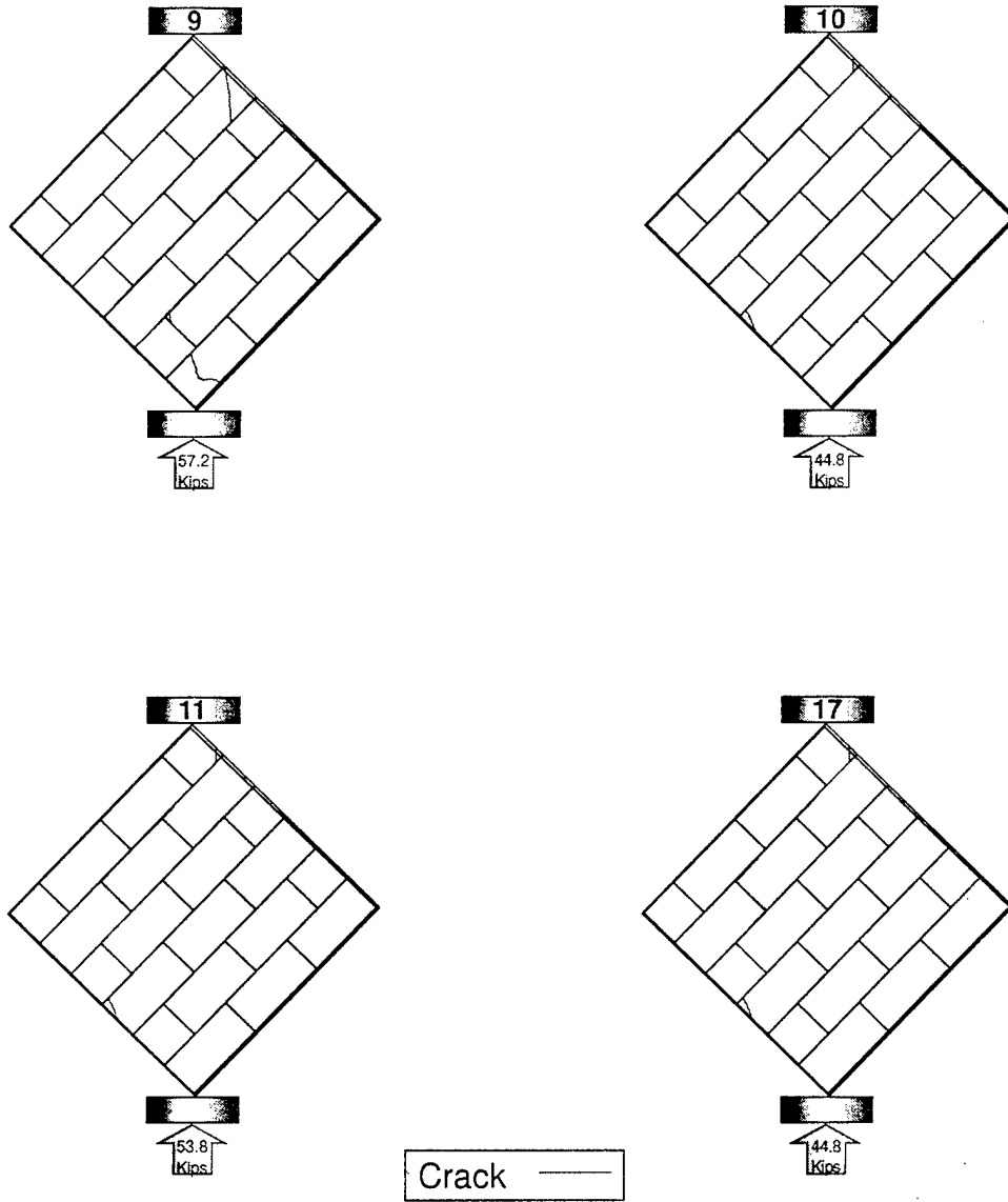
Figure 23. CMU controls.
