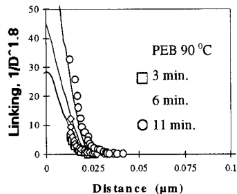
(a) (b) Figure 10. Normalized linewidth data (data points) fit to diffusion reaction kinetics model (solid lines). (a) PEB 105 °C: 1, 3, and 10 min. Reaction order 2.4, Diffusion coefficient 8 nm 2 /s, acid loss rate 0.005%/s. (b) PEB 90 °C: 3, 6, and 11 min. Reaction order 1.8, Diffusion coefficient 0.05 nm 2 /s, acid loss rate 0.0005%/s. [Ref. 36]
