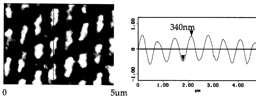
Figure 8: Magnetic force image of a FePt film showing magnetic dots structured, by resistless IPL with 10^{16} He + / cm 2 at 75 keV; The averaged intensity profile demonstrates a dot size of 340 nm.
