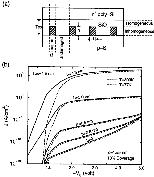
Figure 5: (a) Schematic illustration of an n^+ poly-Si/ \text{SiO}_2 /p-Si tunnel structure with oxide-embedded cylindrical quantum wires. (b) Calculated current density-voltage curves for such structures with various cylinder heights. Quantum wires cover approximately 10% of the cross-sectional area.
