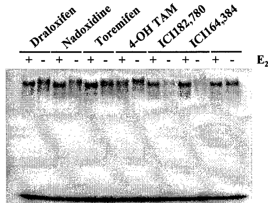
Figure 5. The effect of ligands on ER-ERE gel complex formation.
